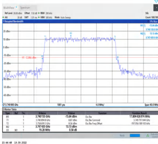
1-N78-3700-3800-30-20-M-4-DFT-64QAM-Outer_Full-50@0-Ant1-17.804-19.280-≤20-PASS
