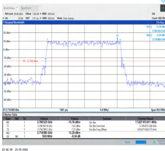
1-N78-3700-3800-30-20-L-5-DFT-256QAM-Outer_Fu II-50@0-Ant1-17.827-18.800-≤20-PASS
