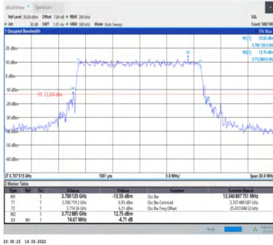
1-N78-3700-3800-30-15-L-6-CP-QPSK-Outer_Full-38@0-Ant1-13.541-14.670-≤15-PASS
