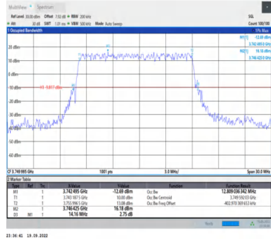
1-N78-3700-3800-30-15-M-2-DFT-PI2BPSK-Outer_Full-36@0-Ant1-12.809-14.160-≤15-PASS
