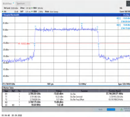
1-N78-3700-3800-30-60-L-2-DFT-PI2BPSK-Outer_Full-162@0-Ant1-57.746-59.640-≤60-PASS
