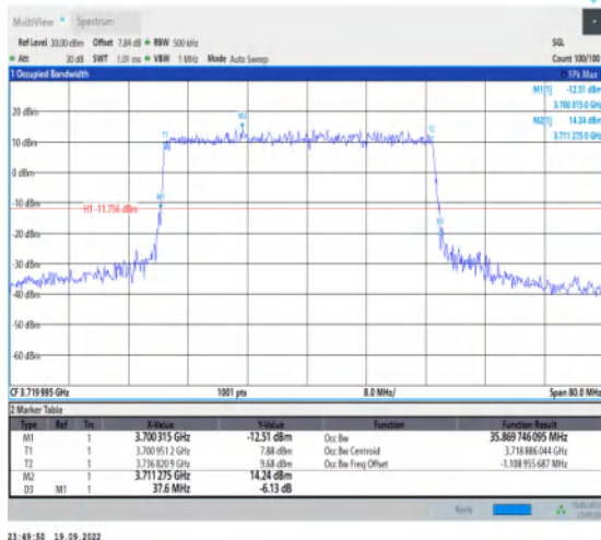
1-N78-3700-3800-30-40-L-4-DFT-64QAM-Outer_Full -100@0-Ant1-35.87-37.600-≤40-PASS
