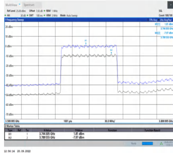
1-N78-3700-3800-30-100-L-2-CP-256QAM-Outer_F ull-273@0-Ant1-9.78-19.56%-7.09-2.69-PASS-≤13
