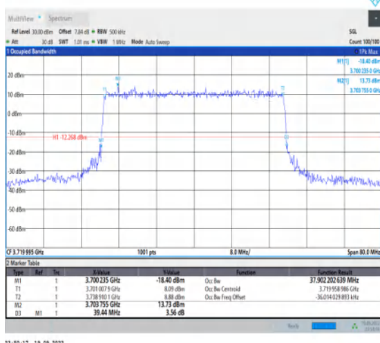
1-N78-3700-3800-30-40-L-6-CP-QPSK-Outer_Full-1 06@0-Ant1-37.902-39.440-≤40-PASS
