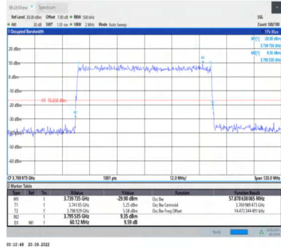
1-N78-3700-3800-30-60-H-5-DFT-256QAM-Outer_F ull-162@0-Ant1-57.879-60.120-≤60-PASS
