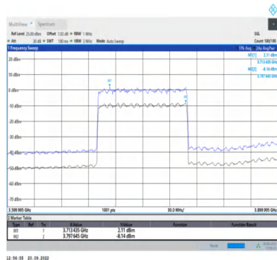
1-N78-3700-3800-30-100-M-2-CP-256QAM-Outer_F ull-273@0-Ant1-10.25-19.56%-7.09-3.16-PASS-≤13
