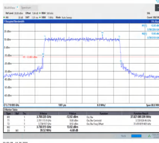
1-N78-3700-3800-30-40-L-7-CP-16QAM-Outer_Full-1 106@0-Ant1-37.821-39.520-≤40-PASS
