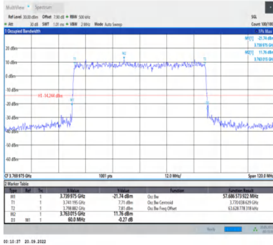
1-N78-3700-3800-30-60-H-4-DFT-64QAM-Outer_Ful I-162@0-Ant1-57.687-60.000-≤60-PASS
