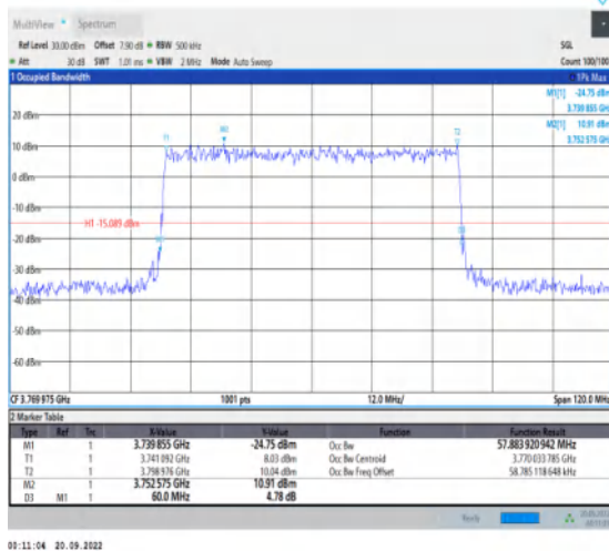
1-N78-3700-3800-30-60-H-6-CP-QPSK-Outer_Full-1 62@0-Ant1-57.884-60.000-≤60-PASS
