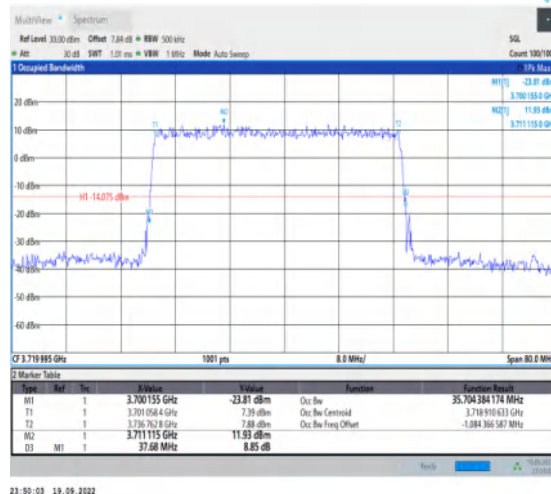
1-N78-3700-3800-30-40-L-5-DFT-256QAM-Outer_Full -100@0-Ant1-35.704-37.680-≤40-PASS
