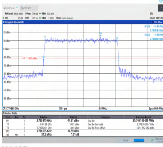
1-N78-3700-3800-30-40-H-4-DFT-64QAM-Outer_Full-100@0-Ant1-35.746-37.200-≤40-PASS
