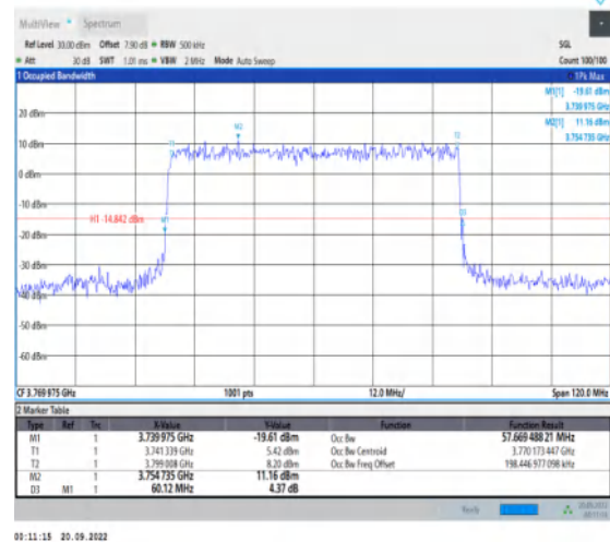
1-N78-3700-3800-30-60-H-7-CP-16QAM-Outer_Full- 162@0-Ant1-57.669-60.120-≤60-PASS
