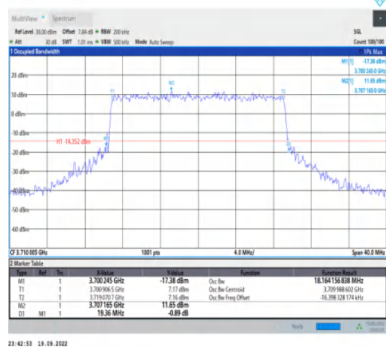
1-N78-3700-3800-30-20-L-6-CP-QPSK-Outer_Full-5 1@0-Ant1-18.164-19.360-≤20-PASS
