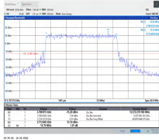
1-N78-3700-3800-30-15-L-7-CP-16QAM-Outer_Full-38@0-Ant1-13.573-14.790-≤15-PASS
