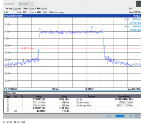
1-N78-3700-3800-30-50-H-4-DFT-64QAM-Outer_Ful I-128@0-Ant1-45.699-47.800-≤50-PASS
