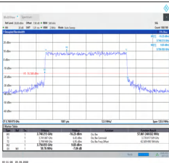
1-N78-3700-3800-30-60-H-8-CP-64QAM-Outer_Full-162@0-Ant1-57.861-59.760-≤60-PASS
