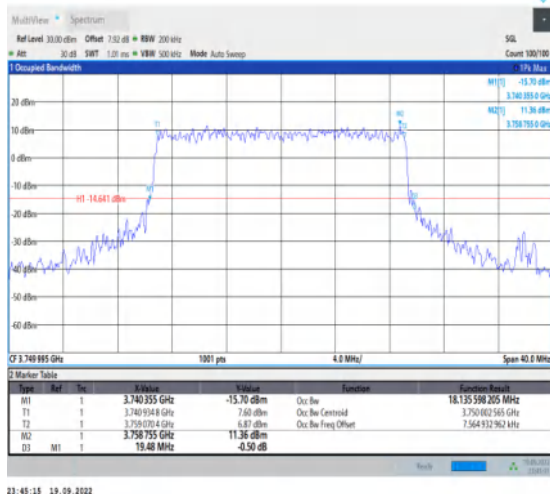
1-N78-3700-3800-30-20-M-6-CP-QPSK-Outet_Full-5 1@0-Ant1-18.136-19.480-≤20-PASS
