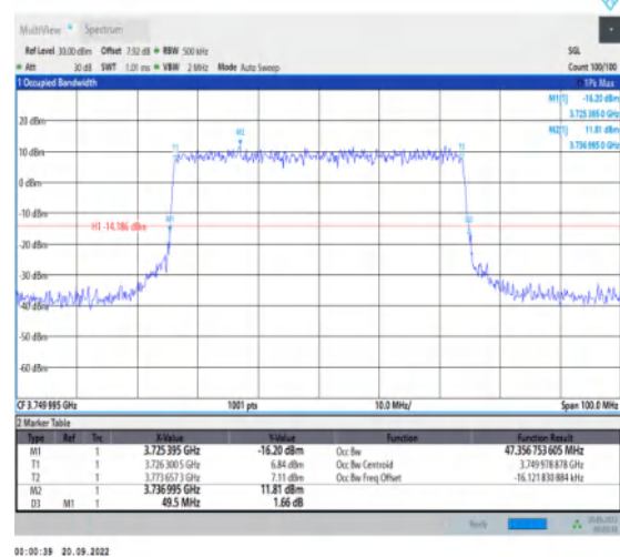
1-N78-3700-3800-30-50-M-7-CP-16QAM-Outer_Full-I-133@0-Ant1-47.357-49.500-≤50-PASS
