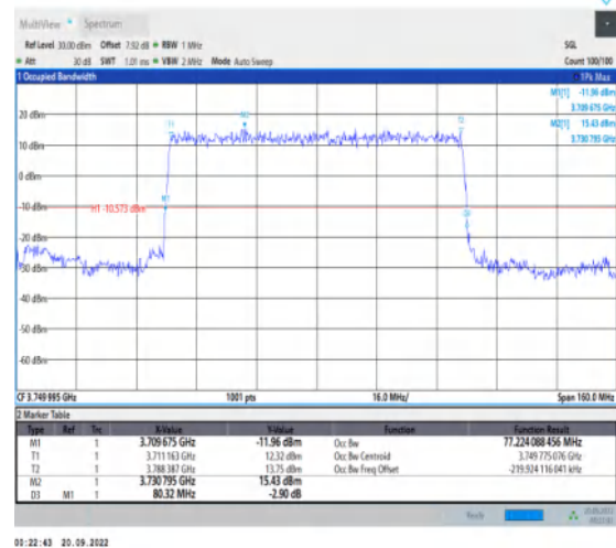
1-N78-3700-3800-30-80-M-2-DFT-PI2BPSK-Outer_Full-216@0-Ant1-77.224-80.320-≤80-PASS
