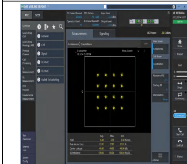
1-N78-3700-3800--30-100-M-7-CP-16QAM-Outer_Full-273@0-Ant1-see graph-PASS
