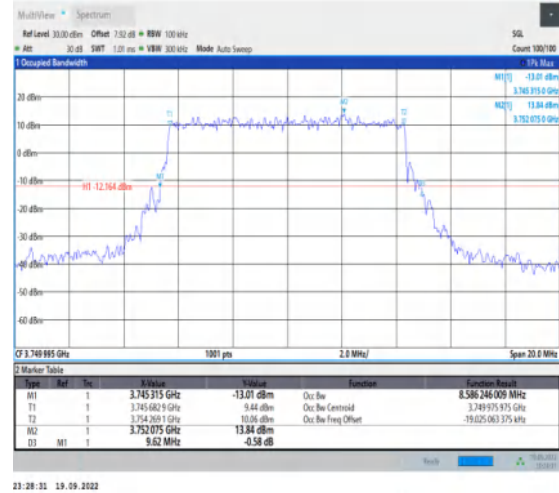
1-N78-3700-3800-30-10-M-1-DFT-QPSK-Outer_Full- 24@0-Ant1-8.586-9.620-≤10-PASS
