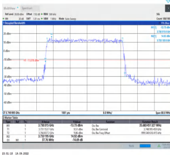
1-N78-3700-3800-30-40-M-1-DFT-QPSK-Outer_Full-100@0-Ant1-35.683-37.760-≤40-PASS
