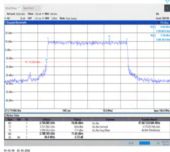
1-N78-3700-3800-30-50-H-6-CP-QPSK-Outer_Full-1 33@0-Ant1-47.467-49.400-≤50-PASS
