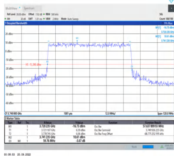
1-N78-3700-3800-30-60-M-8-CP-64QAM-Outer_Full-162@0-Ant1-57.638-59.760-≤60-PASS
