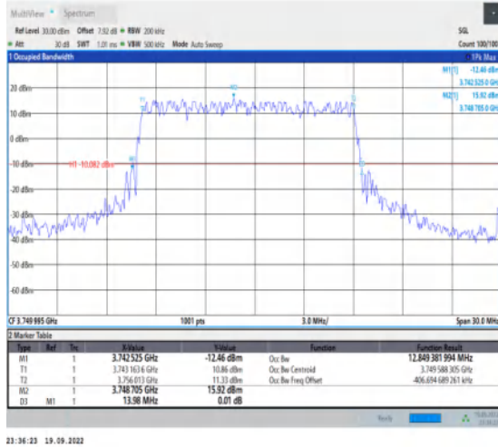
1-N78-3700-3800-30-15-M-1-DFT-QPSK-Outer_Full-36@0-Ant1-12.849-13.980-≤15-PASS
