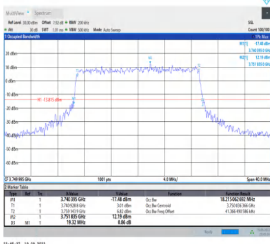
1-N78-3700-3800-30-20-M-8-CP-64QAM-Outet_Full-51@0-Ant1-18.215-19.320-≤20-PASS
