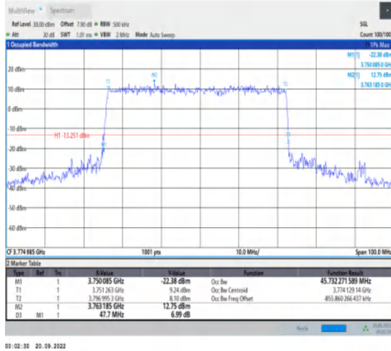
1-N78-3700-3800-30-50-H-3-DFT-16QAM-Outer_Ful I-128@0-Ant1-45.732-47.700-≤50-PASS
