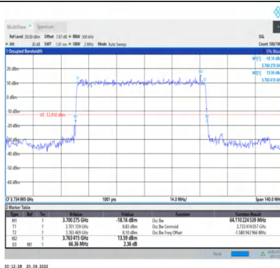
1-N78-3700-3800-30-70-L-2-DFT-PI2BPSK-Outer_Full-180@0-Ant1-64.11-66.360-≤70-PASS
