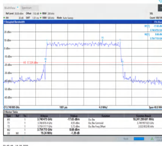
1-N78-3700-3800-30-20-M-9-CP-256QAM-Outet_Full-51@0-Ant1-18.241-19.240-≤20-PASS
