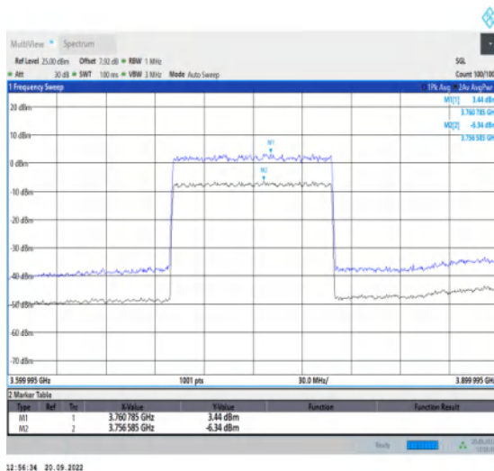
1-N78-3700-3800-30-100-M-1-DFT-256QAM-Outer_F ull-270@0-Ant1-9.78-19.56%-7.09-2.69-PASS-≤13
