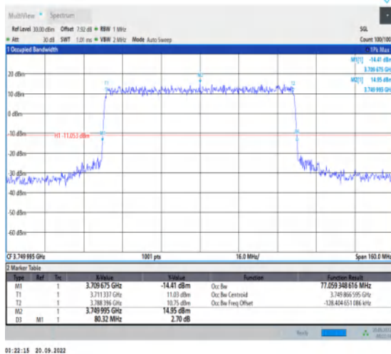
1-N78-3700-3800-30-80-M-1-DFT-QPSK-Outer_Full-216@0-Ant1-77.059-80.320-≤80-PASS
