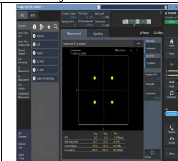
1-N78-3700-3800--30-100-M-6-CP-QPSK-Outer_Full-273@0-Ant1-see graph-PASS
