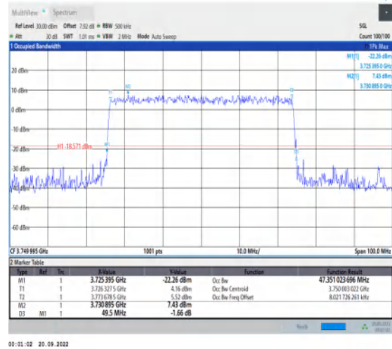
1-N78-3700-3800-30-50-M-9-CP-256QAM-Outer_Fu ll-133@0-Ant1-47.351-49.500-≤50-PASS
