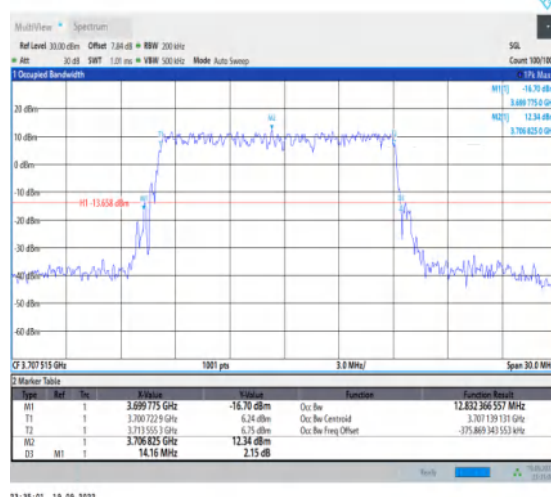
1-N78-3700-3800-30-15-L-5-DFT-256QAM-Outer_Full-36@0-Ant1-12.832-14.160≤15-PASS
