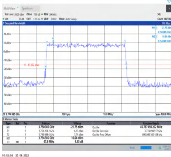
1-N78-3700-3800-30-50-H-5-DFT-256QAM-Outer_F ull-128@0-Ant1-45.787-47.600-≤50-PASS
