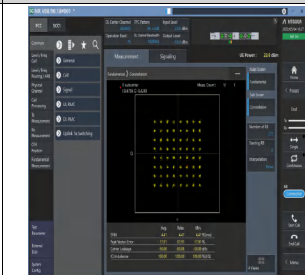
1-N78-3700-3800--30-100-M-8-CP-64QAM-Outer_Full-273@0-Ant1-see graph-PASS
