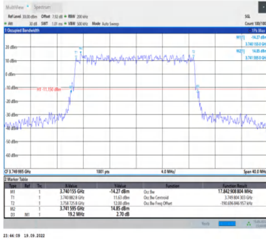
1-N78-3700-3800-30-20-M-2-DFT-PI2BPSK-Outer_Full-50@0-Ant1-17.843-19.200-≤20-PASS
