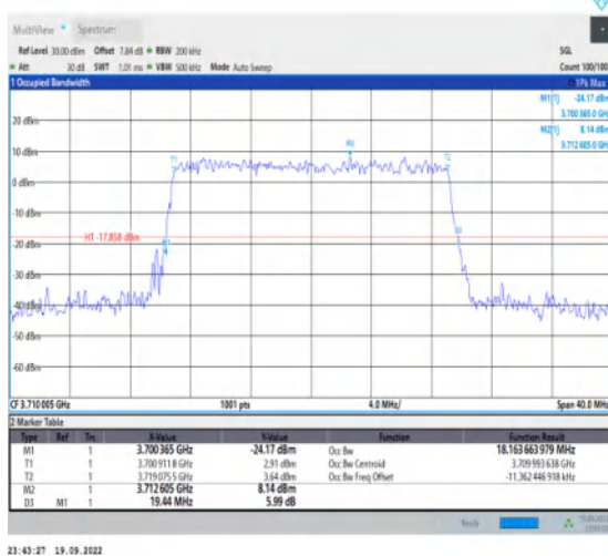
1-N78-3700-3800-30-20-L-9-CP-256QAM-Outer_Full-51@0-Ant1-18.164-19.440-≤20-PASS
