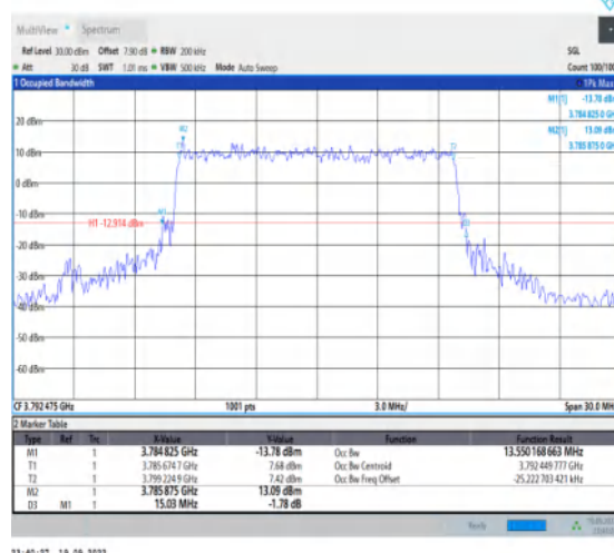
1-N78-3700-3800-30-15-H-7-CP-16QAM-Outer_Full-I-38@0-Ant1-13.55-15.030-≤15-PASS
