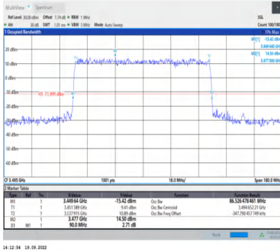
1-N78-3450-3550--30-90-L-1-DFT-QPSK-Outer_Full-243@0-Ant1-86.526-90.000-≤90-PASS
