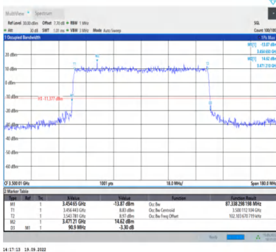
1-N78-3450-3550--30-90-M-6-CP-QPSK-Outer_Full-245@0-Ant1-87.338-90.900-≤90-PASS
