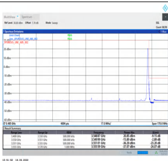
1-N78-3450-3550--30-60-H-2-DFT-PI2BPSK-Edge_1R B_Right-1@161-Ant1-1--PASS-see graph
