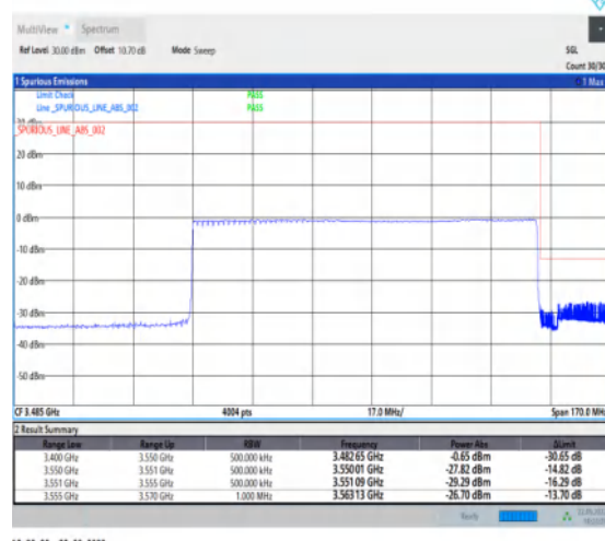
1-N78-3450-3550-PC2-30-100-H-6-CP-QPSK-Out er_Full-273@0-Ant1-1--PASS-see graph
