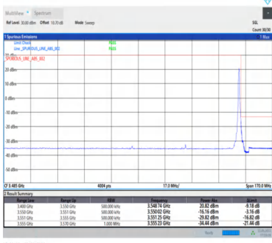
1-N78-3450-3550-PC2-30-70-H-5-CP-QPSK-Edge_1R B_Right-1@188-Ant1-1--PASS-see graph
