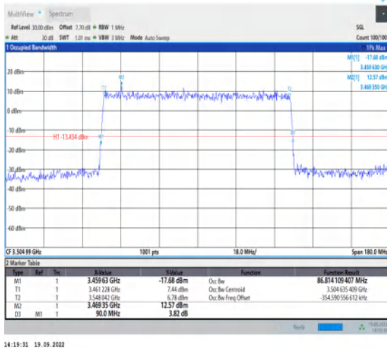
1-N78-3450-3550--30-90-H-5-DFT-256QAM-Outer_F ull-243@0-Ant1-86.814-90.000-≤90-PASS
