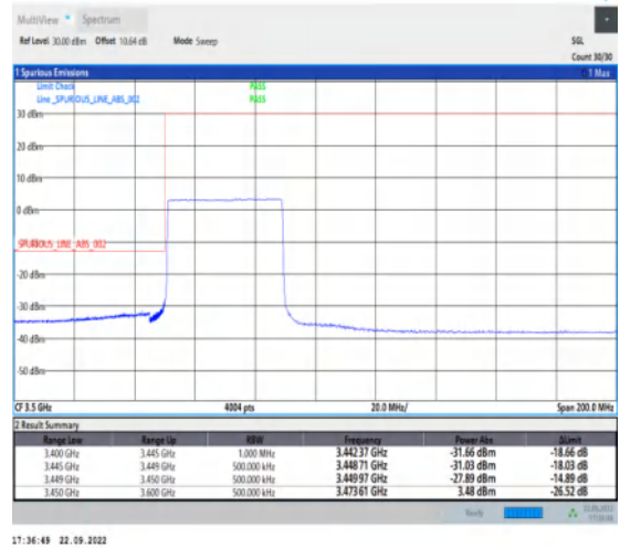
1-N78-3450-3550-PC2-30-40-L-6-CP-QPSK-Outer _Full-106@0-Ant1-1--PASS-see graph
