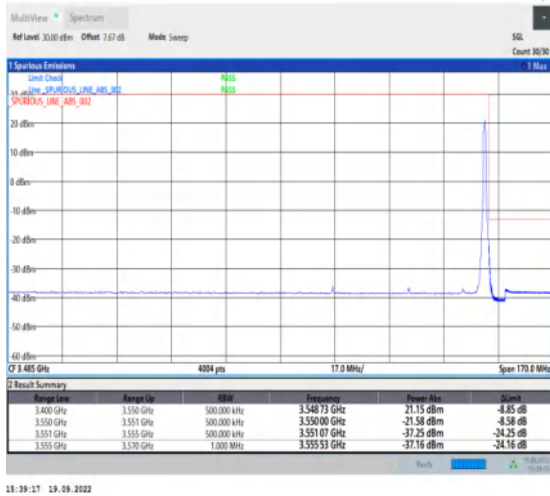
1-N78-3450-3550--30-50-H-2-DFT-PI2BPSK-Edge_1R B_Right-1@132-Ant1-1--PASS-see graph
