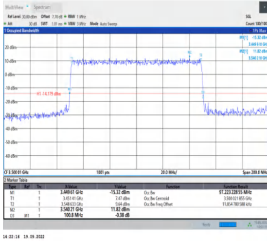
1-N78-3450-3550--30-100-L-6-CP-QPSK-Outer_Full -273@0-Ant1-97.223-100.800≤100-PASS
