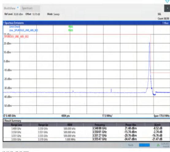
1-N78-3450-3550-PC2-30-80-H-5-CP-QPSK-Edge_1R B_Right-1@216-Ant1-1--PASS-see graph
