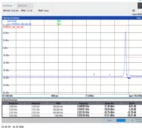
1-N78-3450-3550--30-40-H-5-CP-QPSK-Edge_1RB_R ight-1@105-Ant1-1--PASS-see graph
