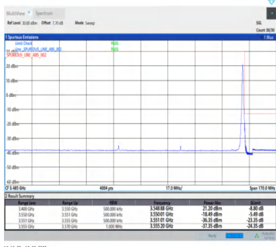
1-N78-3450-3550--30-80-H-5-CP-QPSK-Edge_1RB_R ight-1@216-Ant1-1--PASS-see graph
