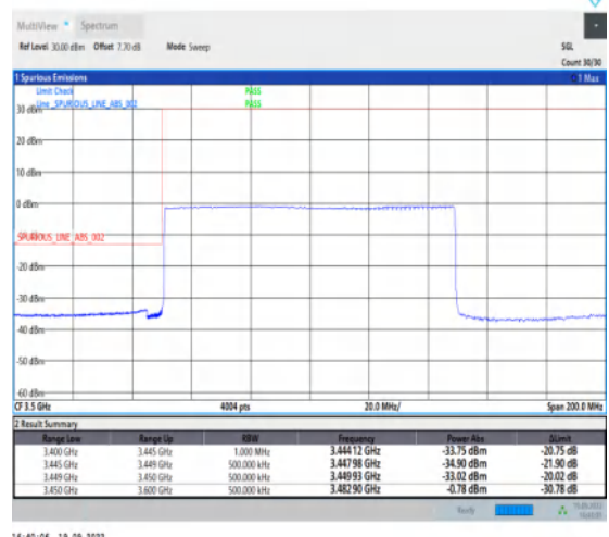
1-N78-3450-3550--30-100-L-6-CP-QPSK-Outer_Full-273@0-Ant1-1--PASS-see graph
