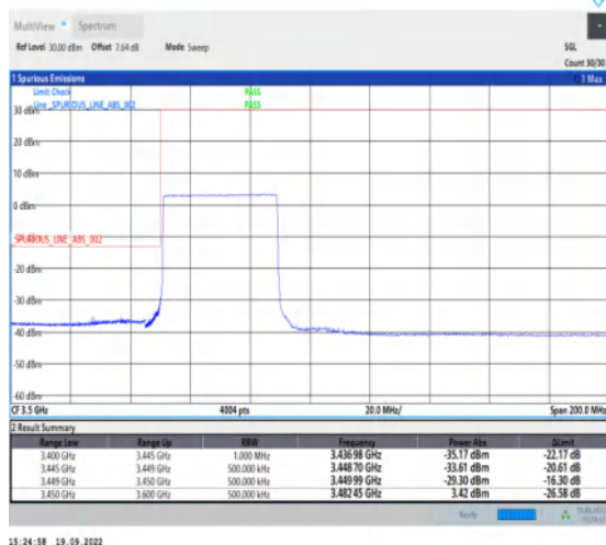
1-N78-3450-3550--30-40-L-6-CP-QPSK-Outer_Ful l-106@0-Ant1-1--PASS-see graph
