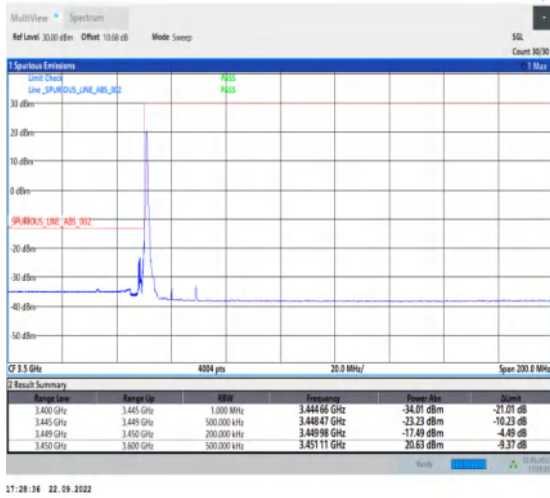
1-N78-3450-3550-PC2-30-20-L-4-CP-QPSK-Edge_1R_B_Left-1@0-Ant1-1--PASS-see graph
