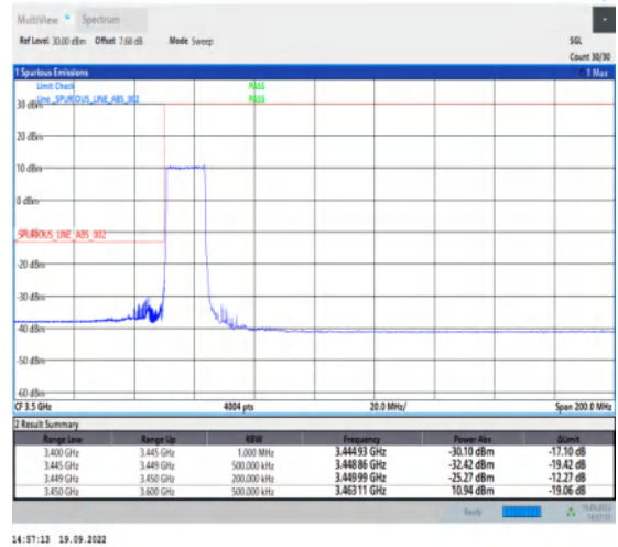
1-N78-3450-3550--30-15-L-3-DFT-PI2BPSK-Outer_Full-36@0-Ant1-1--PASS-see graph
