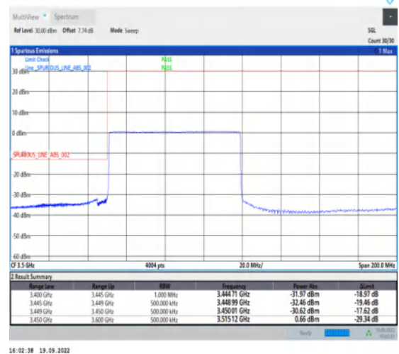
1-N78-3450-3550--30-70-L-6-CP-QPSK-Outer_Ful l-189@0-Ant1-1--PASS-see graph
