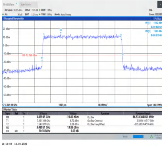
1-N78-3450-3550--30-90-H-3-DFT-16QAM-Outer_Fu II-243@0-Ant1-86.533-90.180-≤90-PASS
