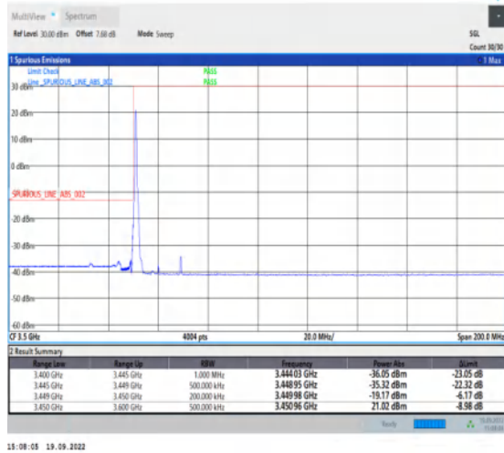
1-N78-3450-3550--30-20-L-1-DFT-PI2BPSK-Edge_1R_B_Left-1@0-Ant1-1--PASS-see graph
