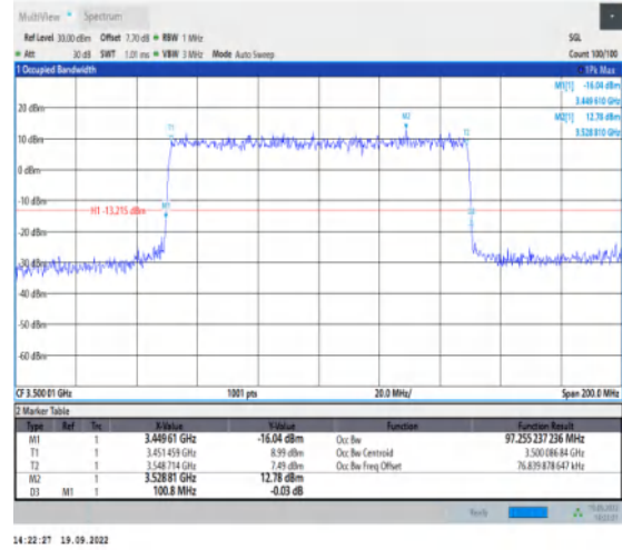
1-N78-3450-3550--30-100-L-7-CP-16QAM-Outer_Fu II-273@0-Ant1-97.255-100.800≤100-PASS
