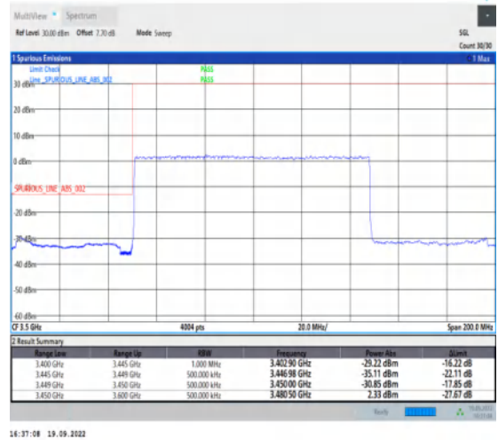
1-N78-3450-3550--30-100-L-3-DFT-PI2BPSK-Outer_Full-270@0-Ant1-1--PASS-see graph
