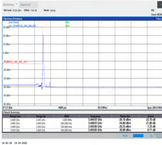
1-N78-3450-3550--30-10-L-1-DFT-PI2BPSK-Edge_1R_B_Left-1@0-Ant1-1--PASS-see graph
