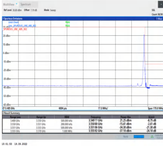
1-N78-3450-3550--30-15-H-2-DFT-PI2BPSK-Edge_1R_B_Right-1@37-Ant1-1--PASS-see graph
