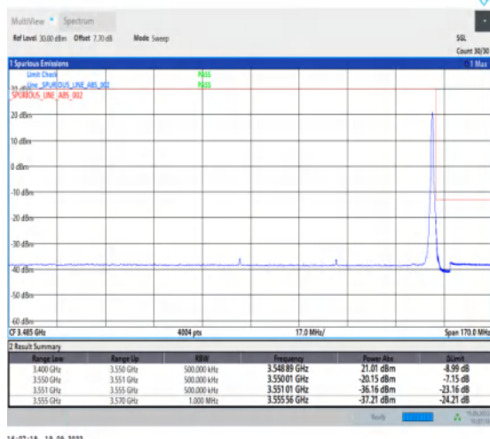
1-N78-3450-3550--30-70-H-5-CP-QPSK-Edge_1RB_R ight-1@188-Ant1-1--PASS-see graph
