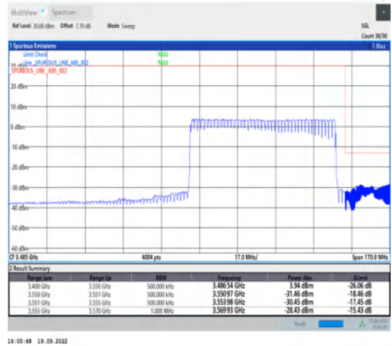
1-N78-3450-3550--30-70-H-3-DFT-PI2BPSK-Outer _Full-180@0-Ant1-1--PASS-see graph
