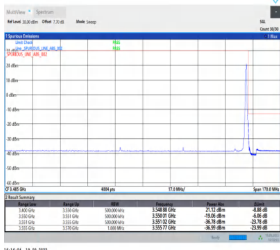
1-N78-3450-3550--30-80-H-2-DFT-PI2BPSK-Edge_1R B_Right-1@216-Ant1-1--PASS-see graph
