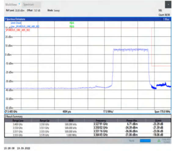
1-N78-3450-3550--30-40-H-3-DFT-PI2BPSK-Outer _Full-100@0-Ant1-1--PASS-see graph
