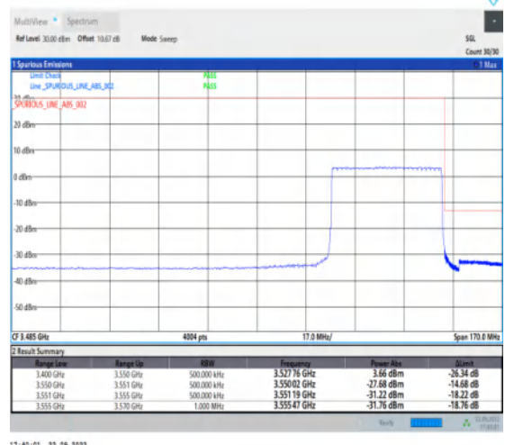
1-N78-3450-3550-PC2-30-40-H-6-CP-QPSK-Outer _Full-106@0-Ant1-1--PASS-see graph
