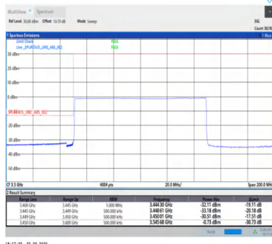
1-N78-3450-3550-PC2-30-100-L-6-CP-QPSK-Out er_Full-273@0-Ant1-1--PASS-see graph
