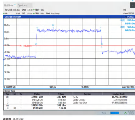
1-N78-3450-3550--30-90-H-2-DFT-PI2BPSK-Outer_Full Full-243@0-Ant1-86.78-89.820≤90-PASS
