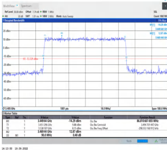
1-N78-3450-3550--30-90-L-3-DFT-16QAM-Outer_Full-243@0-Ant1-86.811-90.000-≤90-PASS
