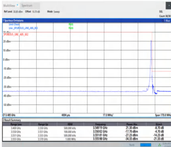
1-N78-3450-3550-PC2-30-10-H-5-CP-QPSK-Edge_1R B_Right-1@23-Ant1-1--PASS-see graph
