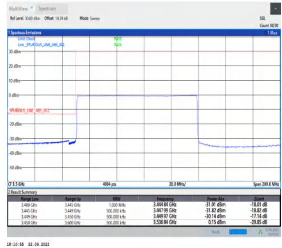
1-N78-3450-3550-PC2-30-90-L-6-CP-QPSK-Outer _Full-245@0-Ant1-1--PASS-see graph
