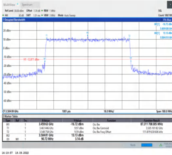
1-N78-3450-3550--30-90-H-7-CP-16QAM-Outer_Full -245@0-Ant1-87.312-90.720≤90-PASS
