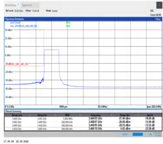
1-N78-3450-3550-PC2-30-20-L-6-CP-QPSK-Outer_Full-51@0-Ant1-1--PASS-see graph
