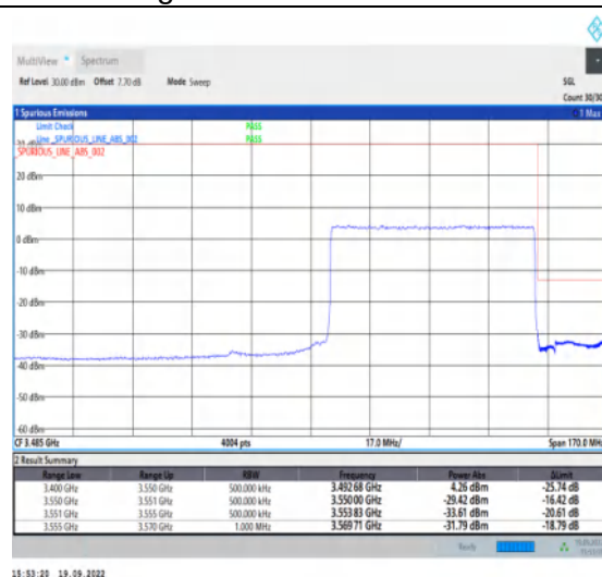
1-N78-3450-3550--30-60-H-3-DFT-PI2BPSK-Outer _Full-162@0-Ant1-1--PASS-see graph
