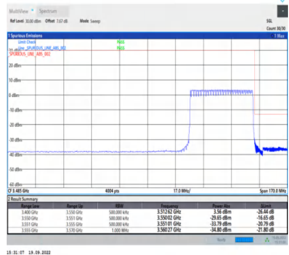
1-N78-3450-3550--30-40-H-6-CP-QPSK-Outer_Ful l-106@0-Ant1-1--PASS-see graph
