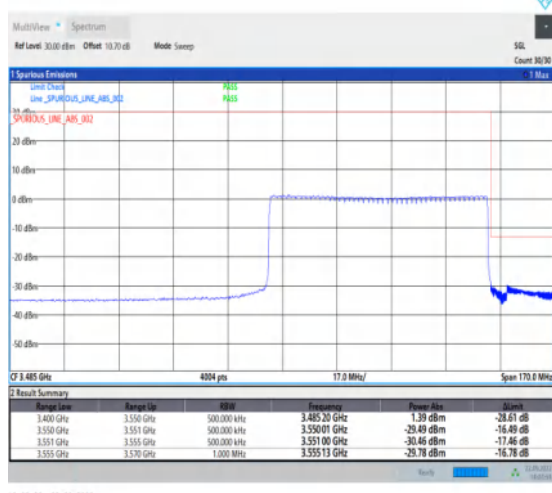
1-N78-3450-3550-PC2-30-70-H-6-CP-QPSK-Outer _Full-189@0-Ant1-1--PASS-see graph
