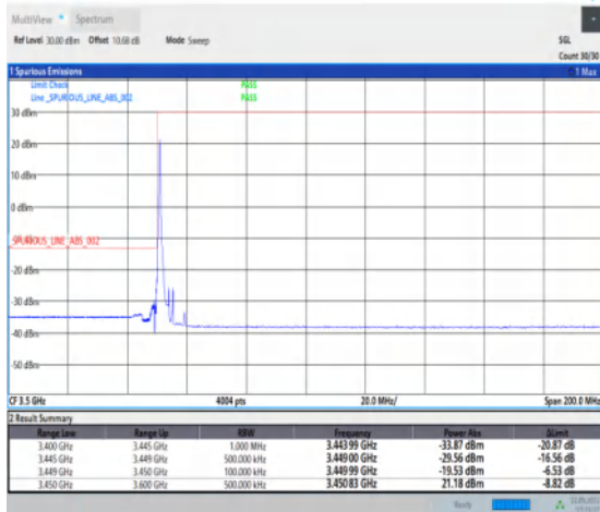
1-N78-3450-3550-PC2-30-10-L-4-CP-QPSK-Edge_1R B_Left-1@0-Ant1-1--PASS-see graph
