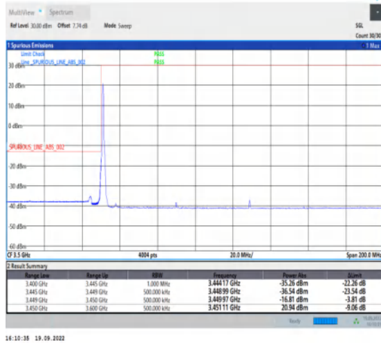
1-N78-3450-3550--30-80-L-1-DFT-PI2BPSK-Edge_1R_B_Left-1@0-Ant1-1--PASS-see graph
