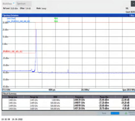
1-N78-3450-3550--30-50-L-1-DFT-PI2BPSK-Edge_1R_B_Left-1@0-Ant1-1--PASS-see graph
