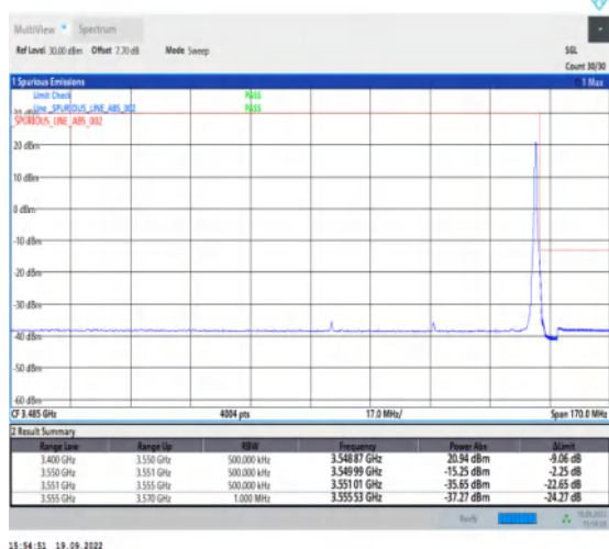
1-N78-3450-3550--30-60-H-5-CP-QPSK-Edge_1RB_R ight-1@161-Ant1-1--PASS-see graph
