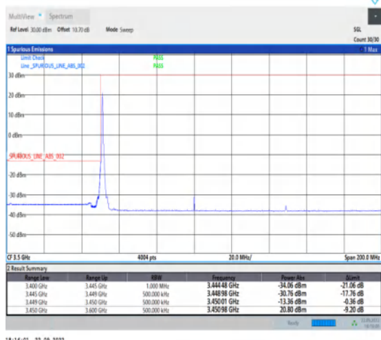
1-N78-3450-3550-PC2-30-100-L-4-CP-QPSK-Edge_1 RB_Left-1@0-Ant1-1--PASS-see graph
