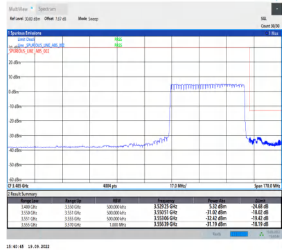
1-N78-3450-3550--30-50-H-3-DFT-PI2BPSK-Outer _Full-128@0-Ant1-1--PASS-see graph
