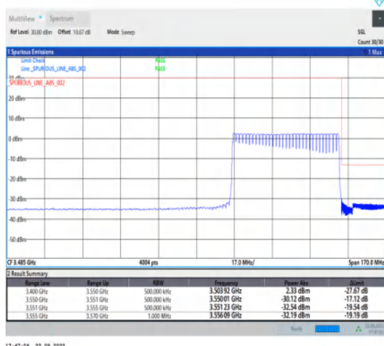
1-N78-3450-3550-PC2-30-50-H-6-CP-QPSK-Outer _Full-133@0-Ant1-1--PASS-see graph
