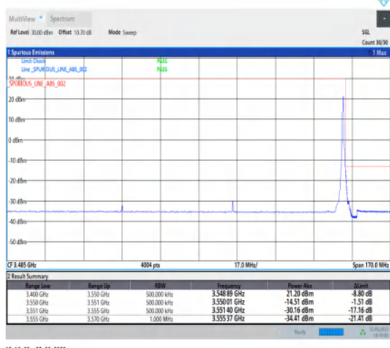
1-N78-3450-3550-PC2-30-100-H-5-CP-QPSK-Edge_1 RB_Right-1@272-Ant1-1--PASS-see graph
