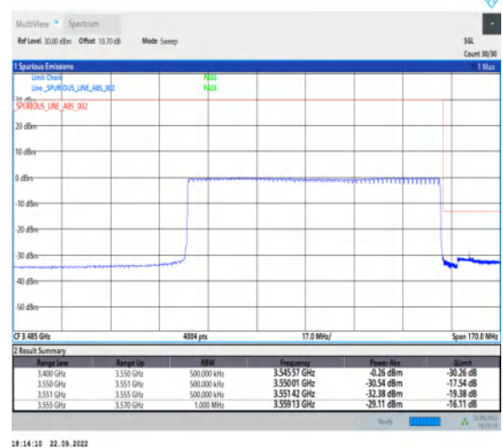
1-N78-3450-3550-PC2-30-90-H-6-CP-QPSK-Outer _Full-245@0-Ant1-1--PASS-see graph
