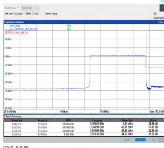
1-N78-3450-3550--30-60-H-6-CP-QPSK-Outer_Ful l-162@0-Ant1-1--PASS-see graph
