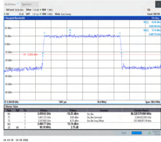
1-N78-3450-3550--30-90-H-4-DFT-64QAM-Outer_Fu II-243@0-Ant1-86.521-90.180-≤90-PASS
