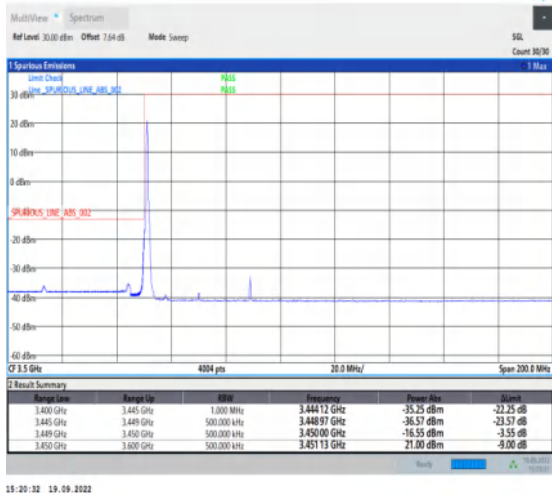
1-N78-3450-3550--30-40-L-1-DFT-PI2BPSK-Edge_1R_B_Left-1@0-Ant1-1--PASS-see graph
