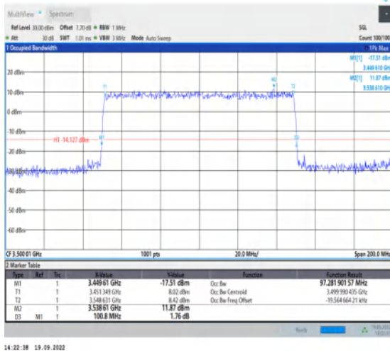
1-N78-3450-3550--30-100-L-8-CP-64QAM-Outer_Fu II-273@0-Ant1-97.282-100.800≤100-PASS
