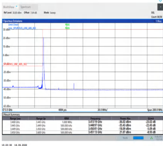
1-N78-3450-3550--30-40-L-4-CP-QPSK-Edge_1RB_L eft-1@0-Ant1-1--PASS-see graph
