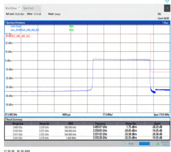
1-N78-3450-3550-PC2-30-60-H-6-CP-QPSK-Outer _Full-162@0-Ant1-1--PASS-see graph
