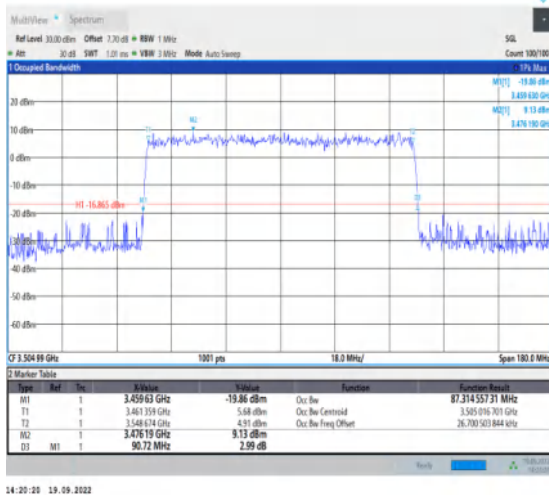
1-N78-3450-3550--30-90-H-9-CP-256QAM-Outer_Full -245@0-Ant1-87.315-90.720≤90-PASS
