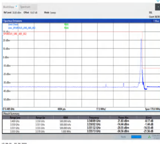
1-N78-3450-3550-PC2-30-40-H-5-CP-QPSK-Edge_1R B_Right-1@105-Ant1-1--PASS-see graph
