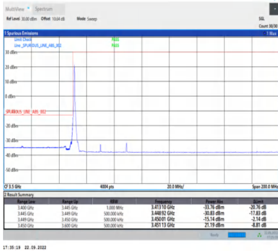
1-N78-3450-3550-PC2-30-40-L-4-CP-QPSK-Edge_1R B_Left-1@0-Ant1-1--PASS-see graph
