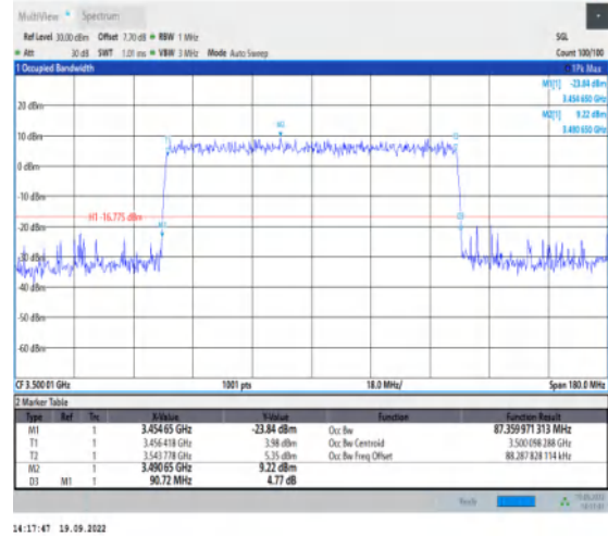
1-N78-3450-3550--30-90-M-9-CP-256QAM-Outer_Full I-245@0-Ant1-87.36-90.720≤90-PASS
