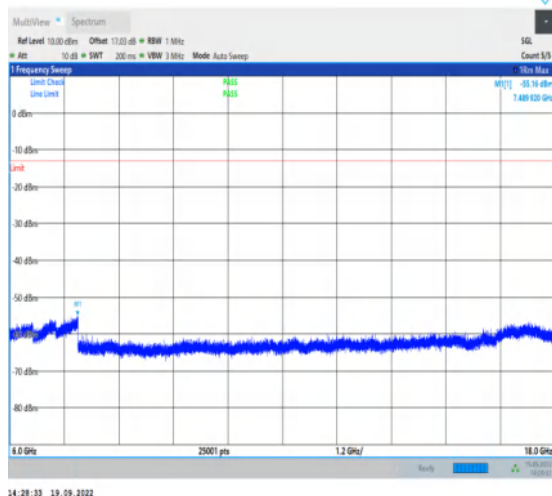
1-N78-3450-3550--30-100-L-1-DFT-PI2BPSK-Inner_1RB_Left-1@1-6000-18000-Ant1-7489.92--55.16--1 3-PASS
