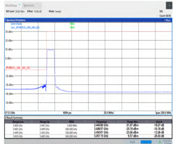
1-N78-3450-3550-PC2-30-10-L-6-CP-QPSK-Outer _Full-24@0-Ant1-1--PASS-see graph
