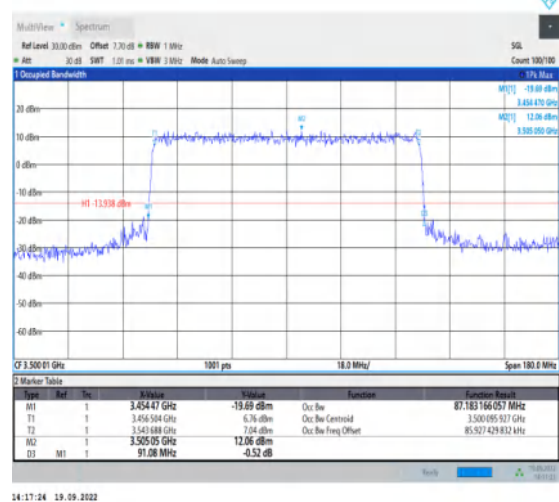
1-N78-3450-3550--30-90-M-7-CP-16QAM-Outer_Full-245@0-Ant1-87.183-91.080-≤90-PASS
