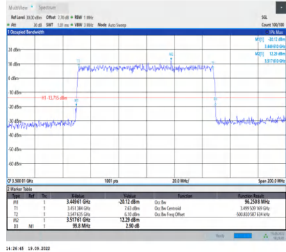
1-N78-3450-3550--30-100-H-5-DFT-256QAM-Outer_Full-270@0-Ant1-96.251-99.800-≤100-PASS
