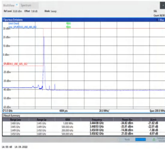
1-N78-3450-3550--30-15-L-1-DFT-PI2BPSK-Edge_1R_B_Left-1@0-Ant1-1--PASS-see graph
