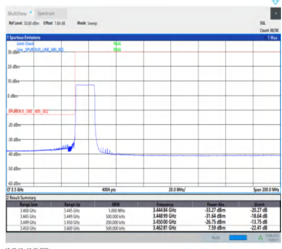
1-N78-3450-3550--30-15-L-6-CP-QPSK-Outer_Ful l-38@0-Ant1-1--PASS-see graph
