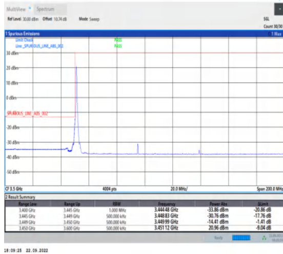
1-N78-3450-3550-PC2-30-90-L-4-CP-QPSK-Edge_1R B_Left-1@0-Ant1-1--PASS-see graph
