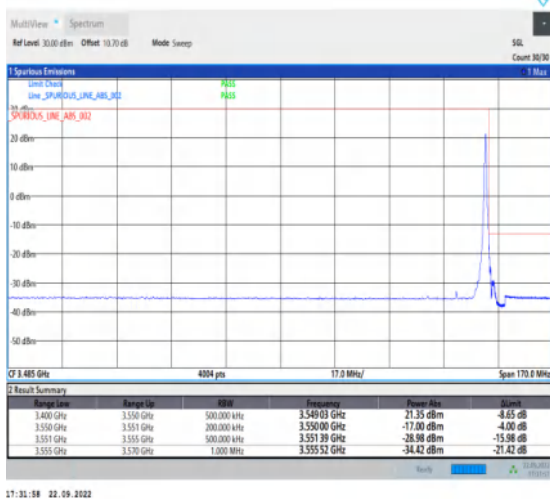
1-N78-3450-3550-PC2-30-20-H-5-CP-QPSK-Edge_1R_B_Right-1@50-Ant1-1--PASS-see graph
