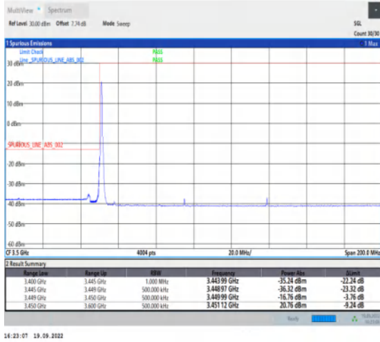
1-N78-3450-3550--30-90-L-1-DFT-PI2BPSK-Edge_1R_B_Left-1@0-Ant1-1--PASS-see graph
