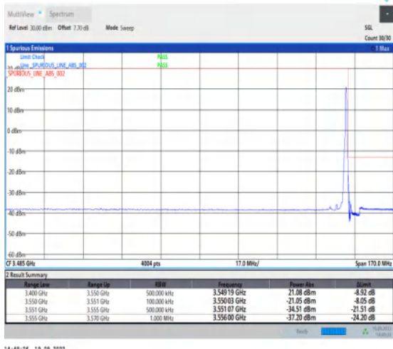
1-N78-3450-3550--30-10-H-2-DFT-PI2BPSK-Edge_1R B_Right-1@23-Ant1-1--PASS-see graph
