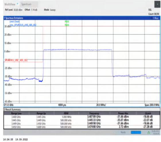
1-N78-3450-3550--30-90-L-3-DFT-PI2BPSK-Outer_Full-243@0-Ant1-1--PASS-see graph
