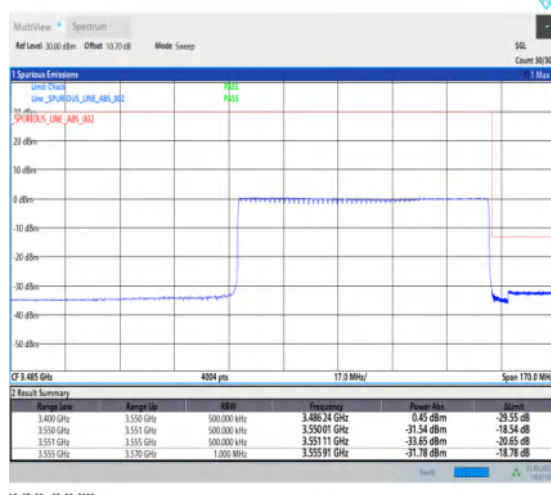
1-N78-3450-3550-PC2-30-80-H-6-CP-QPSK-Outer _Full-217@0-Ant1-1--PASS-see graph
