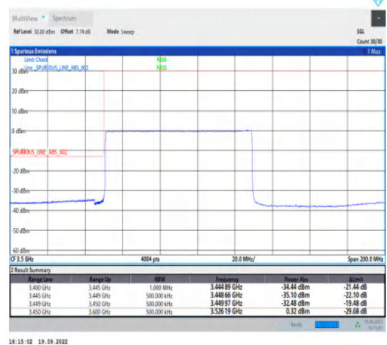
1-N78-3450-3550--30-80-L-6-CP-QPSK-Outer_Ful l-217@0-Ant1-1--PASS-see graph
