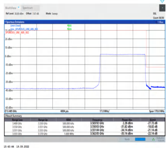
1-N78-3450-3550--30-50-H-6-CP-QPSK-Outer_Ful l-133@0-Ant1-1--PASS-see graph
