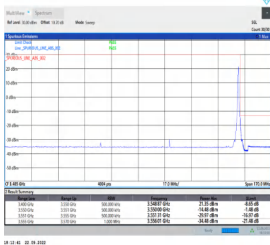
1-N78-3450-3550-PC2-30-90-H-5-CP-QPSK-Edge_1R B_Right-1@244-Ant1-1--PASS-see graph
