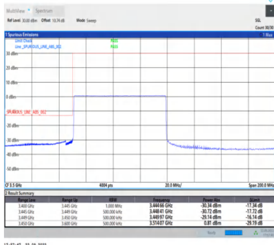
1-N78-3450-3550-PC2-30-70-L-6-CP-QPSK-Outer _Full-189@0-Ant1-1--PASS-see graph
