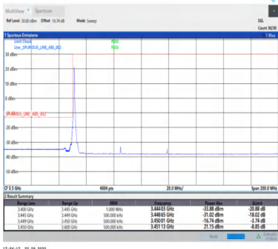
1-N78-3450-3550-PC2-30-70-L-4-CP-QPSK-Edge_1R B_Left-1@0-Ant1-1--PASS-see graph
