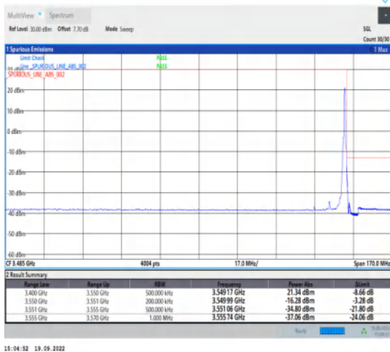
1-N78-3450-3550--30-15-H-5-CP-QPSK-Edge_1RB_R ight-1@37-Ant1-1--PASS-see graph
