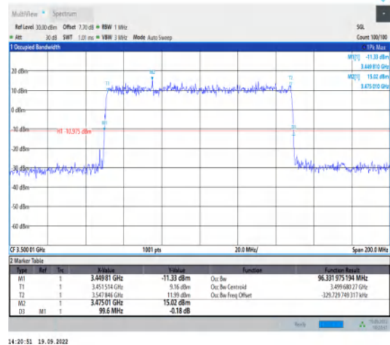
1-N78-3450-3550--30-100-L-1-DFT-QPSK-Outer_Full -270@0-Ant1-96.332-99.600≤100-PASS
