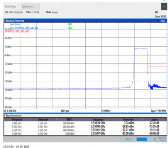
1-N78-3450-3550--30-15-H-6-CP-QPSK-Outer_Ful l-38@0-Ant1-1--PASS-see graph
