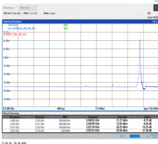
1-N78-3450-3550-PC2-30-60-H-5-CP-QPSK-Edge_1R B_Right-1@161-Ant1-1--PASS-see graph
