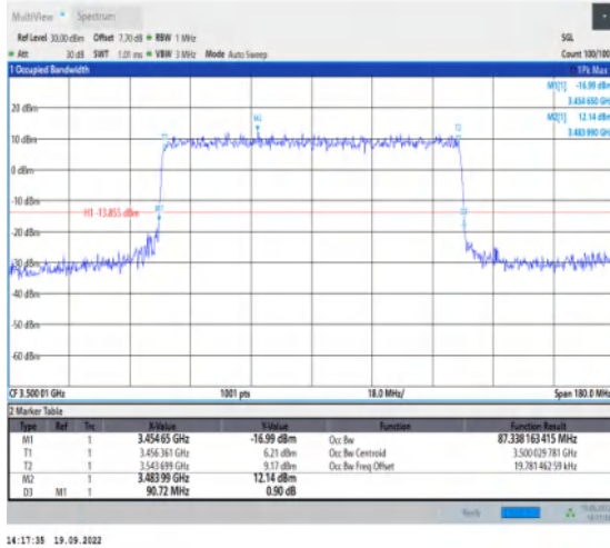
1-N78-3450-3550--30-90-M-8-CP-64QAM-Outer_Full I-245@0-Ant1-87.338-90.720≤90-PASS
