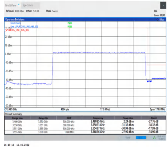
1-N78-3450-3550--30-100-H-3-DFT-PI2BPSK-Out er_Full-270@0-Ant1-1--PASS-see graph
