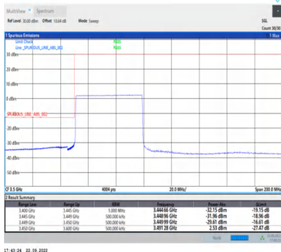
1-N78-3450-3550-PC2-30-50-L-6-CP-QPSK-Outer _Full-133@0-Ant1-1--PASS-see graph
