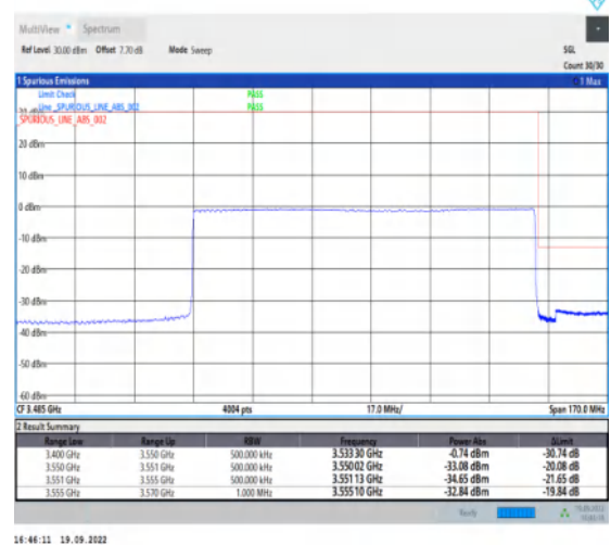
1-N78-3450-3550--30-100-H-6-CP-QPSK-Outer_F ull-273@0-Ant1-1--PASS-see graph
