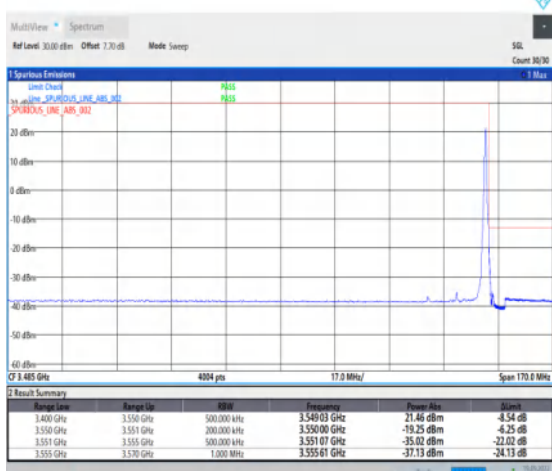
1-N78-3450-3550--30-20-H-5-CP-QPSK-Edge_1RB_R_ight-1@50-Ant1-1--PASS-see graph
