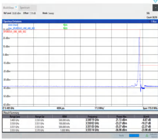
1-N78-3450-3550--30-10-H-5-CP-QPSK-Edge_1RB_R ight-1@23-Ant1-1--PASS-see graph
