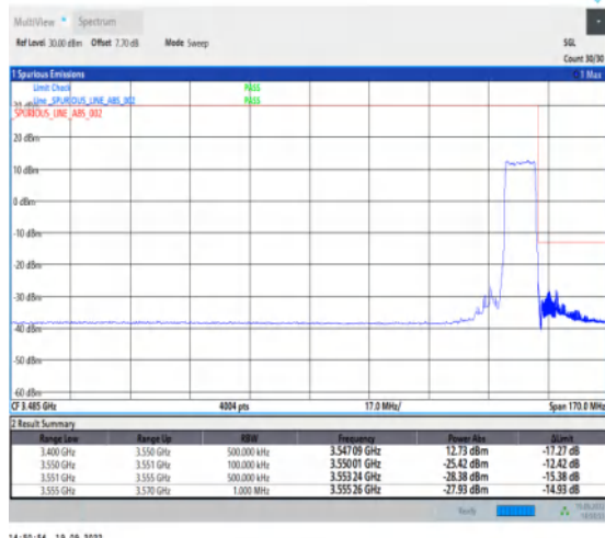
1-N78-3450-3550--30-10-H-3-DFT-PI2BPSK-Outer _Full-24@0-Ant1-1--PASS-see graph
