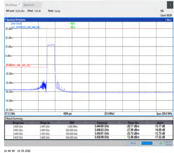
1-N78-3450-3550--30-10-L-3-DFT-PI2BPSK-Outer_Full-24@0-Ant1-1--PASS-see graph
