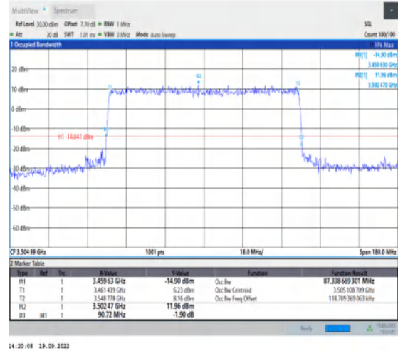
1-N78-3450-3550--30-90-H-8-CP-64QAM-Outer_Full -245@0-Ant1-87.339-90.720≤90-PASS
