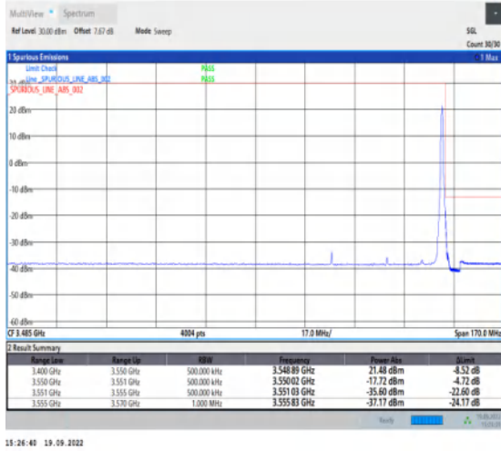
1-N78-3450-3550--30-40-H-2-DFT-PI2BPSK-Edge_1R B_Right-1@105-Ant1-1--PASS-see graph
