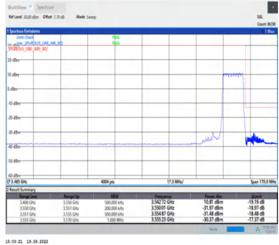
1-N78-3450-3550--30-15-H-3-DFT-PI2BPSK-Outer_Full-36@0-Ant1-1--PASS-see graph
