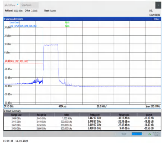
1-N78-3450-3550--30-20-L-3-DFT-PI2BPSK-Outer_Full-50@0-Ant1-1--PASS-see graph
