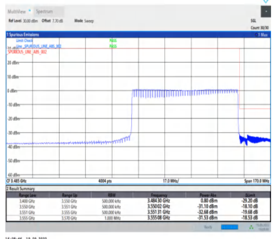
1-N78-3450-3550--30-70-H-6-CP-QPSK-Outer_Ful l-189@0-Ant1-1--PASS-see graph
