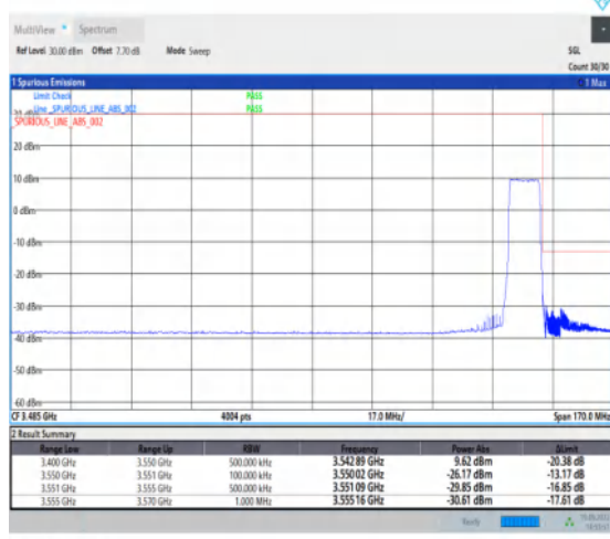
1-N78-3450-3550--30-10-H-6-CP-QPSK-Outer_Ful l-24@0-Ant1-1--PASS-see graph
