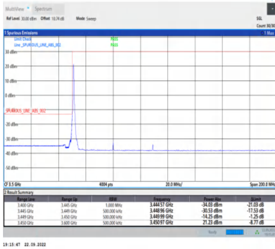
1-N78-3450-3550-PC2-30-60-L-4-CP-QPSK-Edge_1R B_Left-1@0-Ant1-1--PASS-see graph
