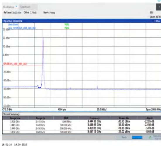
1-N78-3450-3550--30-70-L-4-CP-QPSK-Edge_1RB_L eft-1@0-Ant1-1--PASS-see graph
