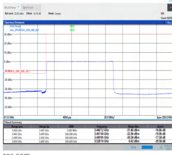
1-N78-3450-3550-PC2-30-80-L-6-CP-QPSK-Outer _Full-217@0-Ant1-1--PASS-see graph
