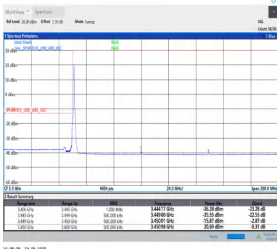
1-N78-3450-3550--30-100-L-4-CP-QPSK-Edge_1RB_Left-1@0-Ant1-1--PASS-see graph
