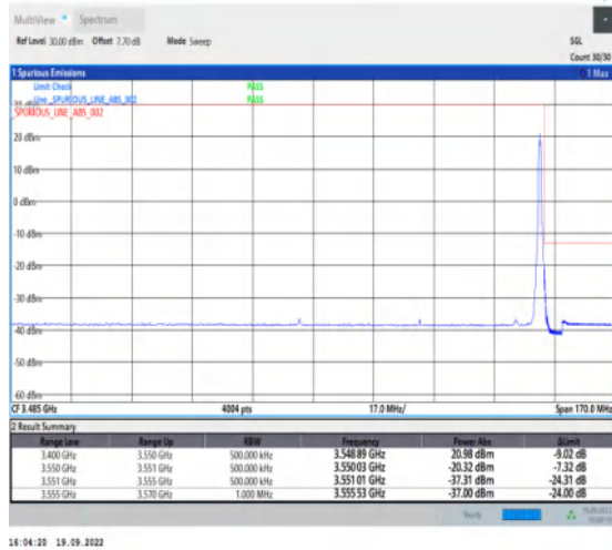
1-N78-3450-3550--30-70-H-2-DFT-PI2BPSK-Edge_1R B_Right-1@188-Ant1-1--PASS-see graph
