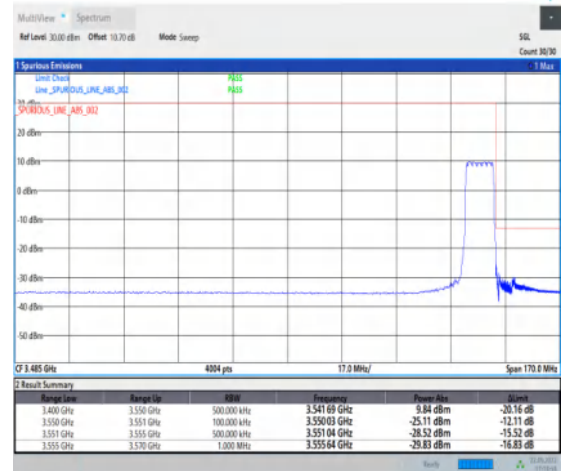
1-N78-3450-3550-PC2-30-10-H-6-CP-QPSK-Outer _Full-24@0-Ant1-1--PASS-see graph
