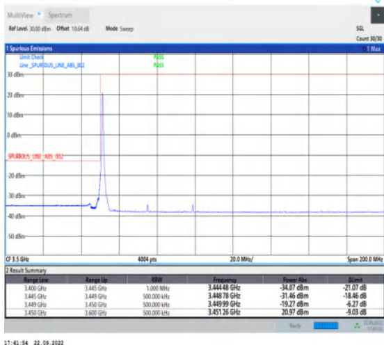
1-N78-3450-3550-PC2-30-50-L-4-CP-QPSK-Edge_1R B_Left-1@0-Ant1-1--PASS-see graph
