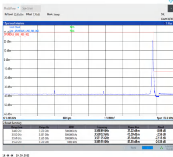
1-N78-3450-3550--30-100-H-5-CP-QPSK-Edge_1RB_ Right-1@272-Ant1-1--PASS-see graph
