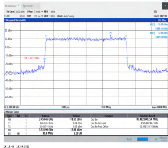
1-N78-3450-3550--30-90-H-6-CP-QPSK-Outer_Full- 245@0-Ant1-87.483-90.900-≤90-PASS
