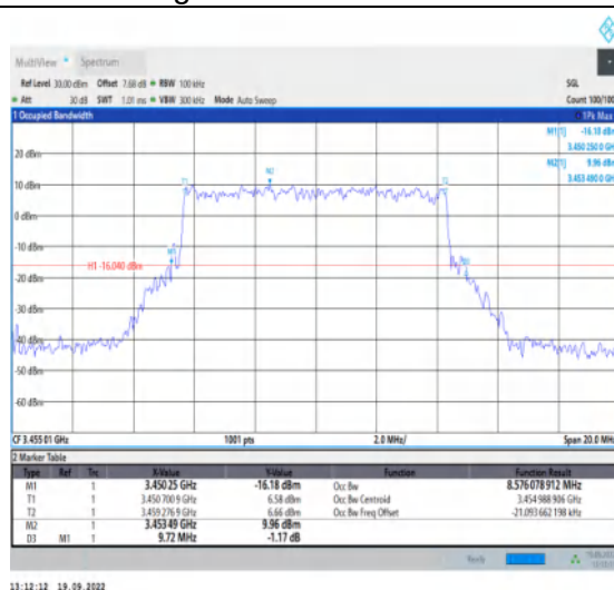
1-N78-3450-3550--30-10-L-6-CP-QPSK-Outer_Full-2 4@0-Ant1-8.576-9.720-≤10-PASS
