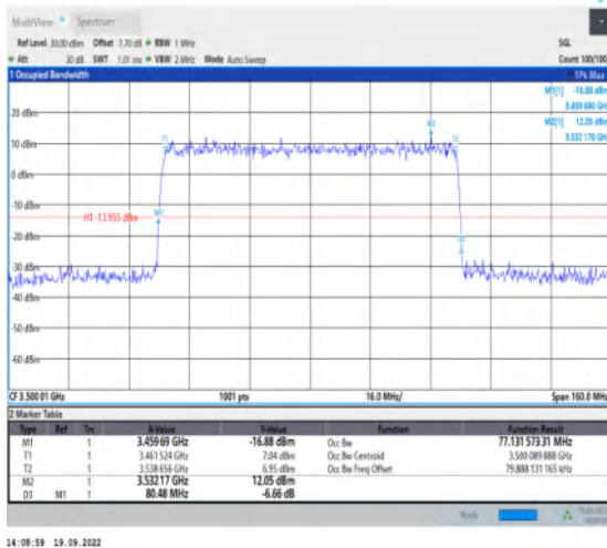
1-N78-3450-3550--30-80-M-5-DFT-256QAM-Outer_Full-216@0-Ant1-77.132-80.480-≤80-PASS
