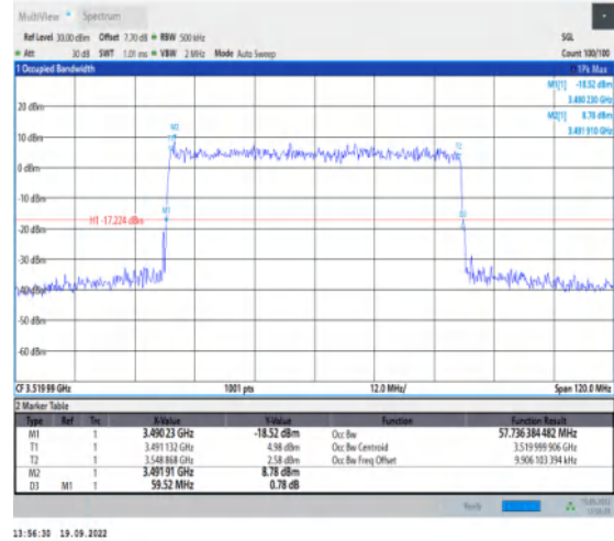
1-N78-3450-3550--30-60-H-9-CP-256QAM-Outer_Fu ll-162@0-Ant1-57.736-59.520-≤60-PASS
