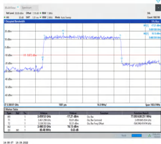
1-N78-3450-3550--30-80-M-2-DFT-PI2BPSK-Outer_Full Full-216@0-Ant1-77.094-80.480-≤80-PASS
