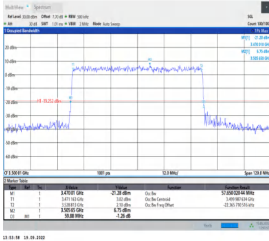
1-N78-3450-3550--30-60-M-9-CP-256QAM-Outer_Full-162@0-Ant1-57.65-59.880-≤60-PASS
