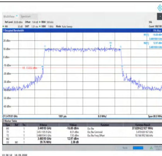
1-N78-3450-3550--30-40-L-8-CP-64QAM-Outer_Full -106@0-Ant1-37.829-39.760-≤40-PASS
