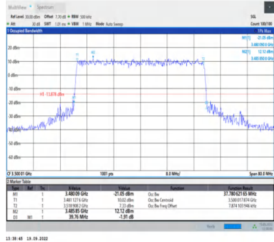
1-N78-3450-3550--30-40-M-8-CP-64QAM-Outer_Full -106@0-Ant1-37.781-39.760≤40-PASS
