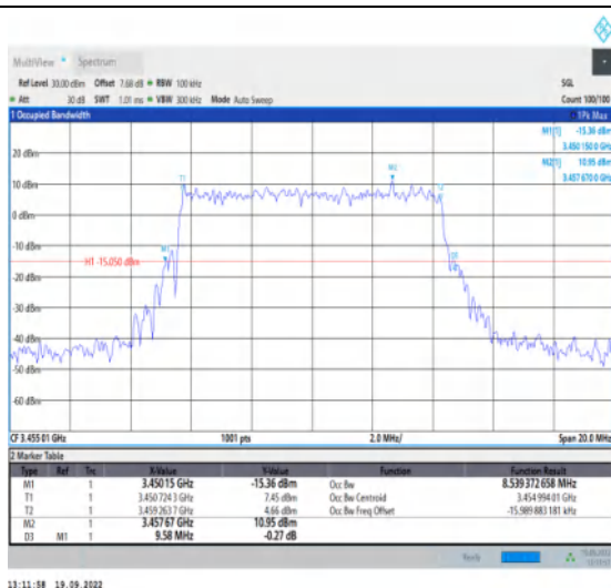
1-N78-3450-3550--30-10-L-5-DFT-256QAM-Outer_F ull-24@0-Ant1-8.539-9.580-≤10-PASS
