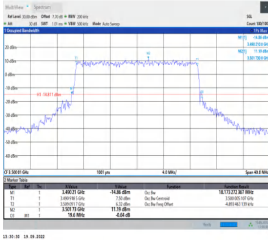
1-N78-3450-3550--30-20-M-6-CP-QPSK-Outer_Full-51@0-Ant1-18.173-19.600-≤20-PASS
