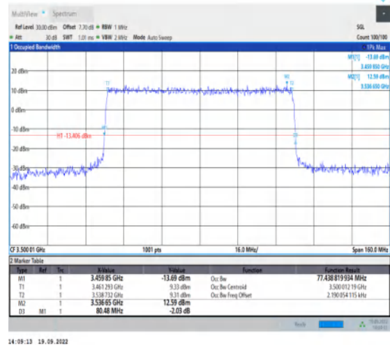
1-N78-3450-3550--30-80-M-6-CP-QPSK-Outer_Full-217@0-Ant1-77.439-80.480-≤80-PASS
