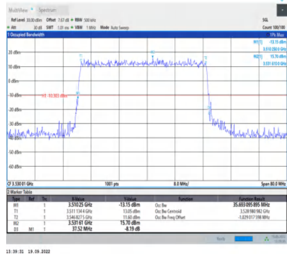
1-N78-3450-3550--30-40-H-1-DFT-QPSK-Outer_Full -100@0-Ant1-35.693-37.520≤40-PASS
