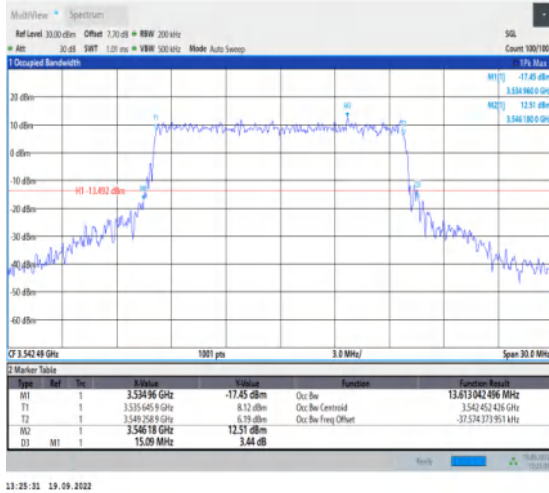
1-N78-3450-3550--30-15-H-8-CP-64QAM-Outer_Full -38@0-Ant1-13.613-15.090≤15-PASS
