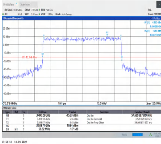
1-N78-3450-3550--30-60-H-8-CP-64QAM-Outer_Full -162@0-Ant1-57.69-59.520-≤60-PASS
