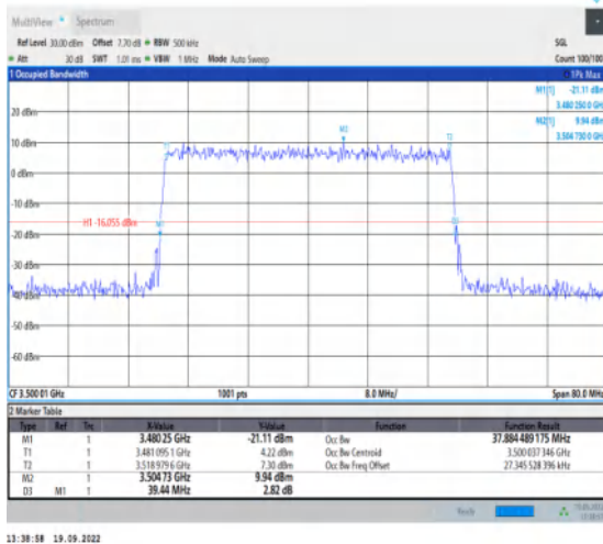
1-N78-3450-3550--30-40-M-9-CP-256QAM-Outer_Full ull-106@0-Ant1-37.884-39.440≤40-PASS
