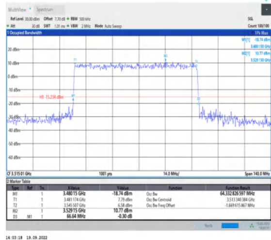
1-N78-3450-3550--30-70-H-4-DFT-64QAM-Outer_Fu -180@0-Ant1-64.333-66.640-≤70-PASS
