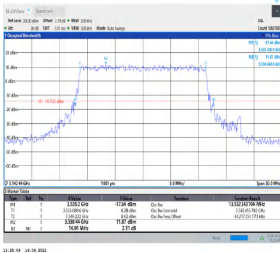
1-N78-3450-3550--30-15-H-6-CP-QPSK-Outer_Full-38@0-Ant1-13.532-14.910-≤15-PASS
