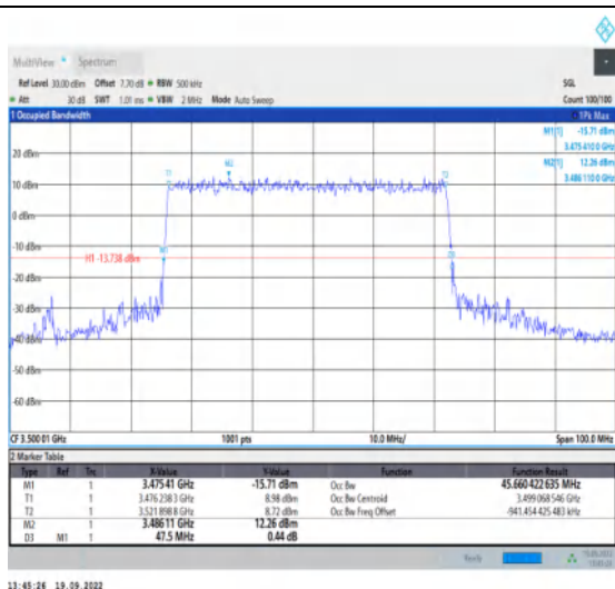
1-N78-3450-3550--30-50-M-4-DFT-64QAM-Outer_Full-128@0-Ant1-45.66-47.500-≤50-PASS
