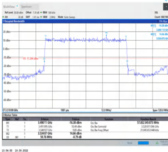
1-N78-3450-3550--30-60-H-2-DFT-PI2BPSK-Outer_Full-162@0-Ant1-57.832-59.760-≤60-PASS
