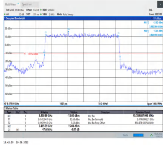
1-N78-3450-3550--30-50-L-2-DFT-PI2BPSK-Outer_Full-128@0-Ant1-45.79-47.600-≤50-PASS
