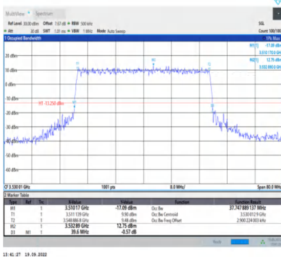
1-N78-3450-3550--30-40-H-8-CP-64QAM-Outet_Full-106@0-Ant1-37.748-39.600-≤40-PASS
