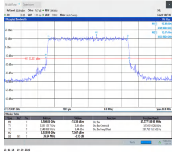
1-N78-3450-3550--30-40-H-7-CP-16QAM-Outet_Full-106@0-Ant1-37.777-39.840-≤40-PASS
