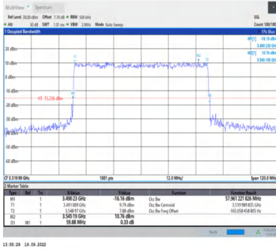
1-N78-3450-3550--30-60-H-4-DFT-64QAM-Outer_Fu II-162@0-Ant1-57.961-59.880-≤60-PASS
