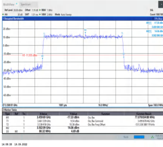
1-N78-3450-3550--30-80-M-3-DFT-16QAM-Outer_Full-216@0-Ant1-77.079-80.320-≤80-PASS
