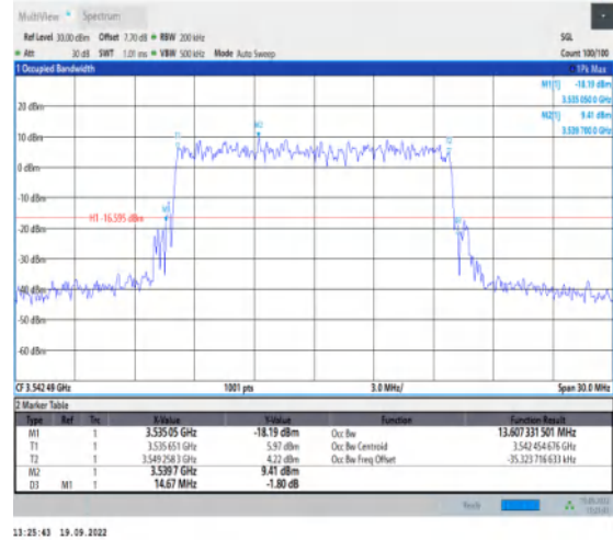
1-N78-3450-3550--30-15-H-9-CP-256QAM-Outer_Fu ll-38@0-Ant1-13.607-14.670≤15-PASS
