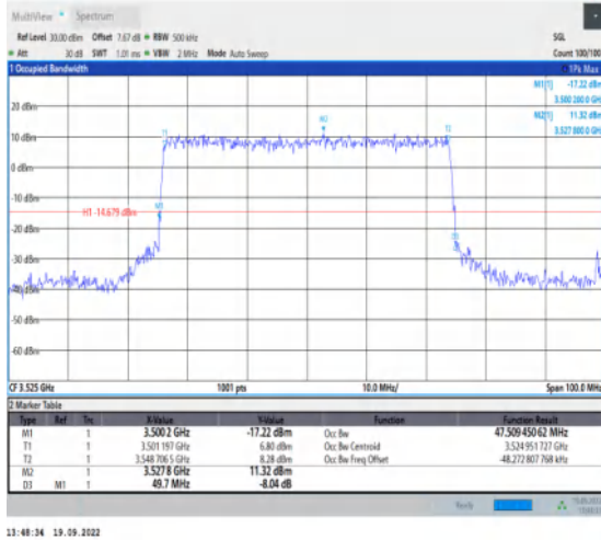
1-N78-3450-3550--30-50-H-7-CP-16QAM-Outer_Full -133@0-Ant1-47.509-49.700-≤50-PASS
