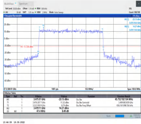
1-N78-3450-3550--30-50-M-1-DFT-QPSK-Outer_Full -128@0-Ant1-45.752-47.400-≤50-PASS
