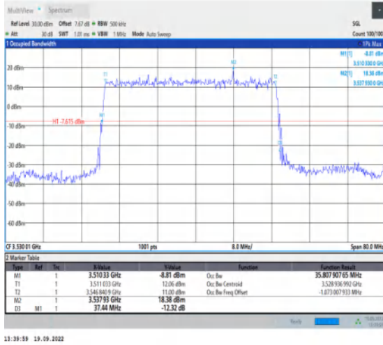
1-N78-3450-3550--30-40-H-2-DFT-PI2BPSK-Outer_Full-100@0-Ant1-35.808-37.440-≤40-PASS
