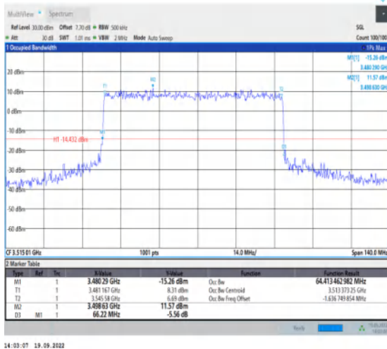
1-N78-3450-3550--30-70-H-3-DFT-16QAM-Outer_Fu -180@0-Ant1-64.413-66.220-≤70-PASS
