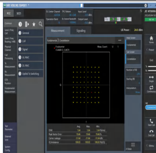
1-N78-3450-3550--30-100-M-4-DFT-64QAM-Outer_Full-270@0-Ant1-see graph-PASS
