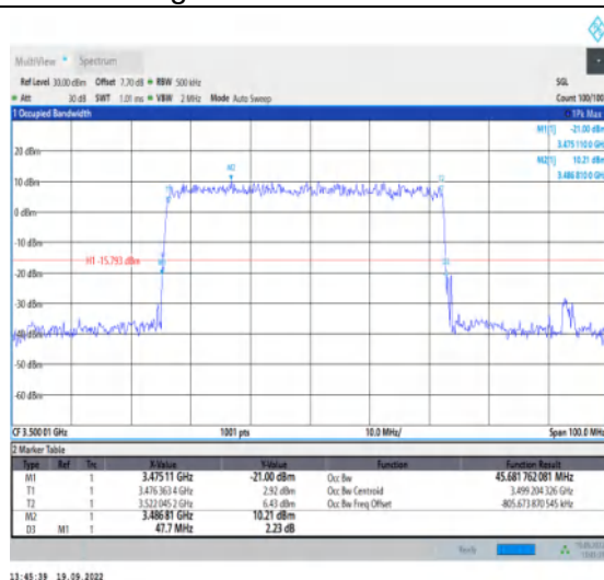
1-N78-3450-3550--30-50-M-5-DFT-256QAM-Outer_Full-128@0-Ant1-45.682-47.700-≤50-PASS
