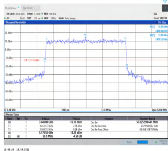
1-N78-3450-3550--30-60-L-1-DFT-QPSK-Outer_Full -162@0-Ant1-57.626-60.000-≤60-PASS
