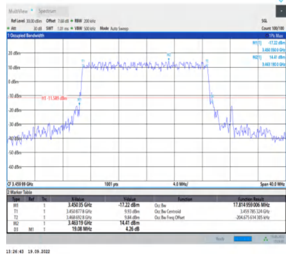
1-N78-3450-3550--30-20-L-2-DFT-PI2BPSK-Outer_F ull-50@0-Ant1-17.815-19.080≤20-PASS
