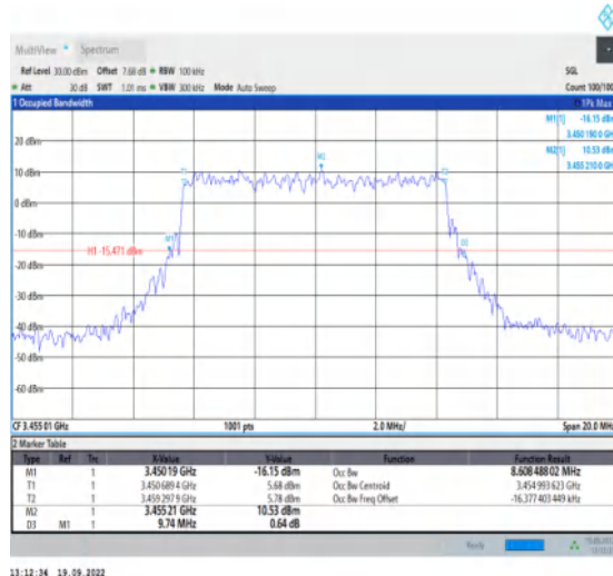
1-N78-3450-3550--30-10-L-8-CP-64QAM-Outer_Full -24@0-Ant1-8.608-9.740-≤10-PASS
