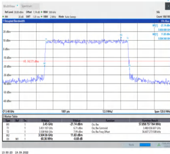
1-N78-3450-3550--30-60-L-4-DFT-64QAM-Outer_Full-162@0-Ant1-57.859-60.360-≤60-PASS
