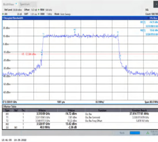
1-N78-3450-3550--30-40-H-6-CP-QPSK-Outet_Full-106@0-Ant1-37.915-40.000-≤40-PASS
