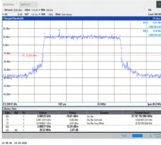
1-N78-3450-3550--30-40-M-7-CP-16QAM-Outer_Full I-106@0-Ant1-37.762-39.520≤40-PASS
