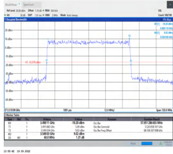
1-N78-3450-3550--30-60-H-5-DFT-256QAM-Outer_F ull-162@0-Ant1-57.951-60.000-≤60-PASS
