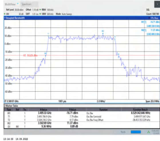
1-N78-3450-3550--30-10-M-5-DFT-256QAM-Outer_Full-24@0-Ant1-8.529-9.360≤10-PASS
