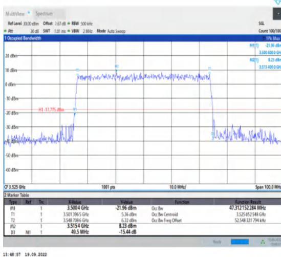
1-N78-3450-3550--30-50-H-9-CP-256QAM-Outer_Full -133@0-Ant1-47.312-49.500-≤50-PASS
