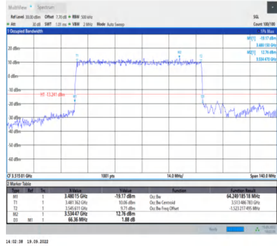
1-N78-3450-3550--30-70-H-2-DFT-PI2BPSK-Outer_Full -180@0-Ant1-64.249-66.360-≤70-PASS
