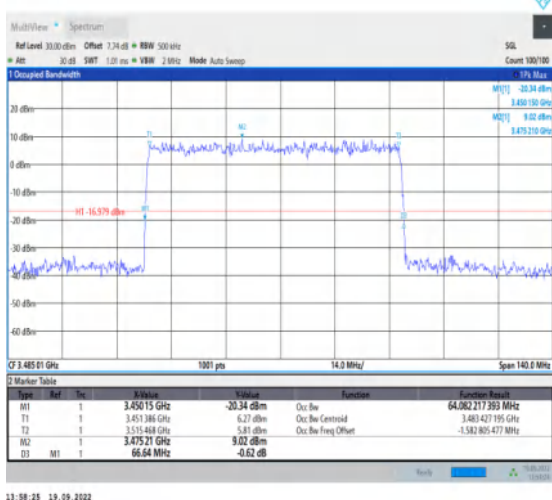
1-N78-3450-3550--30-70-L-5-DFT-256QAM-Outer_F ull-180@0-Ant1-64.082-66.640-≤70-PASS
