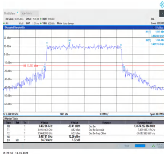
1-N78-3450-3550--30-15-M-8-CP-64QAM-Outer_Full-38@0-Ant1-13.674-14.730-≤15-PASS
