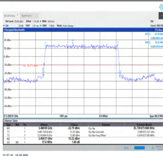
1-N78-3450-3550--30-40-M-2-DFT-PI2BPSK-Outer_Full Full-100@0-Ant1-35.739-37.600-≤40-PASS
