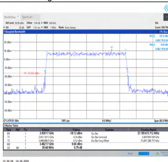
1-N78-3450-3550--30-40-L-9-CP-256QAM-Outer_Fu ll-106@0-Ant1-37.786-39.680-≤40-PASS
