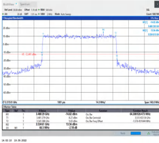
1-N78-3450-3550--30-70-H-1-DFT-QPSK-Outer_Full -180@0-Ant1-64.309-66.500-≤70-PASS
