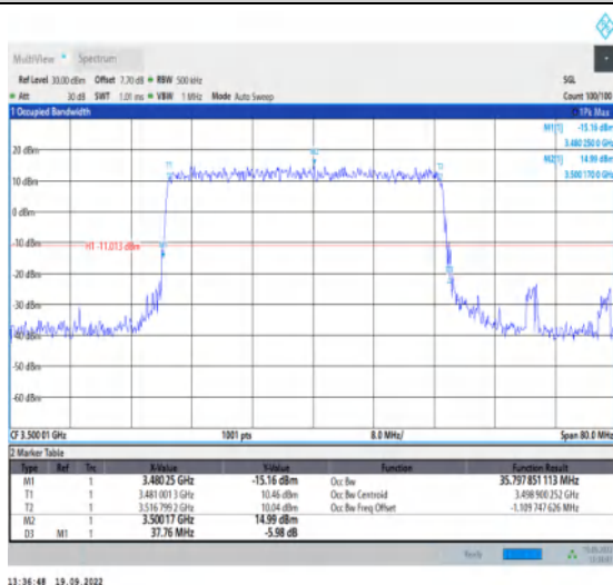
1-N78-3450-3550--30-40-M-1-DFT-QPSK-Outer_Full -100@0-Ant1-35.798-37.760-≤40-PASS
