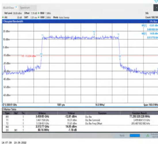
1-N78-3450-3550--30-80-M-1-DFT-QPSK-Outer_Full -216@0-Ant1-77.293-80.160-≤80-PASS
