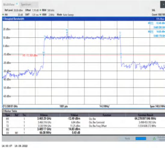
1-N78-3450-3550--30-70-M-2-DFT-PI2BPSK-Outer_Full-180@0-Ant1-64.278-66.080-≤70-PASS
