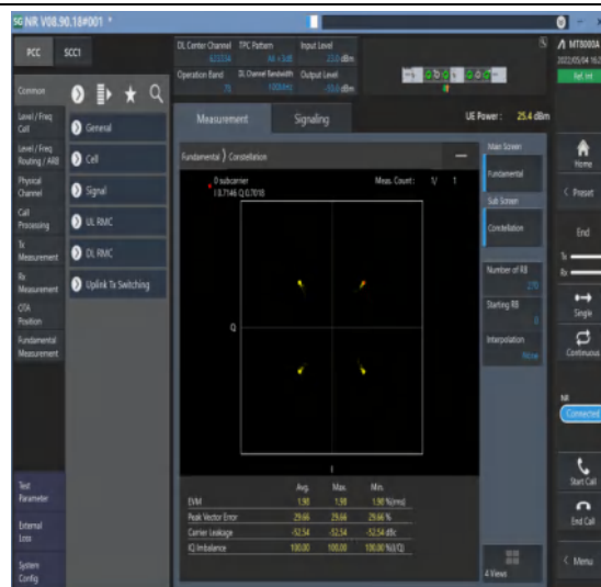
1-N78-3450-3550--30-100-M-2-DFT-QPSK-Outer_Full-270@0-Ant1-see graph-PASS
