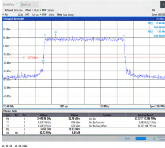
1-N78-3450-3550--30-60-L-6-CP-QPSK-Outet_Full-162@0-Ant1-57.731-60.120-≤60-PASS
