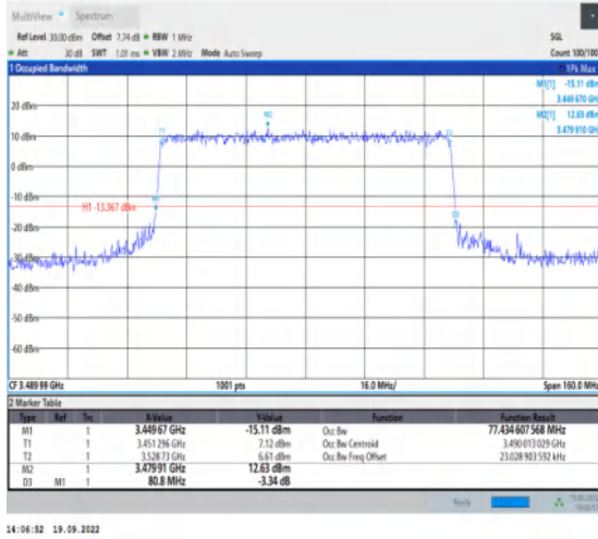
1-N78-3450-3550--30-80-L-8-CP-64QAM-Outer_Full -217@0-Ant1-77.435-80.800-≤80-PASS
