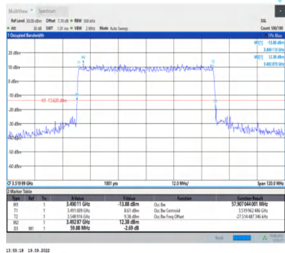
1-N78-3450-3550--30-60-H-3-DFT-16QAM-Outer_Full-162@0-Ant1-57.907-59.880-≤60-PASS
