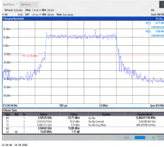
1-N78-3450-3550--30-15-H-4-DFT-64QAM-Outer_Fu ll-36@0-Ant1-12.864-13.650-≤15-PASS
