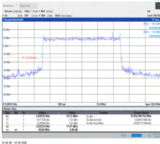
1-N78-3450-3550--30-60-M-3-DFT-16QAM-Outer_Full-162@0-Ant1-57.817-59.640-≤60-PASS
