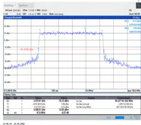
1-N78-3450-3550--30-50-M-3-DFT-16QAM-Outer_Full ull-128@0-Ant1-45.537-47.800-≤50-PASS
