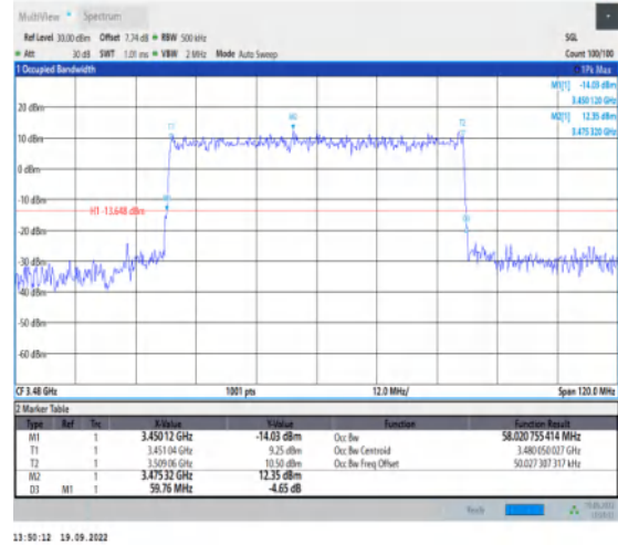
1-N78-3450-3550--30-60-L-3-DFT-16QAM-Outer_Full-162@0-Ant1-58.021-59.760-≤60-PASS
