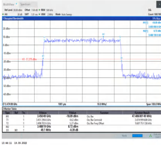
1-N78-3450-3550--30-50-L-9-CP-256QAM-Outer_Fu II-133@0-Ant1-47.406-49.100-≤50-PASS
