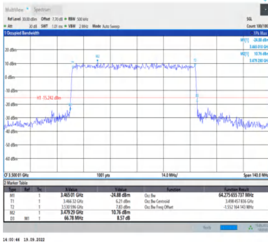
1-N78-3450-3550--30-70-M-4-DFT-64QAM-Outer_Full-180@0-Ant1-64.276-66.780-≤70-PASS
