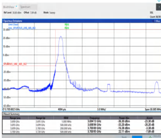
1-N77-3700-3980--30-20-L-4-CP-QPSK-Edge_1RB_L eft-1@0-Ant1-1--PASS-see graph
