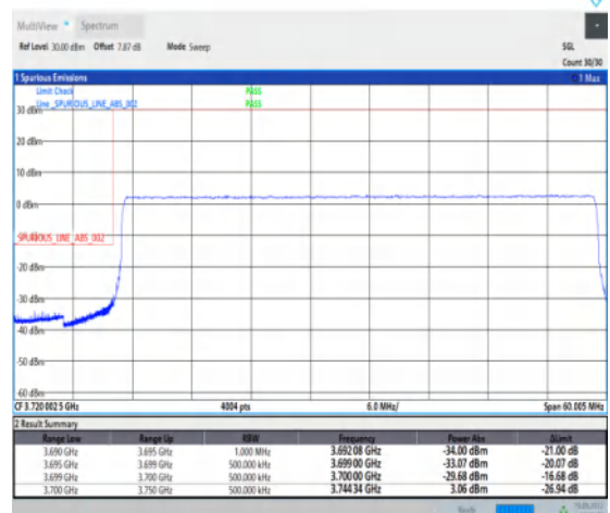
1-N77-3700-3980--30-50-L-6-CP-QPSK-Outer_Full-133@0-Ant1-1--PASS-see graph
