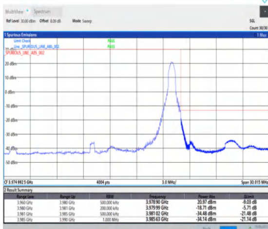
1-N77-3700-3980--30-20-H-5-CP-QPSK-Edge_1RB_R ight-1@50-Ant1-1--PASS-see graph
