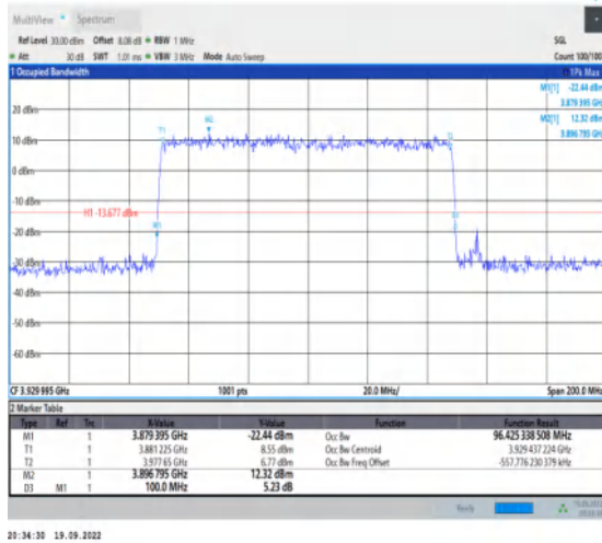
1-N77-3700-3980--30-100-H-4-DFT-64QAM-Outer_Full-270@0-Ant1-96.425-100.000-≤100-PASS
