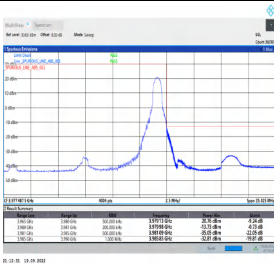
1-N77-3700-3980--30-15-H-2-DFT-PI2BPSK-Edge_1R_B_Right-1@37-Ant1-1--PASS-see graph
