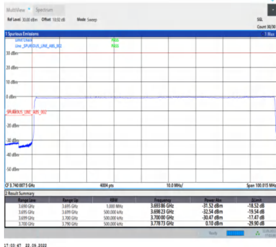
1-N77-3700-3980-PC2-30-90-L-6-CP-QPSK-Outer _Full-245@0-Ant1-1--PASS-see graph
