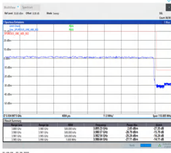
1-N77-3700-3980--30-100-H-3-DFT-PI2BPSK-Out_er_Full-270@0-Ant1-1--PASS-see graph
