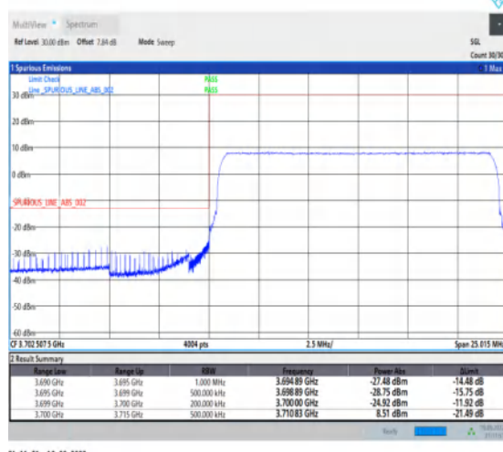
1-N77-3700-3980--30-15-L-6-CP-QPSK-Outer_Full-38@0-Ant1-1--PASS-see graph
