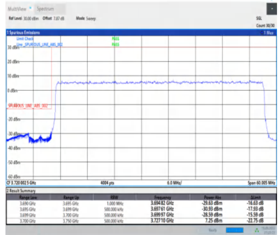
1-N77-3700-3980--30-50-L-3-DFT-PI2BPSK-Outer_Full-128@0-Ant1-1--PASS-see graph
