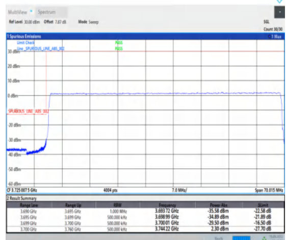
1-N77-3700-3980--30-60-L-6-CP-QPSK-Outer_Full-162@0-Ant1-1--PASS-see graph
