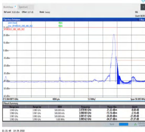
1-N77-3700-3980--30-40-H-5-CP-QPSK-Edge_1RB_R ight-1@105-Ant1-1--PASS-see graph
