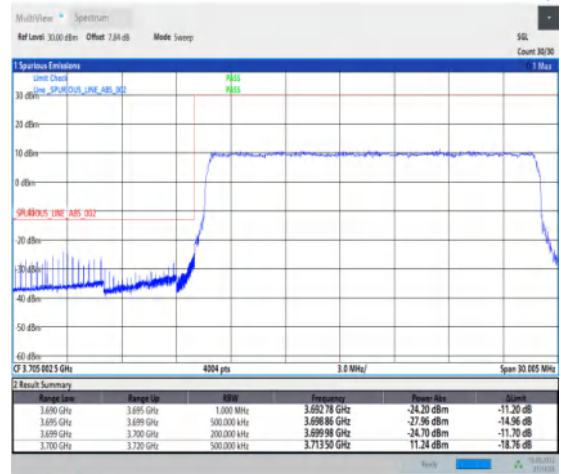
1-N77-3700-3980--30-20-L-3-DFT-PI2BPSK-Outer _Full-50@0-Ant1-1--PASS-see graph
