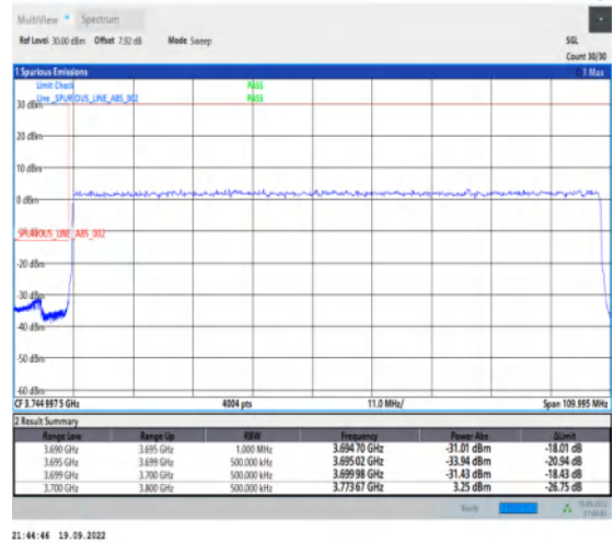
1-N77-3700-3980--30-100-L-3-DFT-PI2BPSK-Outer_Full-270@0-Ant1-1--PASS-see graph
