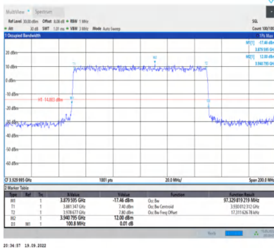
1-N77-3700-3980--30-100-H-6-CP-QPSK-Outer_Full-273@0-Ant1-97.33-100.800-≤100-PASS
