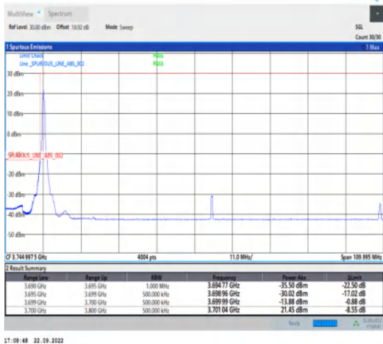
1-N77-3700-3980-PC2-30-100-L-4-CP-QPSK-Edge_1 RB_Left-1@0-Ant1-1--PASS-see graph
