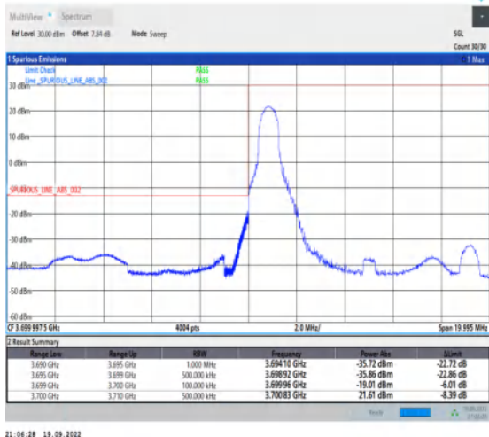
1-N77-3700-3980--30-10-L-1-DFT-PI2BPSK-Edge_1R_B_Left-1@0-Ant1-1--PASS-see graph
