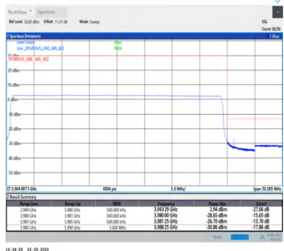
1-N77-3700-3980-PC2-30-40-H-6-CP-QPSK-Outer _Full-106@0-Ant1-1--PASS-see graph
