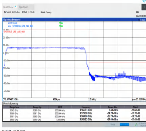
1-N77-3700-3980-PC2-30-15-H-6-CP-QPSK-Outer _Full-38@0-Ant1-1--PASS-see graph
