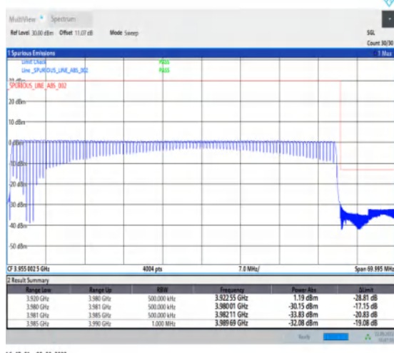
1-N77-3700-3980-PC2-30-60-H-6-CP-QPSK-Outer _Full-162@0-Ant1-1--PASS-see graph
