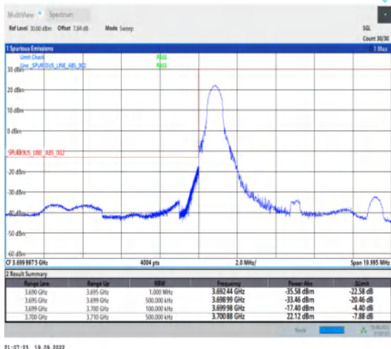
1-N77-3700-3980--30-10-L-4-CP-QPSK-Edge_1RB_Left-1@0-Ant1-1--PASS-see graph
