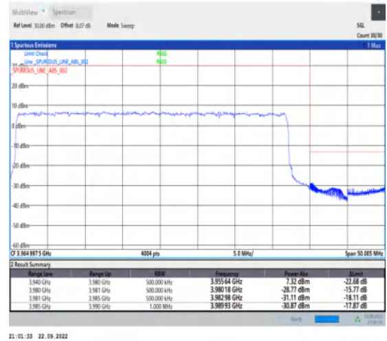
1-N77-3700-3980--30-40-H-3-DFT-PI2BPSK-Outer _Full-100@0-Ant1-1--PASS-see graph
