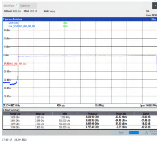
1-N77-3700-3980-PC2-30-100-L-6-CP-QPSK-Out er_Full-273@0-Ant1-1--PASS-see graph
