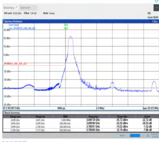
1-N77-3700-3980--30-15-L-4-CP-QPSK-Edge_1RB_Left-1@0-Ant1-1--PASS-see graph
