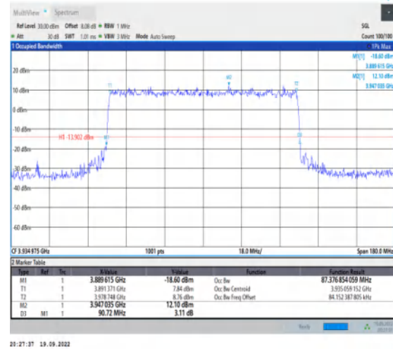
1-N77-3700-3980--30-90-H-8-CP-64QAM-Outer_Full -245@0-Ant1-87.377-90.720-≤90-PASS
