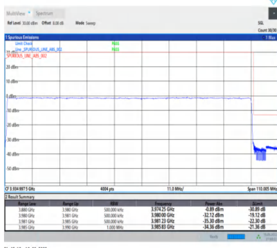
1-N77-3700-3980--30-100-H-6-CP-QPSK-Outer_Full-273@0-Ant1-1--PASS-see graph
