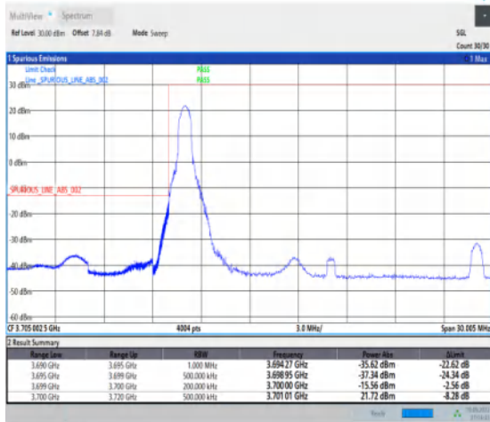
1-N77-3700-3980--30-20-L-1-DFT-PI2BPSK-Edge_1R B_Left-1@0-Ant1-1--PASS-see graph
