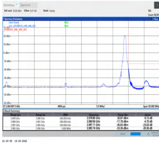
1-N77-3700-3980--30-40-H-2-DFT-PI2BPSK-Edge_1R B_Right-1@105-Ant1-1--PASS-see graph
