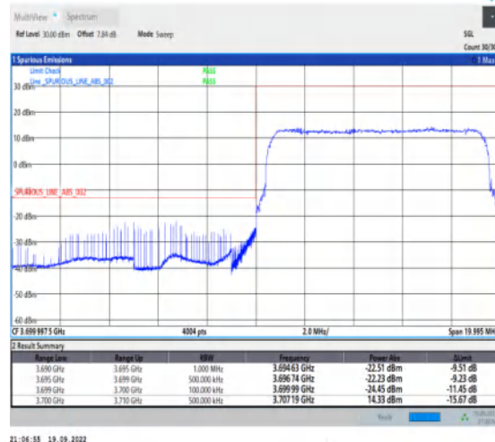
1-N77-3700-3980--30-10-L-3-DFT-PI2BPSK-Outer_Full-24@0-Ant1-1--PASS-see graph
