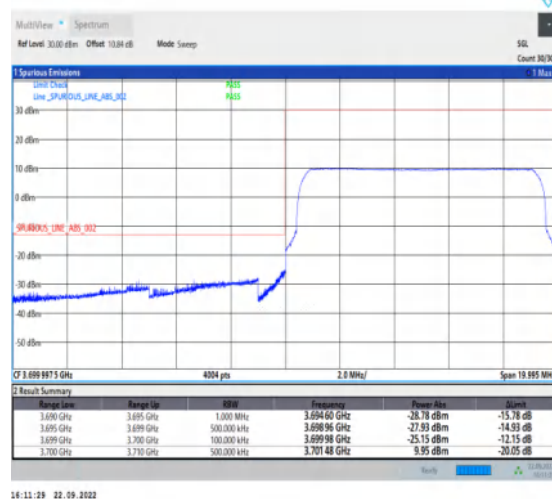
1-N77-3700-3980-PC2-30-10-L-6-CP-QPSK-Outer _Full-24@0-Ant1-1--PASS-see graph
