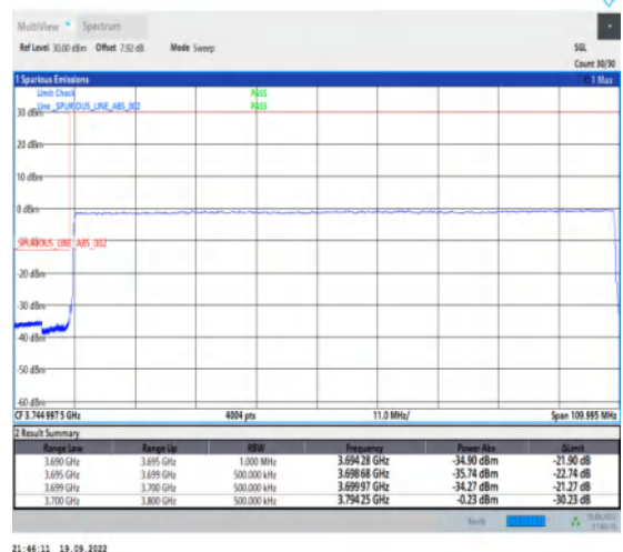
1-N77-3700-3980--30-100-L-6-CP-QPSK-Outer_Full-273@0-Ant1-1--PASS-see graph
