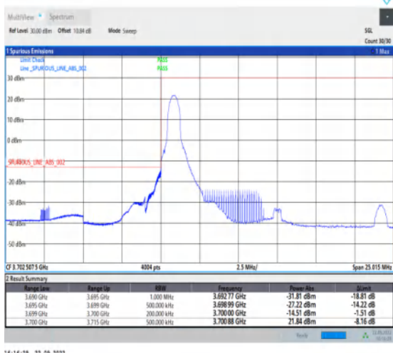
1-N77-3700-3980-PC2-30-15-L-4-CP-QPSK-Edge_1R B_Left-1@0-Ant1-1--PASS-see graph
