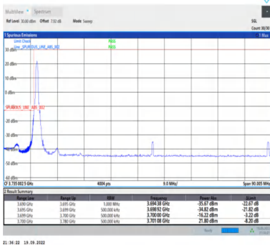
1-N77-3700-3980--30-80-L-4-CP-QPSK-Edge_1RB_Left-1@0-Ant1-1--PASS-see graph
