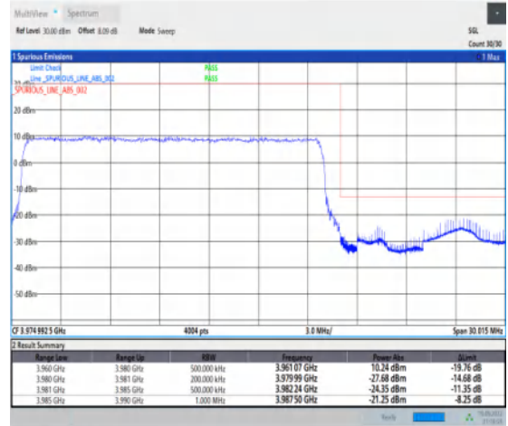
1-N77-3700-3980--30-20-H-3-DFT-PI2BPSK-Outer_Full-50@0-Ant1-1--PASS-see graph
