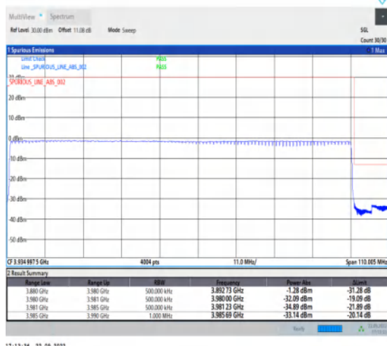
1-N77-3700-3980-PC2-30-100-H-6-CP-QPSK-Out er_Full-273@0-Ant1-1--PASS-see graph
