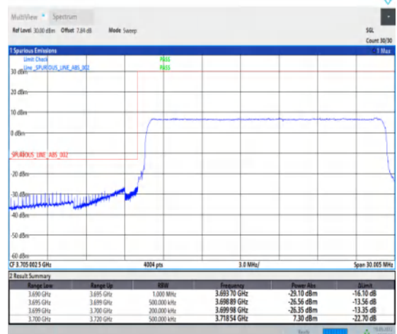
1-N77-3700-3980--30-20-L-6-CP-QPSK-Outer_Ful l-51@0-Ant1-1--PASS-see graph
