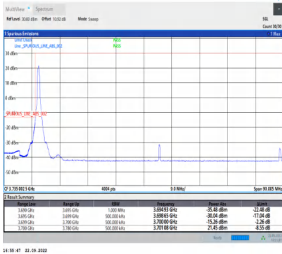
1-N77-3700-3980-PC2-30-80-L-4-CP-QPSK-Edge_1R B_Left-1@0-Ant1-1--PASS-see graph
