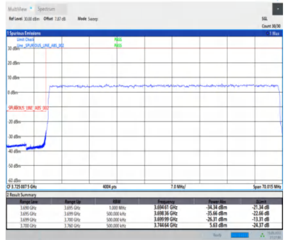
1-N77-3700-3980--30-60-L-3-DFT-PI2BPSK-Outer_Full-162@0-Ant1-1--PASS-see graph
