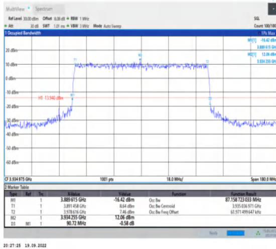
1-N77-3700-3980--30-90-H-7-CP-16QAM-Outer_Full I-245@0-Ant1-87.159-90.720-≤90-PASS
