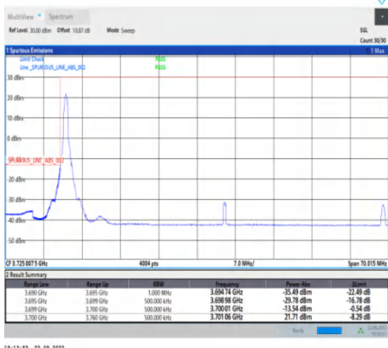
1-N77-3700-3980-PC2-30-60-L-4-CP-QPSK-Edge_1R B_Left-1@0-Ant1-1--PASS-see graph
