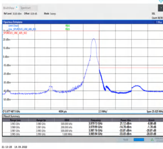
1-N77-3700-3980--30-15-H-5-CP-QPSK-Edge_1RB_Right-1@37-Ant1-1--PASS-see graph
