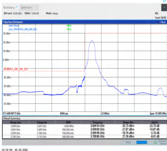
1-N77-3700-3980-PC2-30-10-L-4-CP-QPSK-Edge_1R B_Left-1@0-Ant1-1--PASS-see graph
