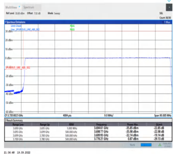
1-N77-3700-3980--30-80-L-6-CP-QPSK-Outer_Full-217@0-Ant1-1--PASS-see graph
