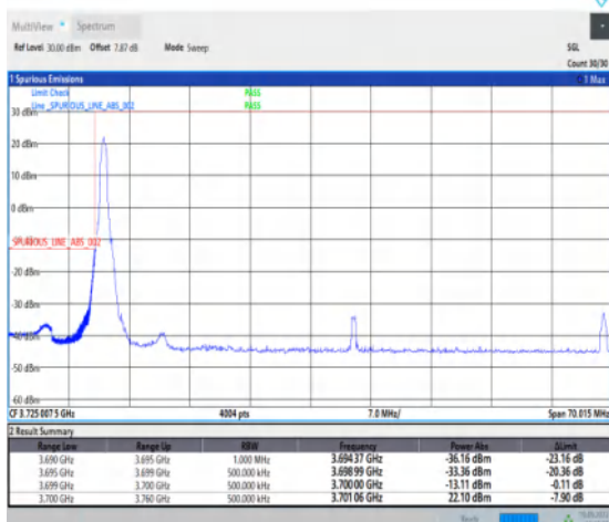
1-N77-3700-3980--30-60-L-4-CP-QPSK-Edge_1RB_Left-1@0-Ant1-1--PASS-see graph
