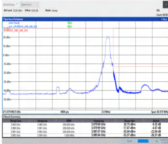
1-N77-3700-3980--30-20-H-2-DFT-PI2BPSK-Edge_1R_B_Right-1@50-Ant1-1--PASS-see graph
