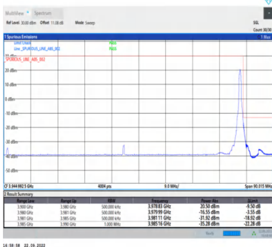
1-N77-3700-3980-PC2-30-80-H-5-CP-QPSK-Edge_1R B_Right-1@216-Ant1-1--PASS-see graph
