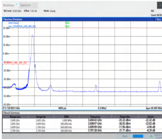
1-N77-3700-3980--30-50-L-1-DFT-PI2BPSK-Edge_1R_B_Left-1@0-Ant1-1--PASS-see graph
