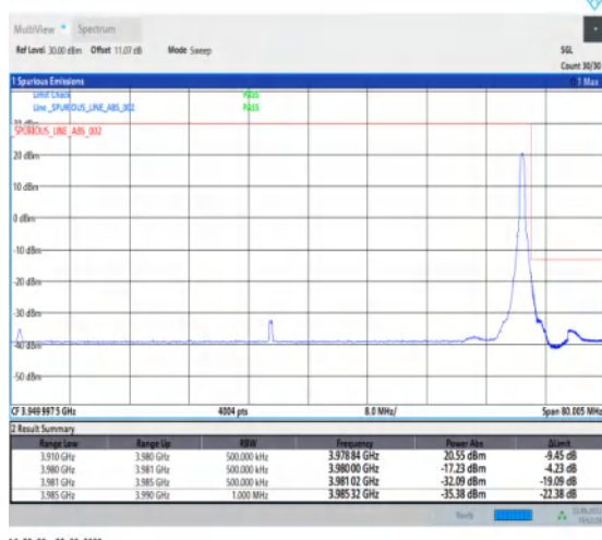
1-N77-3700-3980-PC2-30-70-H-5-CP-QPSK-Edge_1R B_Right-1@188-Ant1-1--PASS-see graph
