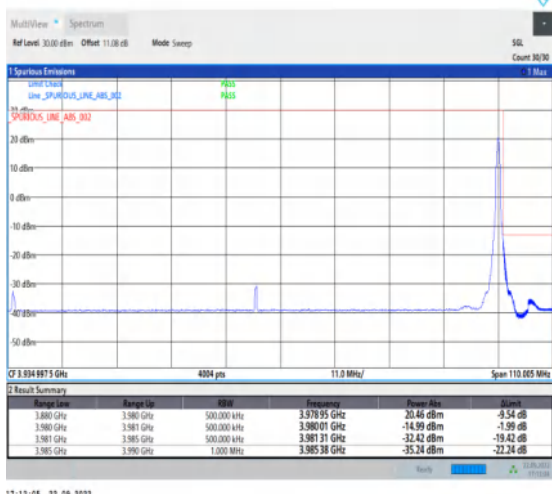
1-N77-3700-3980-PC2-30-100-H-5-CP-QPSK-Edge_1 RB_Right-1@272-Ant1-1--PASS-see graph
