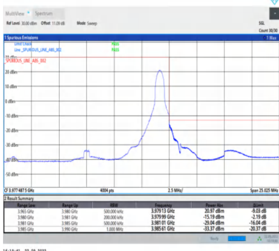
1-N77-3700-3980-PC2-30-15-H-5-CP-QPSK-Edge_1R B_Right-1@37-Ant1-1--PASS-see graph
