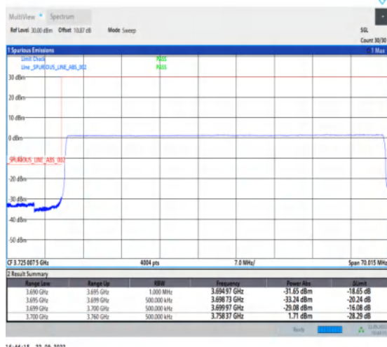
1-N77-3700-3980-PC2-30-60-L-6-CP-QPSK-Outer _Full-162@0-Ant1-1--PASS-see graph
