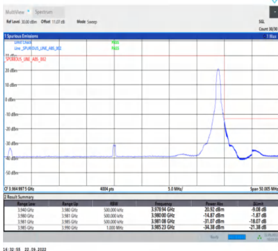
1-N77-3700-3980-PC2-30-40-H-5-CP-QPSK-Edge_1R B_Right-1@105-Ant1-1--PASS-see graph
