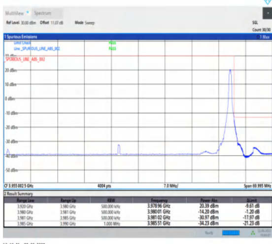
1-N77-3700-3980-PC2-30-60-H-5-CP-QPSK-Edge_1R B_Right-1@161-Ant1-1--PASS-see graph
