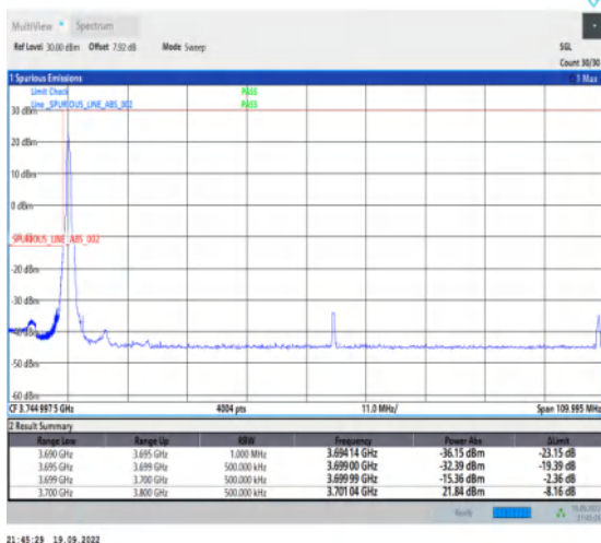
1-N77-3700-3980--30-100-L-4-CP-QPSK-Edge_1RB_Left-1@0-Ant1-1--PASS-see graph
