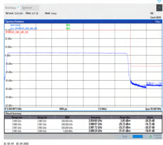
1-N77-3700-3980--30-40-H-6-CP-QPSK-Outer_Ful l-106@0-Ant1-1--PASS-see graph
