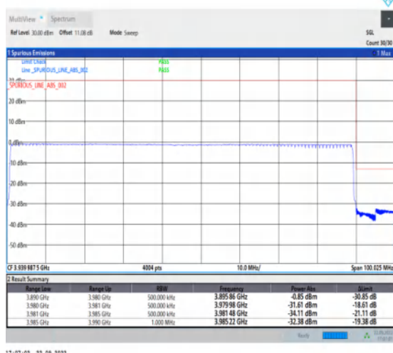
1-N77-3700-3980-PC2-30-90-H-6-CP-QPSK-Outer _Full-245@0-Ant1-1--PASS-see graph
