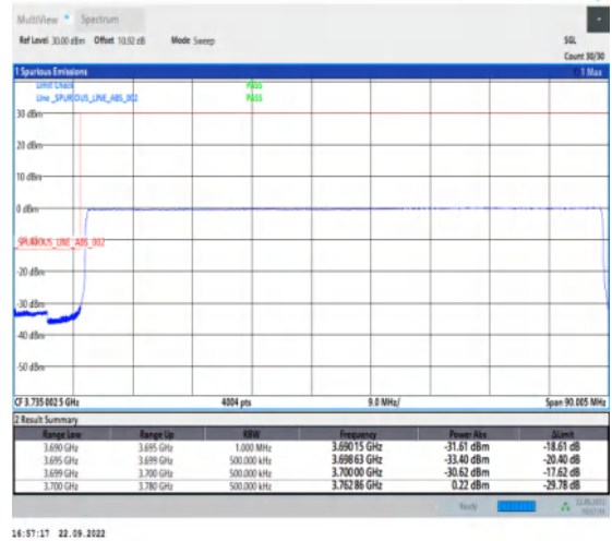
1-N77-3700-3980-PC2-30-80-L-6-CP-QPSK-Outer _Full-217@0-Ant1-1--PASS-see graph
