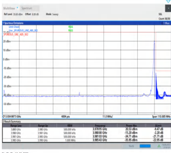
1-N77-3700-3980--30-100-H-5-CP-QPSK-Edge_1RB_Right-1@272-Ant1-1--PASS-see graph
