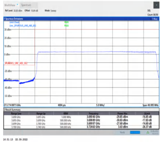
1-N77-3700-3980-PC2-30-40-L-6-CP-QPSK-Outer _Full-106@0-Ant1-1--PASS-see graph
