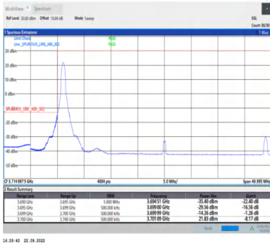
1-N77-3700-3980-PC2-30-40-L-4-CP-QPSK-Edge_1R B_Left-1@0-Ant1-1--PASS-see graph
