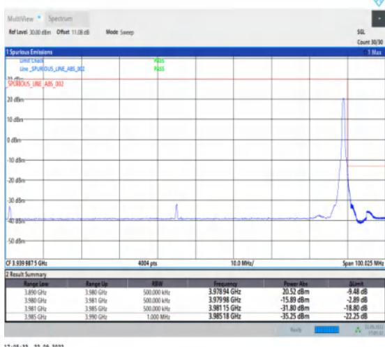
1-N77-3700-3980-PC2-30-90-H-5-CP-QPSK-Edge_1R B_Right-1@244-Ant1-1--PASS-see graph
