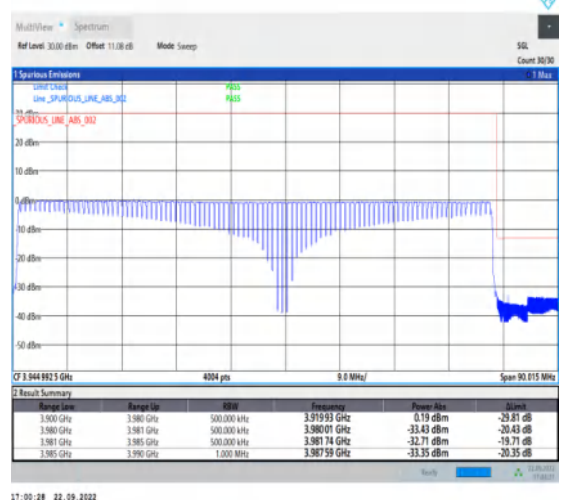
1-N77-3700-3980-PC2-30-80-H-6-CP-QPSK-Outer _Full-217@0-Ant1-1--PASS-see graph
