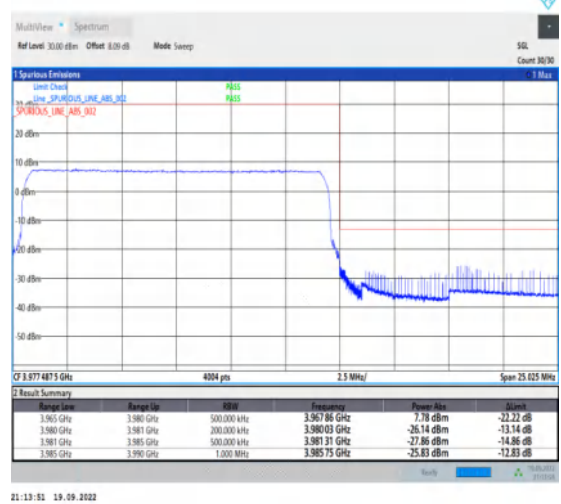
1-N77-3700-3980--30-15-H-6-CP-QPSK-Outer_Full-38@0-Ant1-1--PASS-see graph
