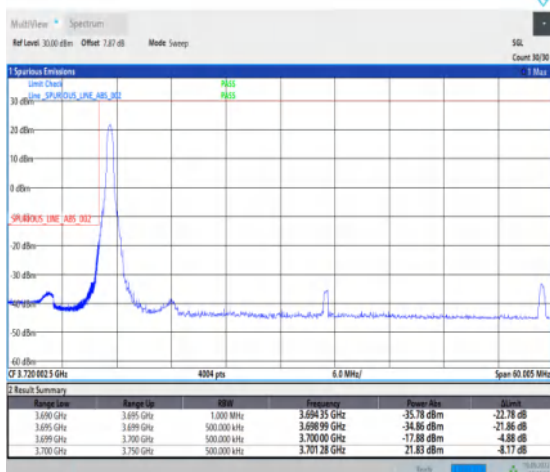
1-N77-3700-3980--30-50-L-4-CP-QPSK-Edge_1RB_Left-1@0-Ant1-1--PASS-see graph
