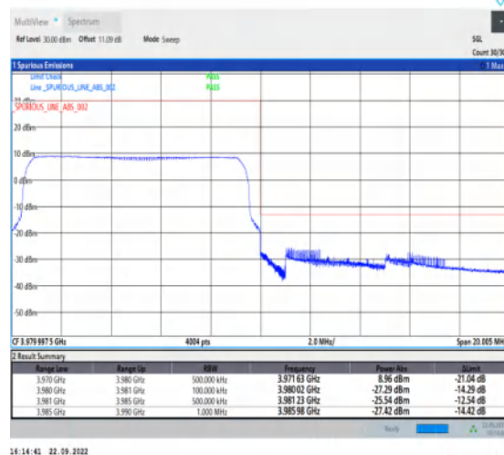
1-N77-3700-3980-PC2-30-10-H-6-CP-QPSK-Outer _Full-24@0-Ant1-1--PASS-see graph
