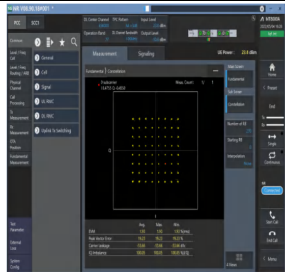
1-N77-3700-3980--30-100-M-4-DFT-64QAM-Outertest_Full-270@0-Ant1-see graph-PASS
