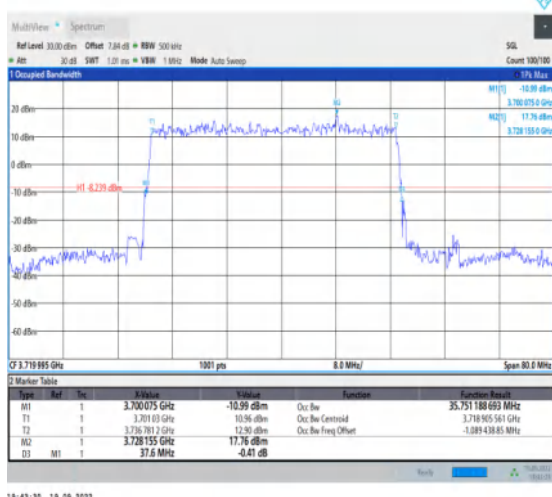
1-N77-3700-3980--30-40-L-2-DFT-P12BPSK-Outer_Full-100@0-Ant1-35.751-37.600-≤40-PASS
