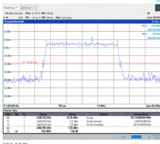
1-N77-3700-3980--30-20-M-9-CP-256QAM-Outer_Fu-II-51@0-Ant1-18.116-19.600-≤20-PASS
