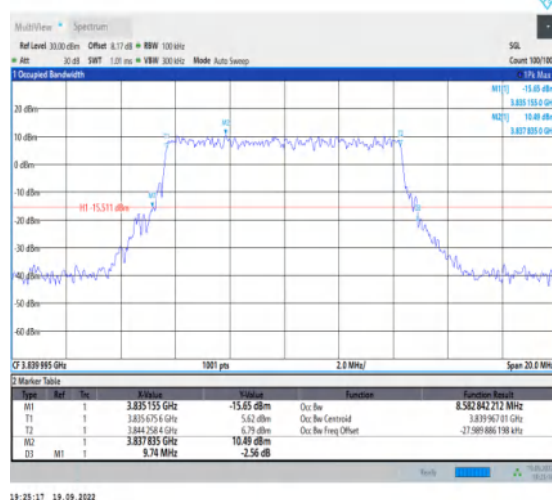
1-N77-3700-3980--30-10-M-7-CP-16QAM-Outer_F ull-24@0-Ant1-8.583-9.740-≤10-PASS
