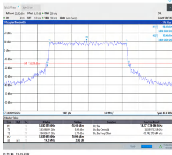
1-N77-3700-3980--30-20-M-7-CP-16QAM-Outer_Full-51@0-Ant1-18.172-19.200-≤20-PASS
