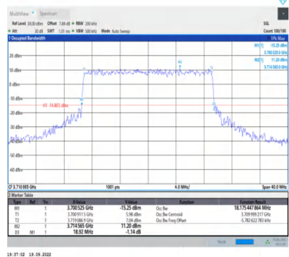
1-N77-3700-3980--30-20-L-6-CP-QPSK-Outer_Full-5 1@0-Ant1-18.175-18.920-≤20-PASS
