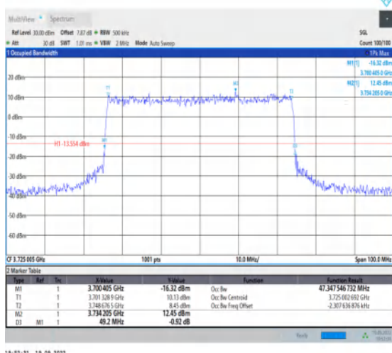
1-N77-3700-3980--30-50-L-7-CP-16QAM-Outer_Full-133@0-Ant1-47.348-49.200-≤50-PASS
