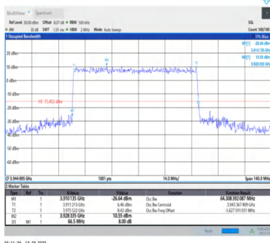
1-N77-3700-3980--30-70-H-4-DFT-64QAM-Outter_Full -180@0-Ant1-64.308-66.500-≤70-PASS
