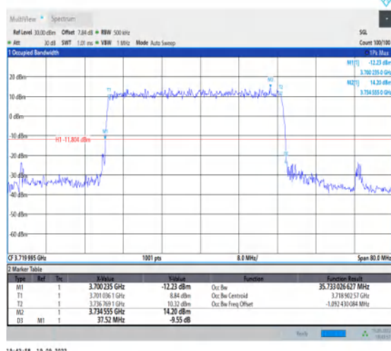
1-N77-3700-3980--30-40-L-3-DFT-16QAM-Outer_Full-100@0-Ant1-35.733-37.520-≤40-PASS
