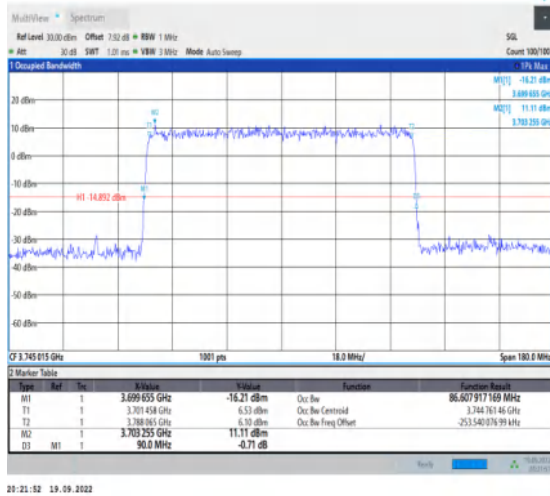
1-N77-3700-3980--30-90-L-5-DFT-256QAM-Outer_Full-243@0-Ant1-86.608-90.000-≤90-PASS
