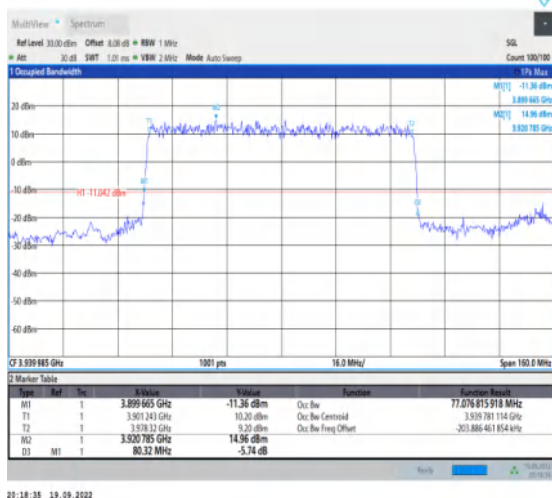
1-N77-3700-3980--30-80-H-2-DFT-PI2BPSK-Outer_Full-216@0-Ant1-77.077-80.320-≤80-PASS
