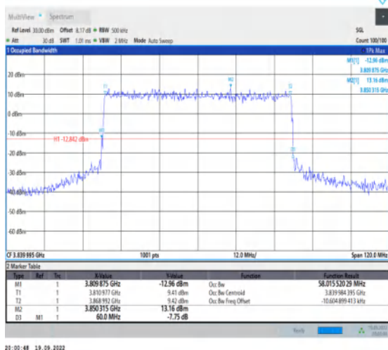
1-N77-3700-3980--30-60-M-1-DFT-QPSK-Outet_Ful I-162@0-Ant1-58.016-60.000-≤60-PASS
