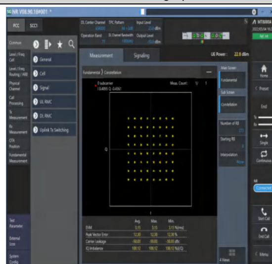
1-N77-3700-3980--30-100-M-8-CP-64QAM-Outer_Fu ull-273@0-Ant1-see graph-PASS
