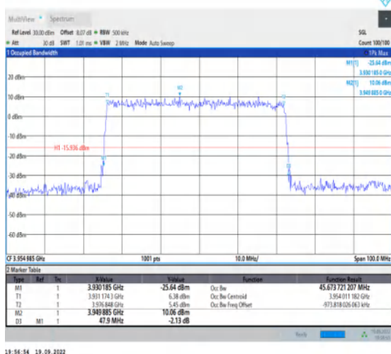
1-N77-3700-3980--30-50-H-5-DFT-256QAM-Outer_Full-128@0-Ant1-45.674-47.900-≤50-PASS
