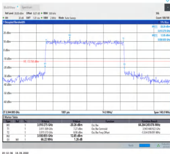
1-N77-3700-3980--30-70-H-1-DFT-QPSK-Outter_Full -180@0-Ant1-64.264-66.220-≤70-PASS
