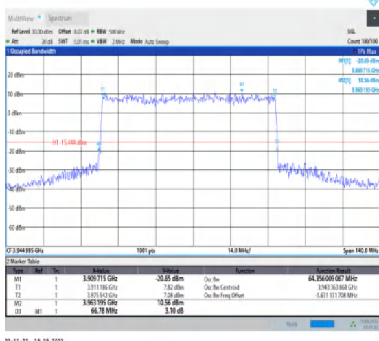
1-N77-3700-3980--30-70-H-3-DFT-16QAM-Outter_Full -180@0-Ant1-64.356-66.780-≤70-PASS
