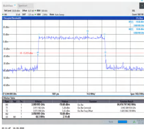
1-N77-3700-3980--30-70-H-5-DFT-256QAM-Out-er_Full-180@0-Ant1-64.417-66.500-≤70-PASS
