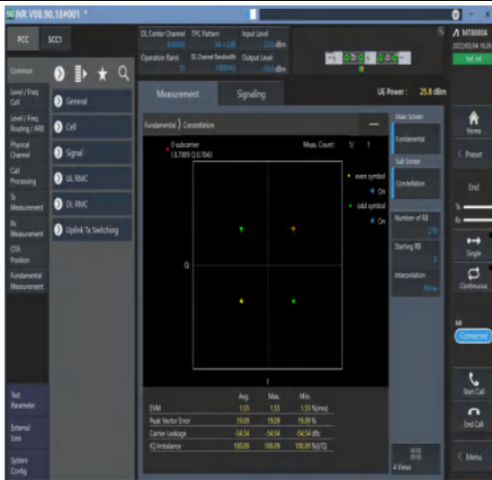
1-N77-3700-3980--30-100-M-1-DFT-PI2BPSK-Outertest_Full-270@0-Ant1-see graph-PASS
