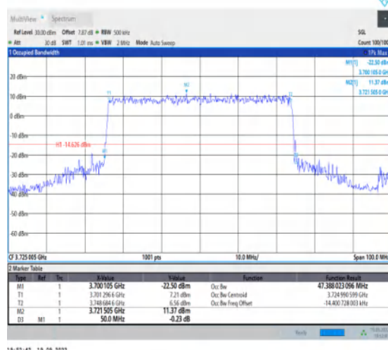
1-N77-3700-3980--30-50-L-8-CP-64QAM-Outer_Full-133@0-Ant1-47.388-50.000-≤50-PASS
