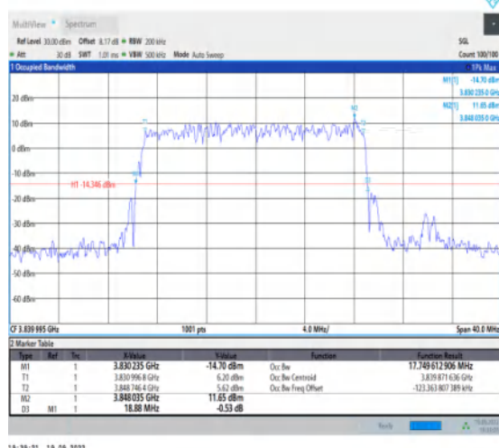
1-N77-3700-3980--30-20-M-5-DFT-256QAM-Outer_Full-50@0-Ant1-17.75-18.880-≤20-PASS
