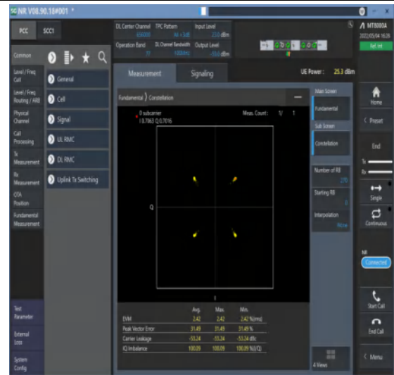
1-N77-3700-3980--30-100-M-2-DFT-QPSK-Outertest_Full-270@0-Ant1-see graph-PASS
