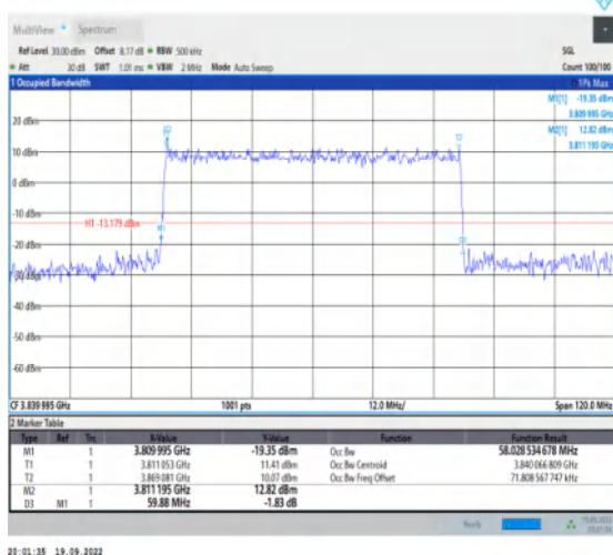
1-N77-3700-3980--30-60-M-3-DFT-16QAM-Outet_Full-162@0-Ant1-58.029-59.880-≤60-PASS
