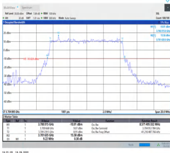
1-N77-3700-3980--30-10-L-1-DFT-QPSK-Outer_Full -24@0-Ant1-8.571-9.220≤10-PASS
