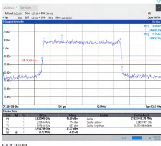
1-N77-3700-3980--30-60-H-6-CP-QPSK-Outer_Full-162@0-Ant1-57.821-60.120-≤60-PASS
