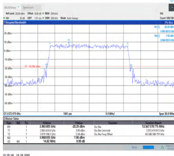
1-N77-3700-3980--30-15-H-9-CP-256QAM-Outer_Fu II-38@0-Ant1-13.568-14.820-≤15-PASS
