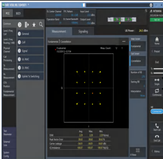
1-N77-3700-3980--30-100-M-3-DFT-16QAM-Outertest_Full-270@0-Ant1-see graph-PASS
