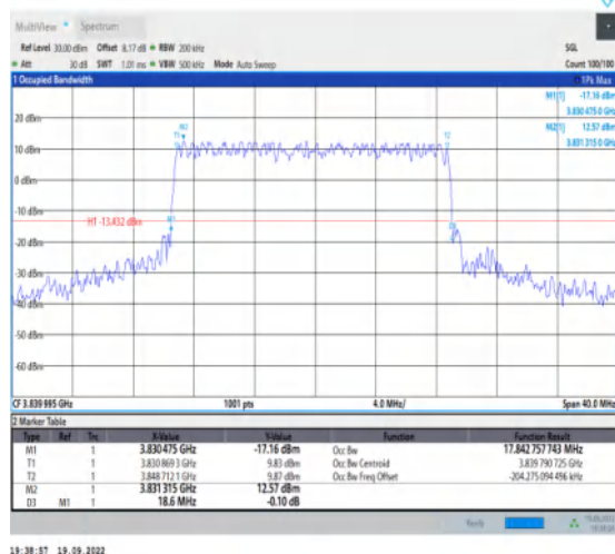
1-N77-3700-3980--30-20-M-3-DFT-16QAM-Outer_Full-50@0-Ant1-17.843-18.600-≤20-PASS
