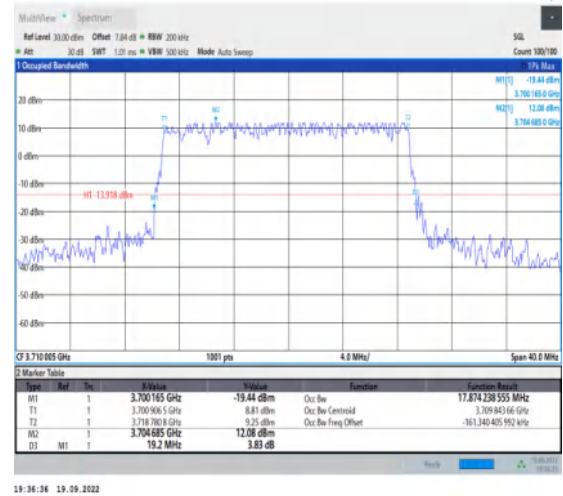
1-N77-3700-3980--30-20-L-4-DFT-64QAM-Outer_Ful I-50@0-Ant1-17.874-19.200-≤20-PASS
