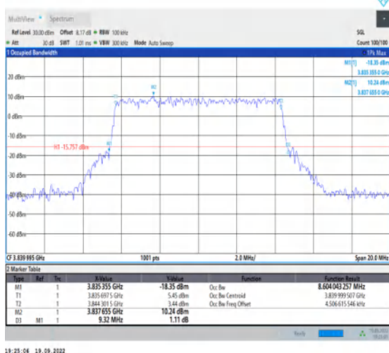
1-N77-3700-3980--30-10-M-6-CP-QPSK-Outer_F ull-24@0-Ant1-8.604-9.320-≤10-PASS
