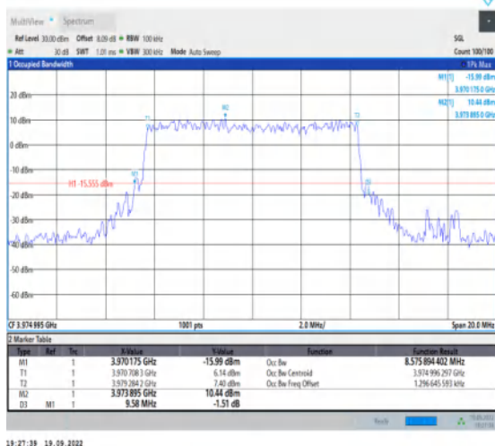
1-N77-3700-3980--30-10-H-7-CP-16QAM-Outer_Full I-24@0-Ant1-8.576-9.580-≤10-PASS
