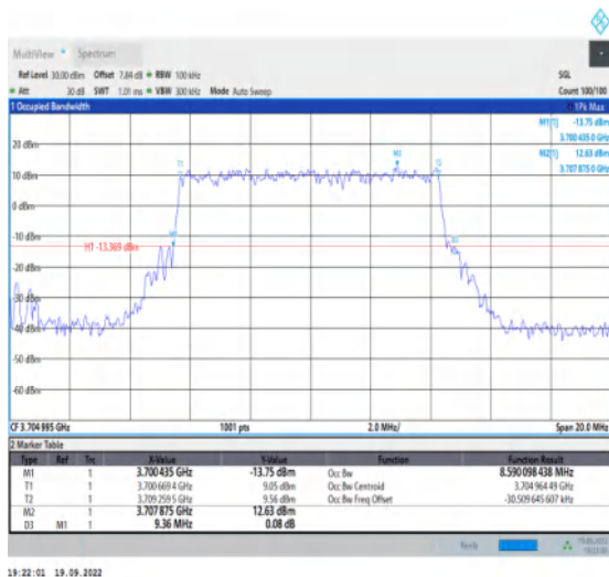
1-N77-3700-3980--30-10-L-3-DFT-16QAM-Outer_Full I-24@0-Ant1-8.59-9.360≤10-PASS
