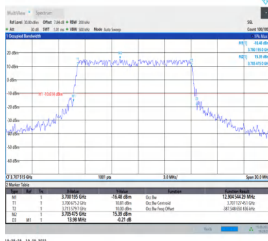
1-N77-3700-3980--30-15-L-1-DFT-QPSK-Outer_Full- 36@0-Ant1-12.905-13.980-≤15-PASS
