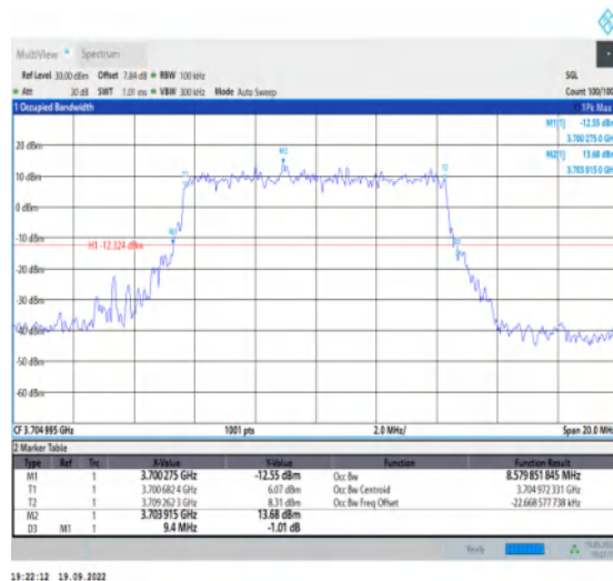
1-N77-3700-3980--30-10-L-4-DFT-64QAM-Outer_Full I-24@0-Ant1-8.58-9.400≤10-PASS
