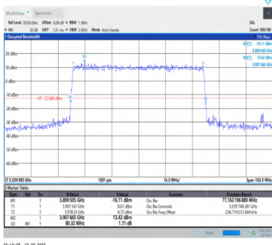
1-N77-3700-3980--30-80-H-4-DFT-64QAM-Outer_Full-216@0-Ant1-77.163-80.320-≤80-PASS
