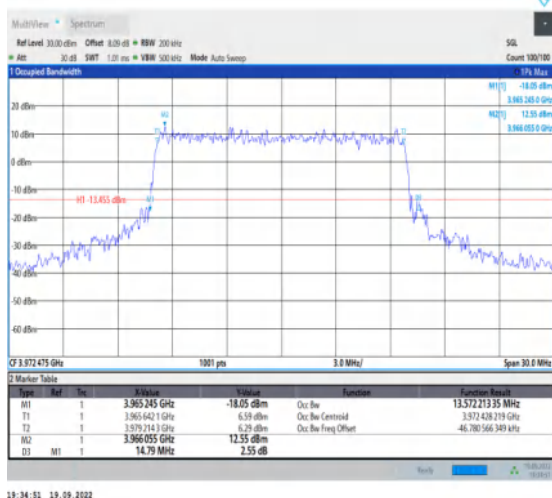
1-N77-3700-3980--30-15-H-8-CP-64QAM-Outer_Ful I-38@0-Ant1-13.572-14.790-≤15-PASS
