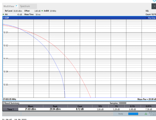
5-5-10MHz-10MHz-QPSK-QPSK-20476-20575-50RB#0-50RB#0
