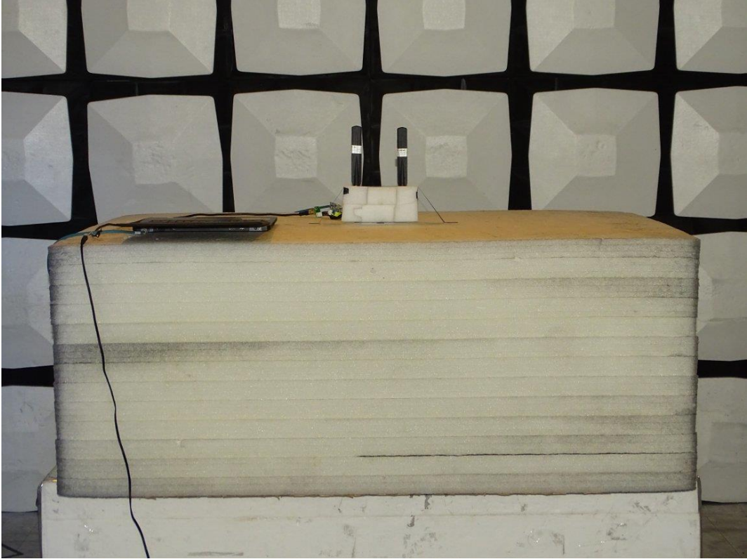
Back View of Spurious Emission Test (Horn) (Antenna No.4)
