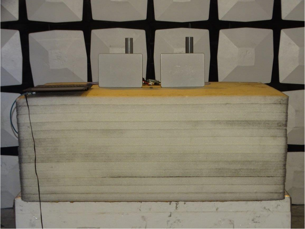
Back View of Spurious Emission Test (Horn) (Antenna No.5)
