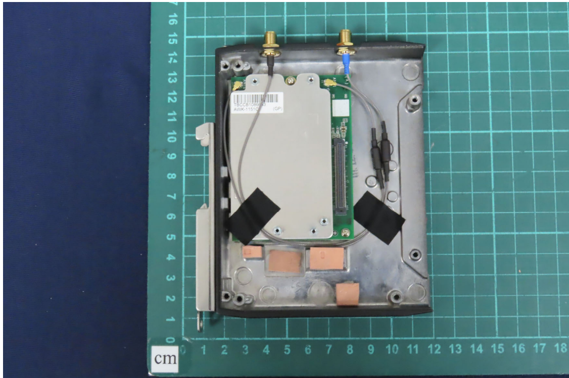
(45) EUT Photo
