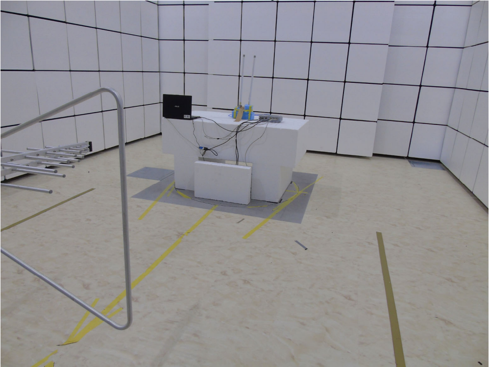
Radiated - Dipole
