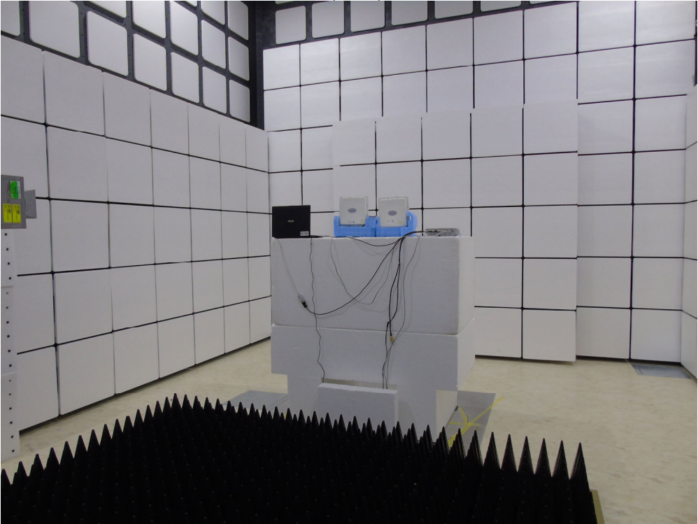
Radiated (Horn) - Panel
