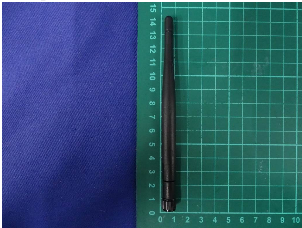
(31) EUT Photo_ANT-WDB-ARM-0202
