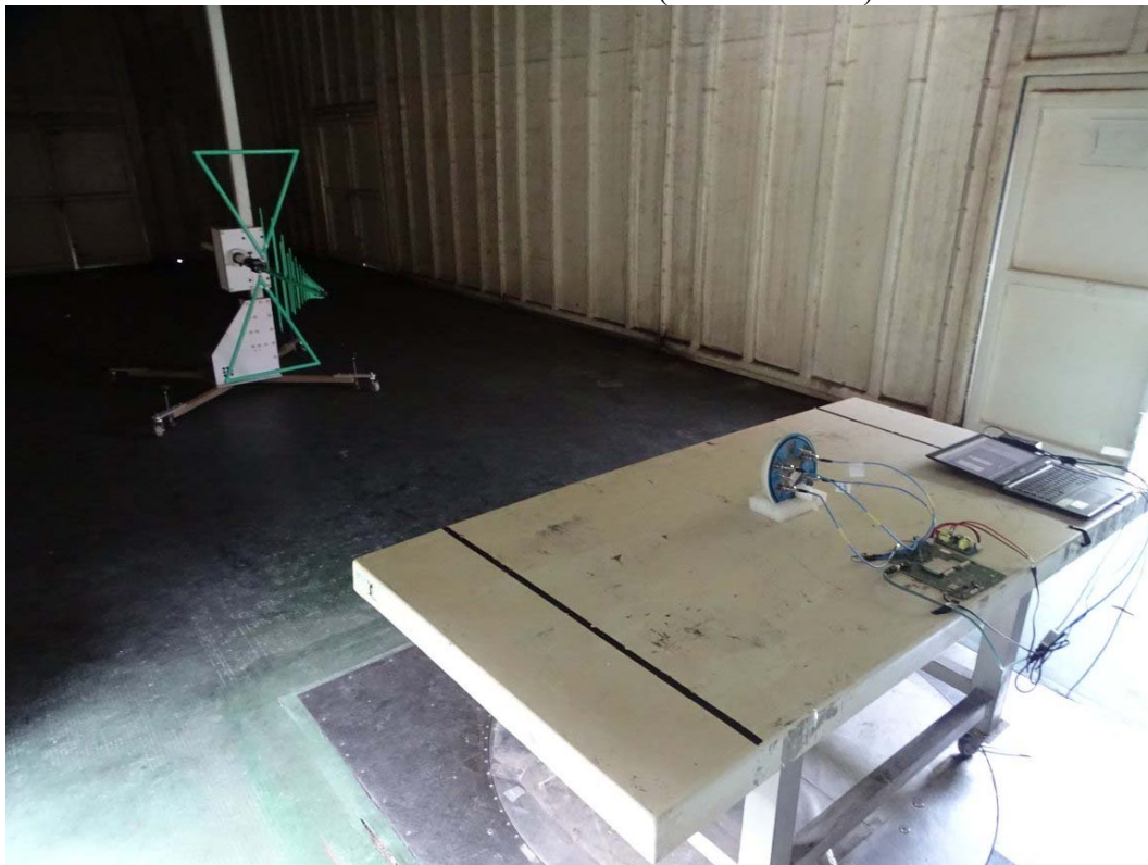
Front View of Radiated Test (Antenna No.19)
