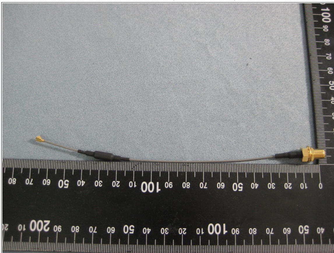
Antenna Cable (SMA-Male-RP)
