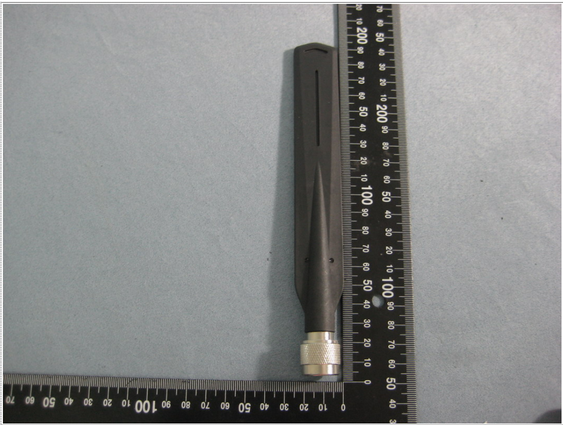
View of Antenna (ANT-WSB-ANM-05)
