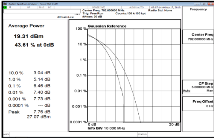
LTE_Band13_10MHz_16QAM_50_0_Low CH23230-782
