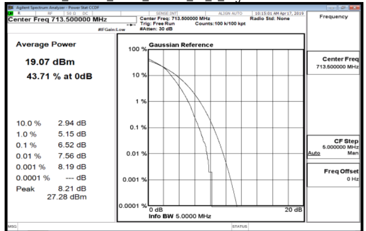
LTE_Band17_5MHz_16QAM_25_0_HighCH23825-713.5
