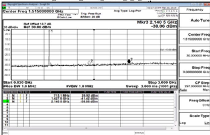
30MHz-3GHz_Band17_5MHz_QPSK_1_0_HighCH23825-713.5
