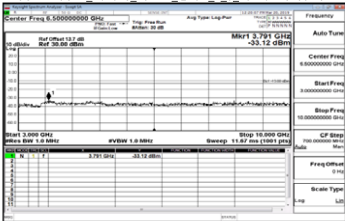
Inband-1_Band13_5MHz_QPSK_1_0_LowCH23205-779.5
