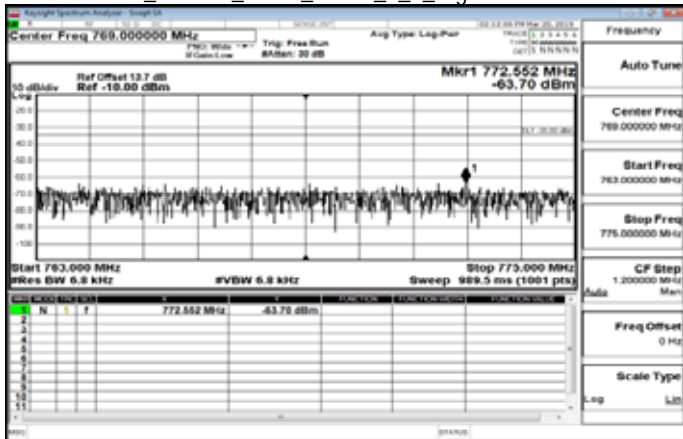
Inband-2_Band13_5MHz_QPSK_1_0_HighCH23255-784.5
