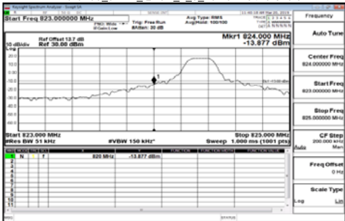
LTE\Band5_5MHz_QPSK_1_0_LowCH20425-826.5
