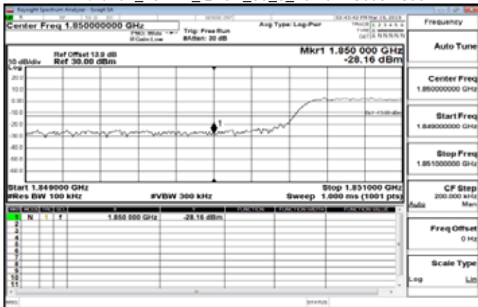
LTE\Band2_10MHz_QPSK_50_0_LowCH18650-1855
