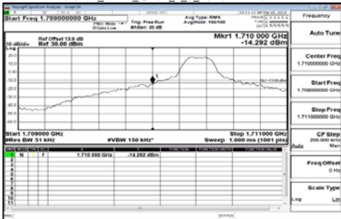
LTE\Band4_5MHz_QPSK_1_0_LowCH19975-1712.5
