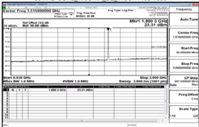
30MHz-3GHz_WCDMA_B2_MidCH9400-1880
