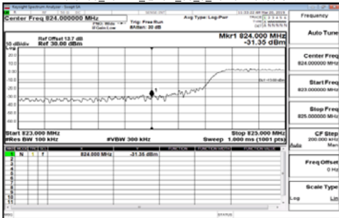
LTE\Band5_10MHz_QPSK_50_0_LowCH20450-829
