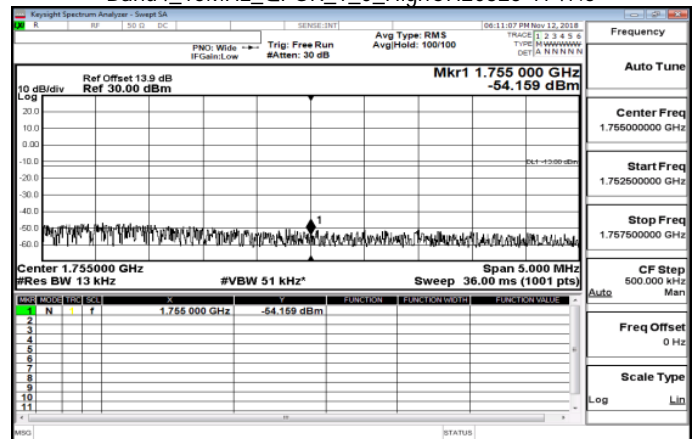
Band4_15MHz_QPSK_1_0_HighCH20325-1747.5
