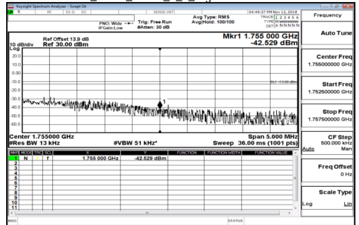
Band4_5MHz_QPSK_6_0_HighCH20375-1752.5
