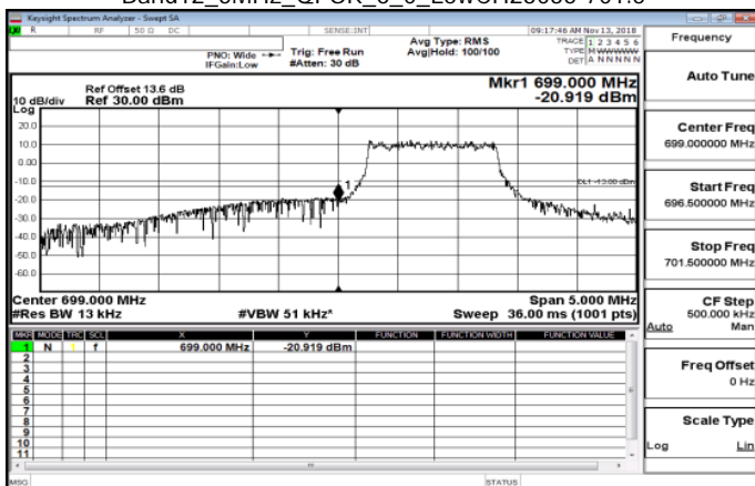
Band12_5MHz_QPSK_6_0_LowCH23035-701.5
