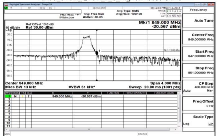
Band5_3MHz_QPSK_1_0_HighCH20635-847.5
