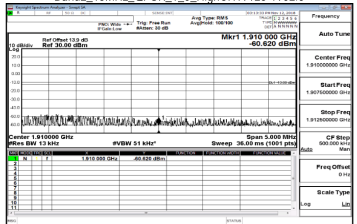
Band2_15MHz_QPSK_1_0_HighCH19125-1902.5
