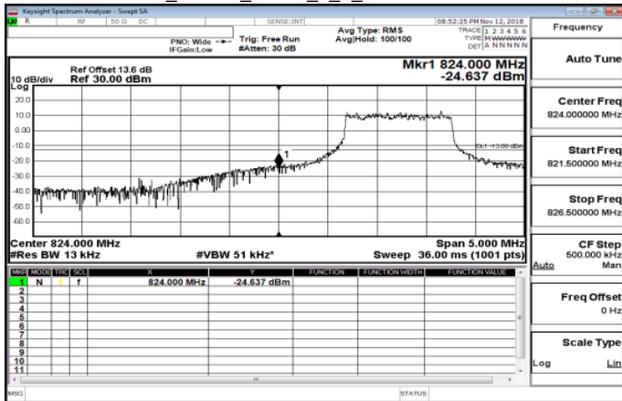
Band5_10MHz_QPSK_6_0_LowCH20450-829
