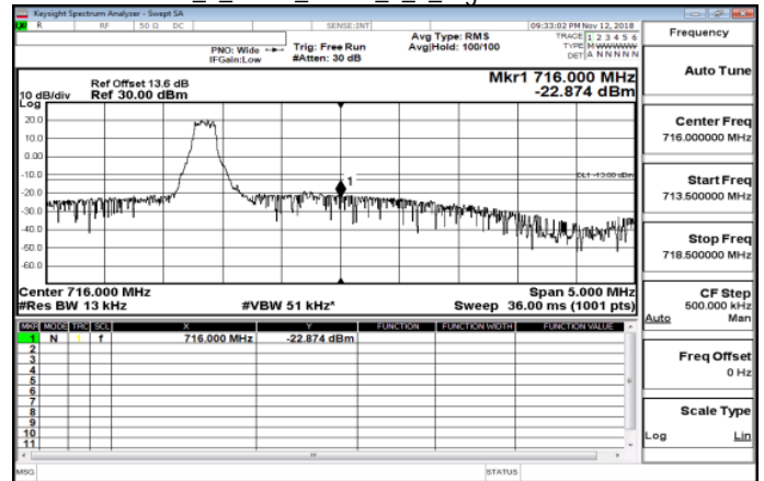
Band12_1_4MHz_QPSK_1_0_HighCH23173-715.3
