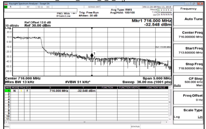
Band12_3MHz_QPSK_6_0_HighCH23165-714.5
