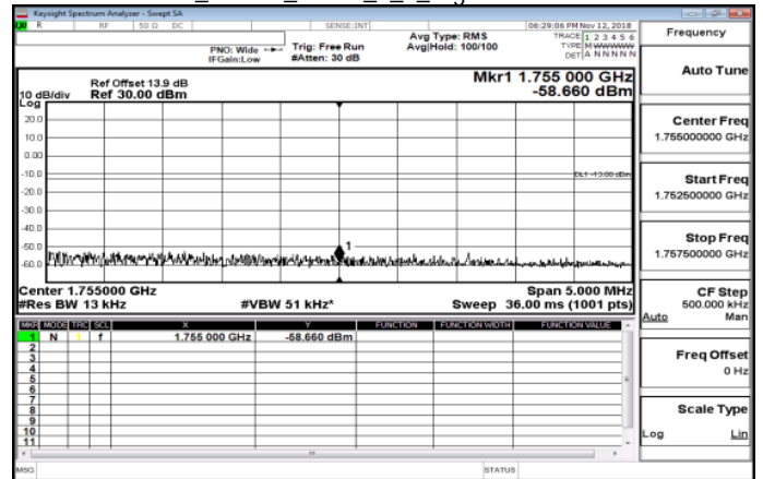
Band4_20MHz_QPSK_6_0_HighCH20300-1745
