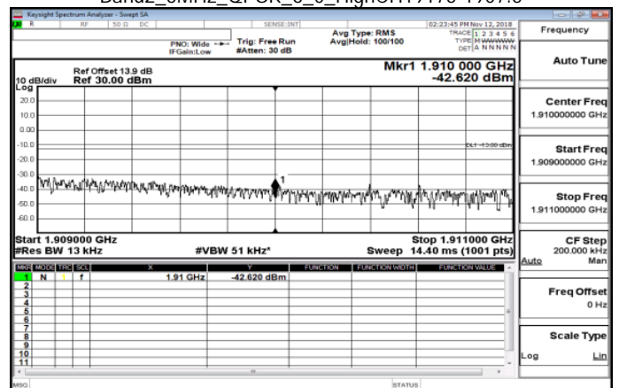
Band2_5MHz_QPSK_6_0_HighCH19175-1907.5
