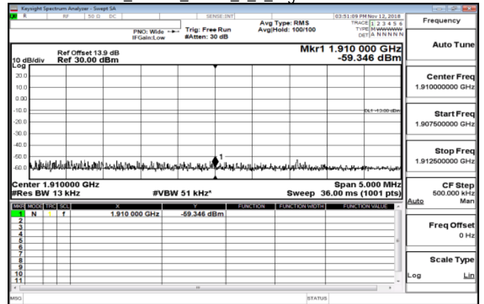
Band2_20MHz_QPSK_6_0_HighCH19100-1900
