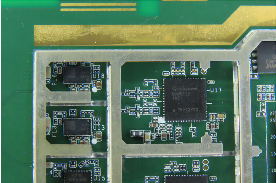
(51) EUT Photo
