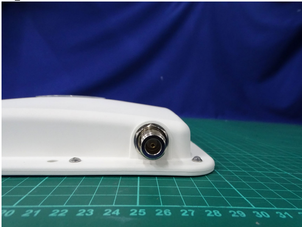
(24) EUT Photo_ Antenna: MOXA / ANT-WDB-PNF-1011
