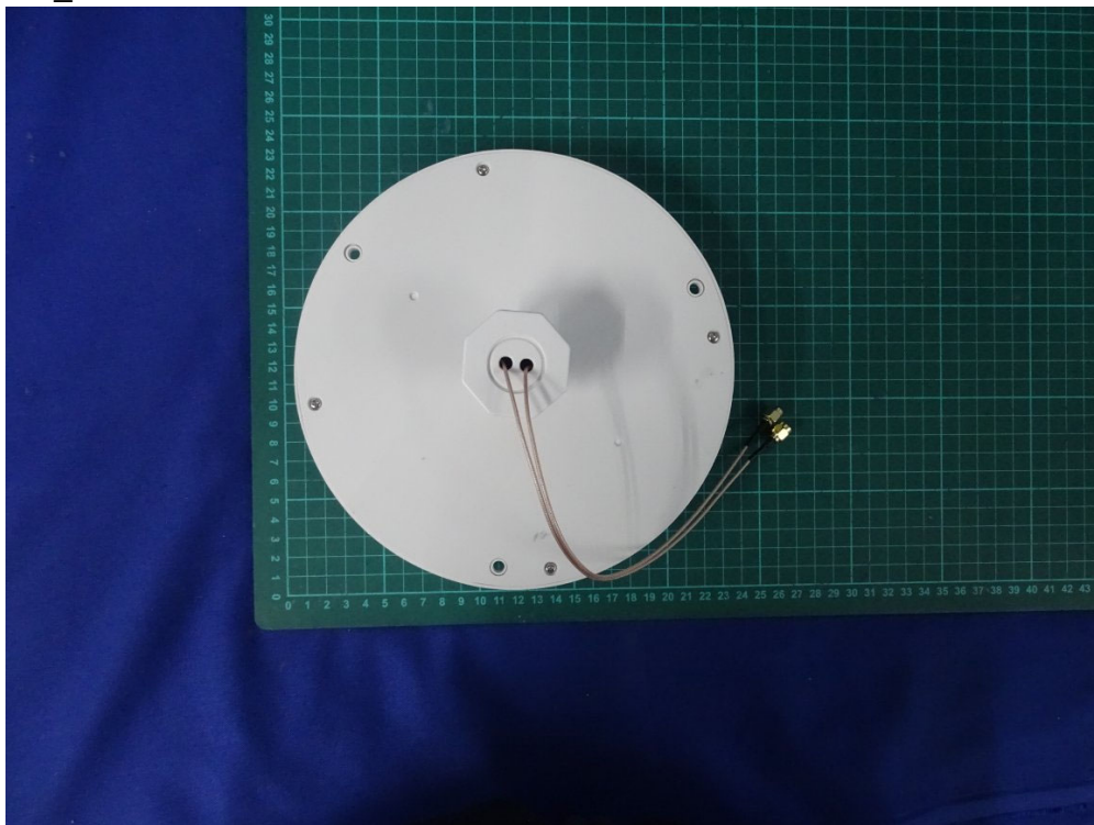
(14) EUT Photo_ Antenna: MOXA / MAT-WDB-CA-RM-2-0205
