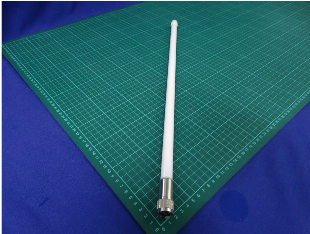
(25) EUT Photo_ Antenna: MOXA / ANT-WDB-ONM-0707
