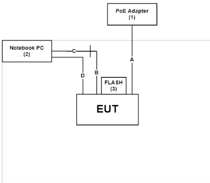
Connection Diagram
