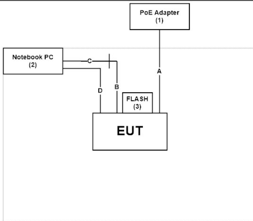
Connection Diagram
