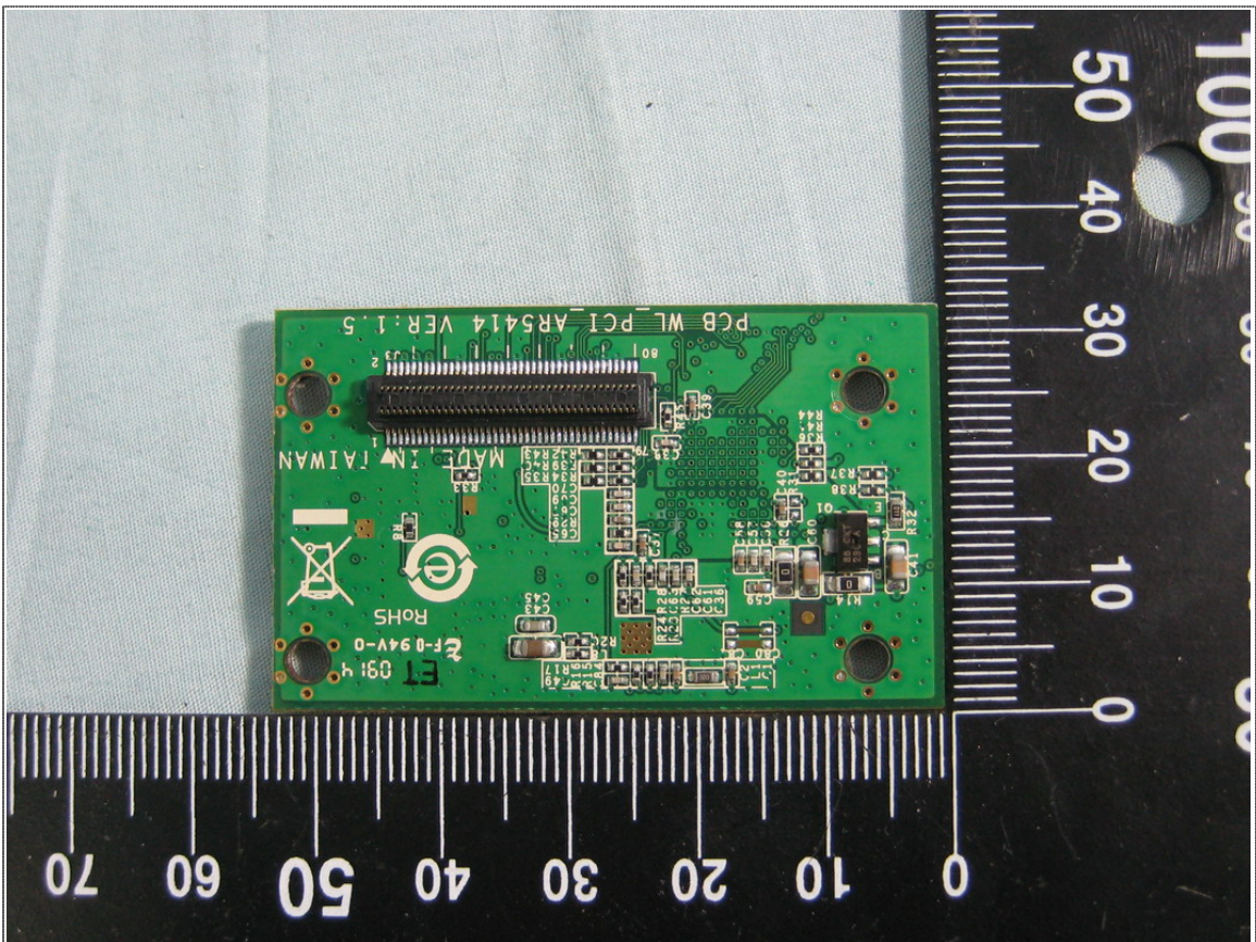
Rear View of WLAN Board (Module B)
