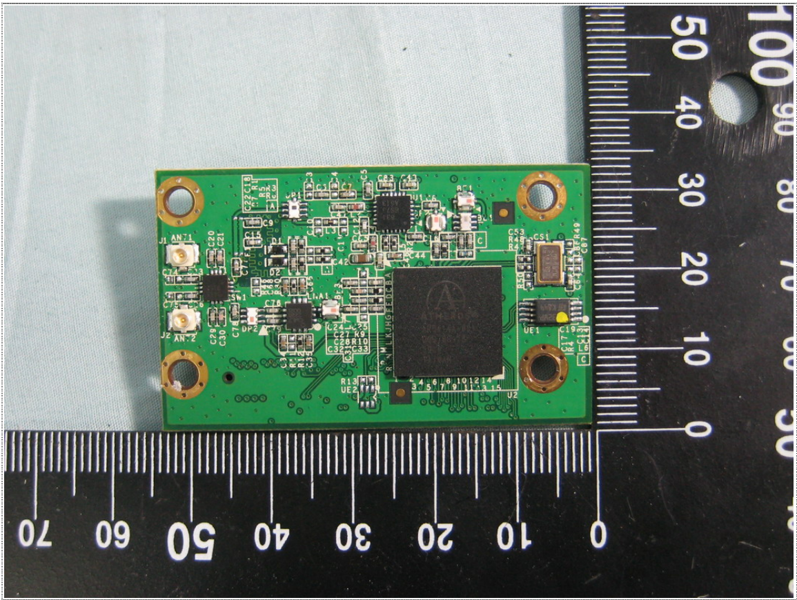
Front View of WLAN Board (Module B)
