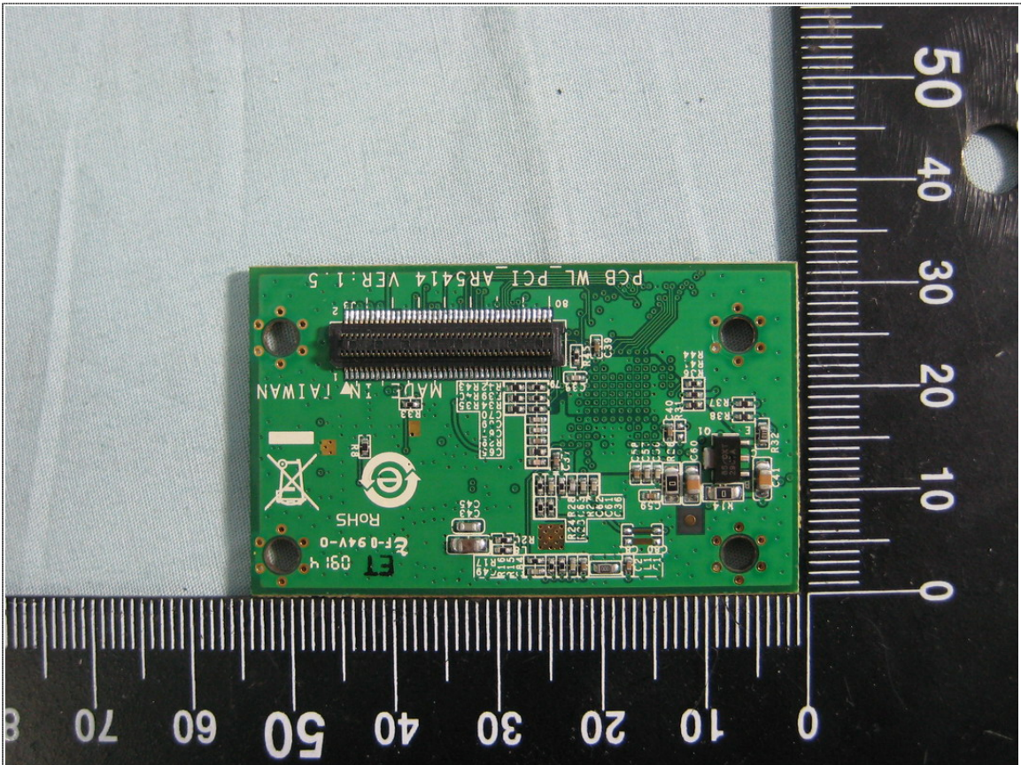
Rear View of WLAN Board (Module A)
