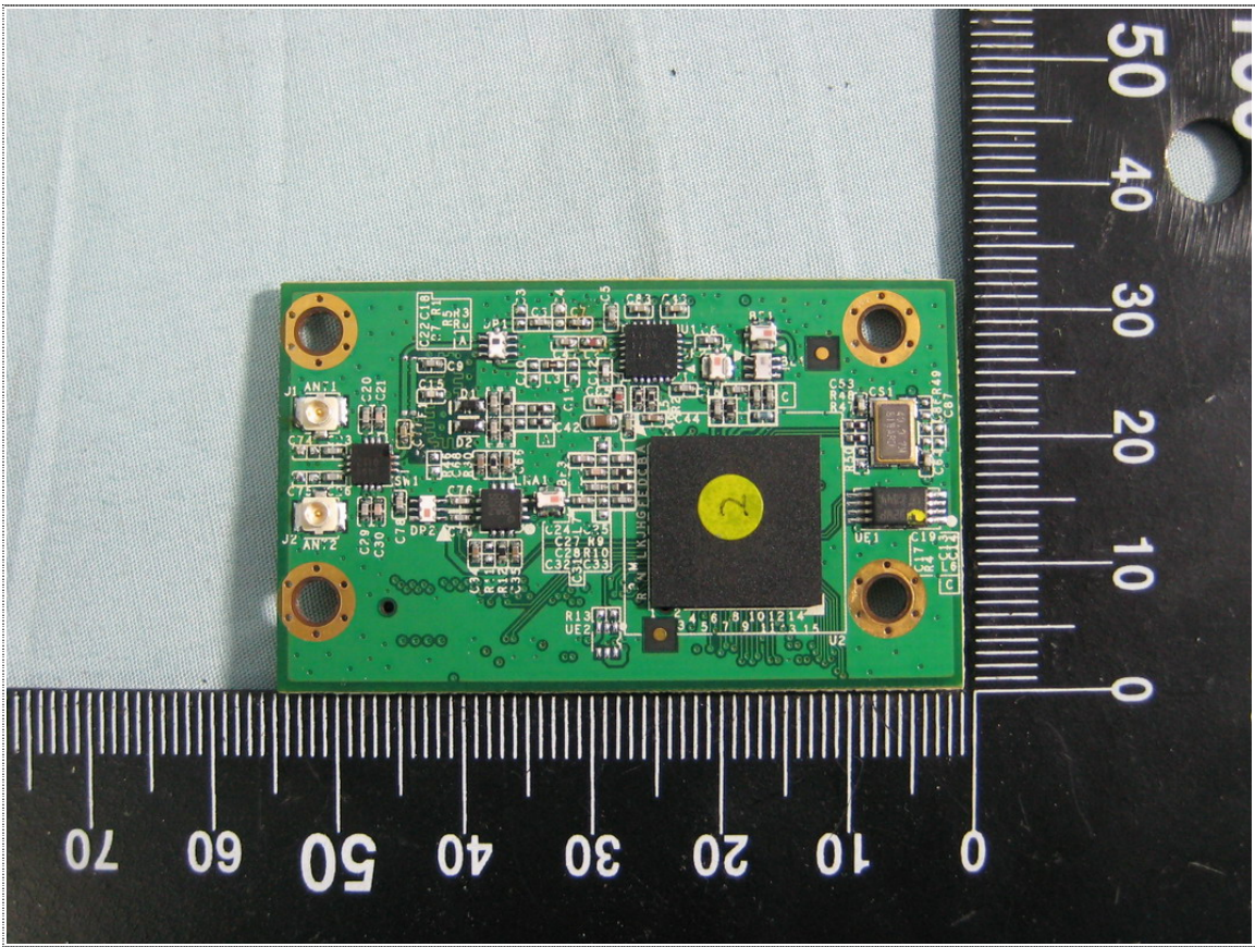
Front View of WLAN Board (Module A)
