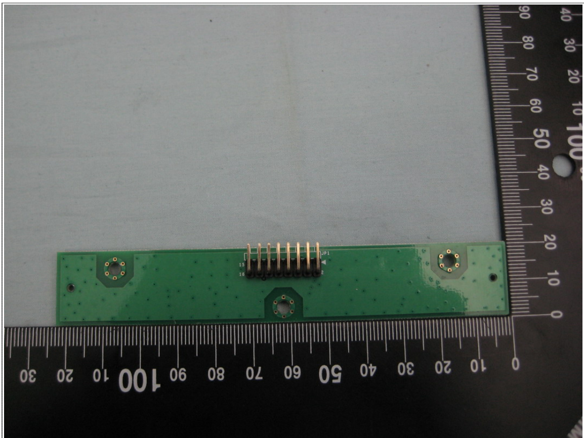
Rear View of LED Board
