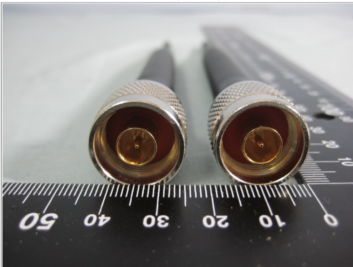
Antenna Connector (WSS007)
