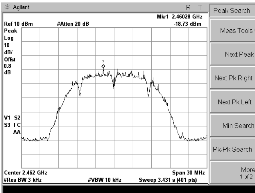
802.11g power density
