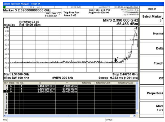
Channel 0 / 2405 MHz
