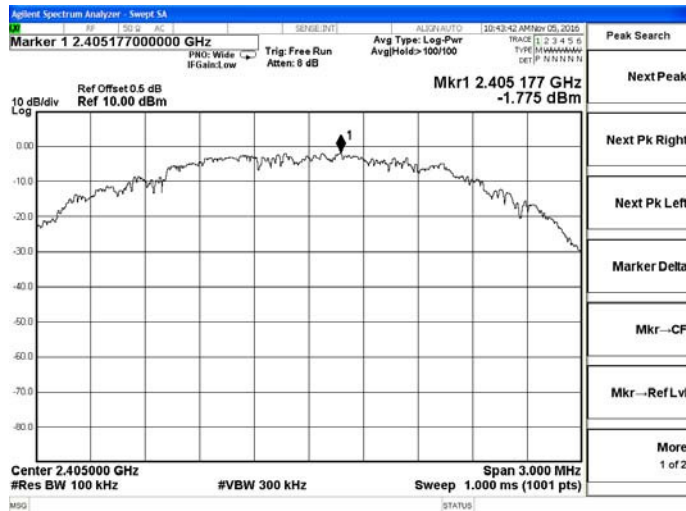
Channel 0 / 2405 MHz
