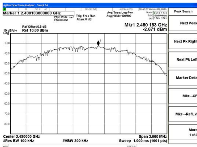
Channel 15 / 2480 MHz
