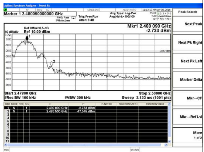
Channel 15 / 2480 MHz
