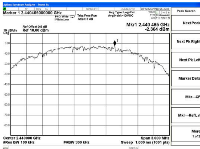
Channel 7 / 2440 MHz
