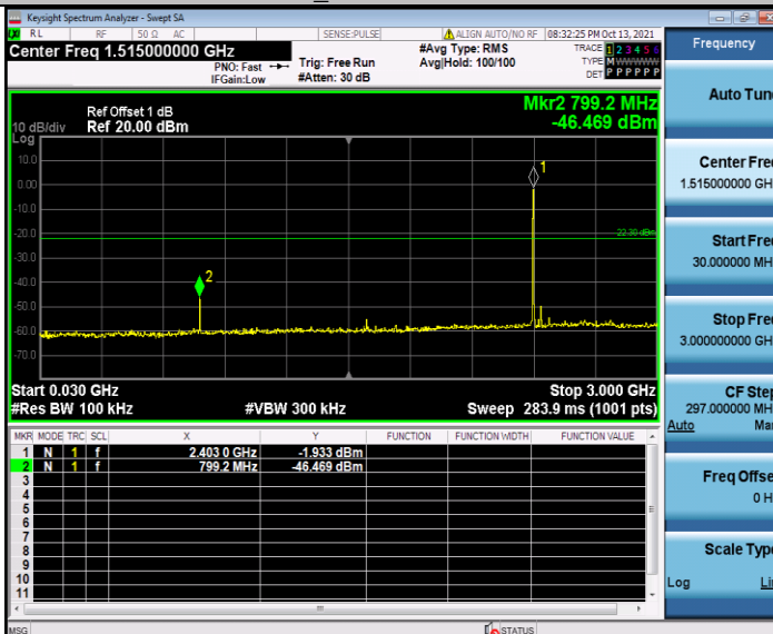
BLE_2402_30-3000
