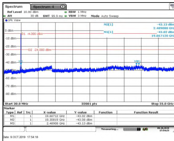
Figure 7.5.1.2-3: HCH – 30MHz–25GHz
