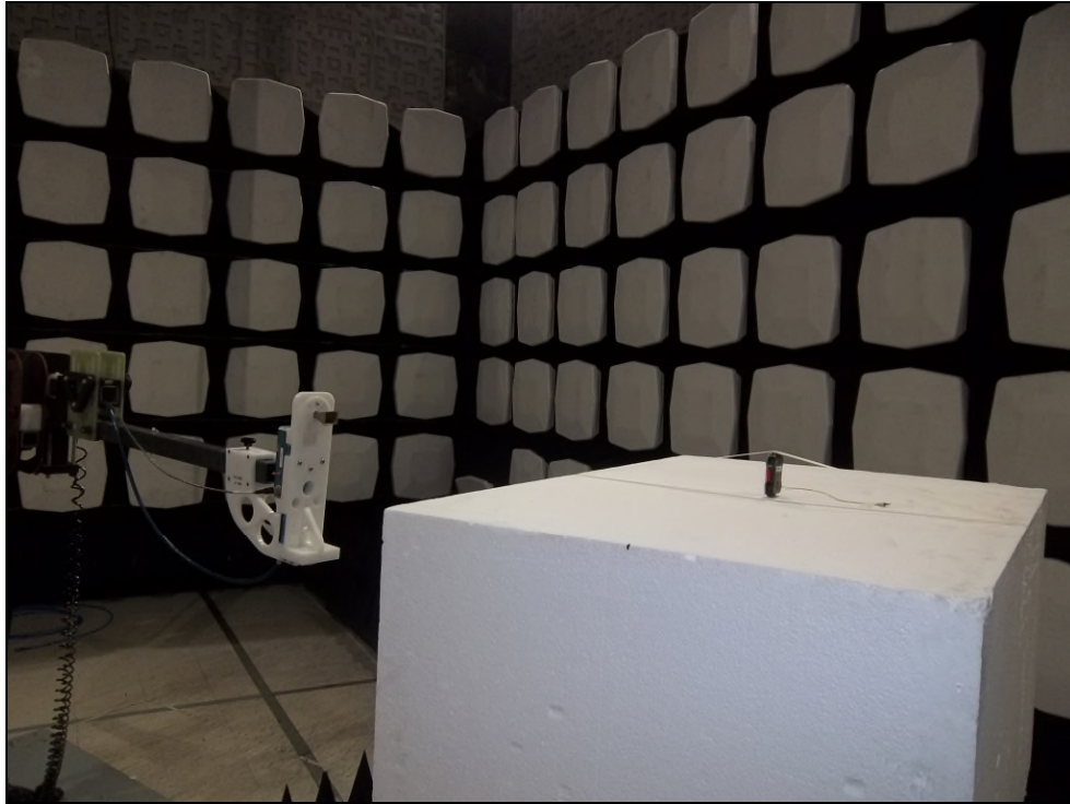
Figure 7: Equipment Under Test – Radiated Emissions 18GHz – 26GHz
