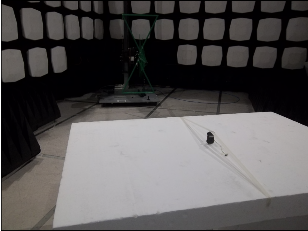
Figure 5: Equipment Under Test – Radiated Emissions 30MHz – 1GHz
