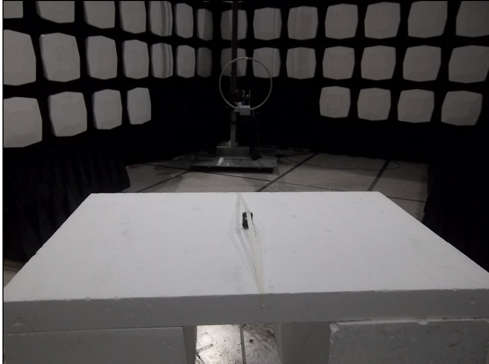
Figure 4: Equipment Under Test – Radiated Emissions 9kHz – 30MHz
