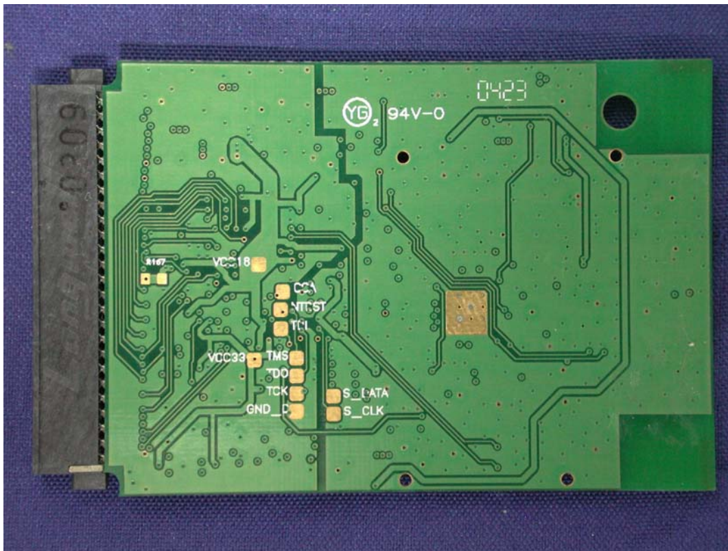
(11) EUT Photo
