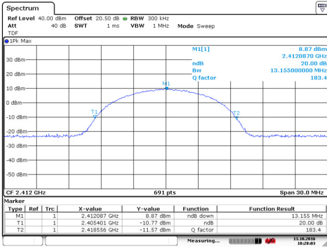
Figure 8.2-4: 20 dB bandwidth on 802.11b, sample plot
