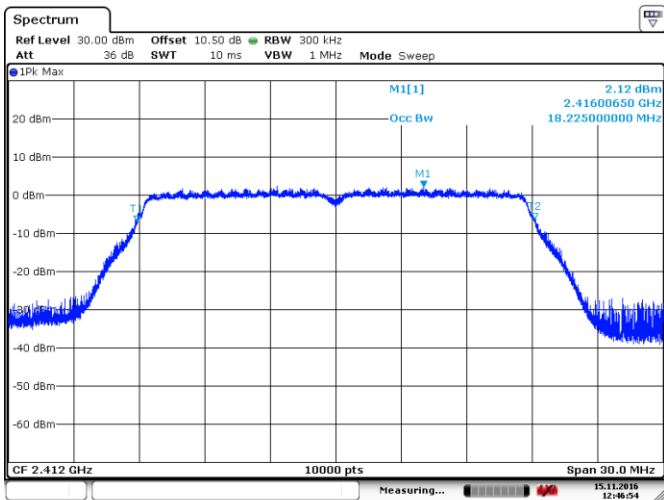
Figure 8.2-9: 99% bandwidth on 802.11n, sample plot
