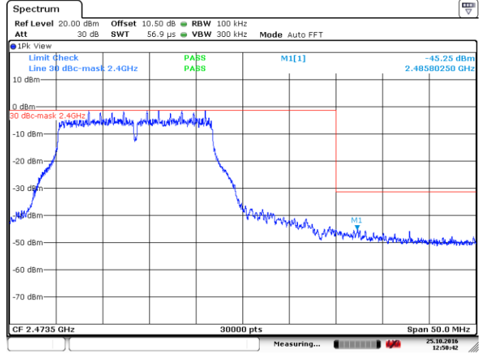
Figure 8.4-14: Conducted spurious emissions Upper band edge for 802.11g, (TX 2462 MHz)
