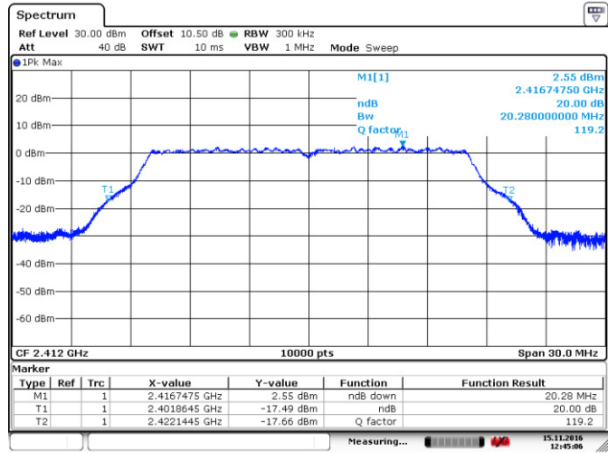
Figure 8.2-5: 20 dB bandwidth on 802.11g, sample plot
