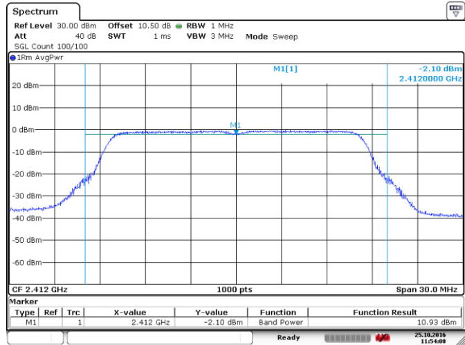
Figure 8.3-2: Conducted output power on 802.11g, sample plot
