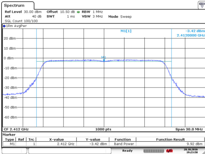
Figure 8.3-3: Conducted output power on 802.11n, sample plot
