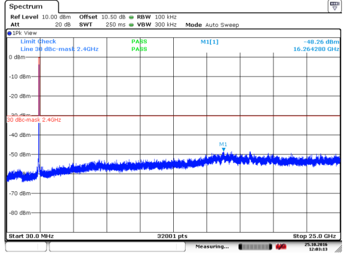
Figure 8.4-2: Conducted spurious emissions for 802.11g (TX 2412 MHz)
