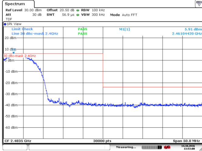
Figure 8.4-13: Conducted spurious emissions Upper band edge for 802.11b, (TX 2462 MHz)
