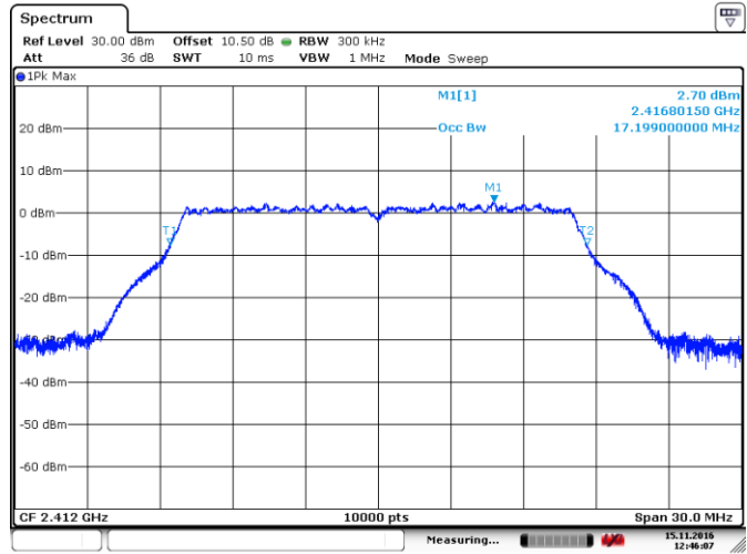
Figure 8.2-8: 99% bandwidth on 802.11g, sample plot
