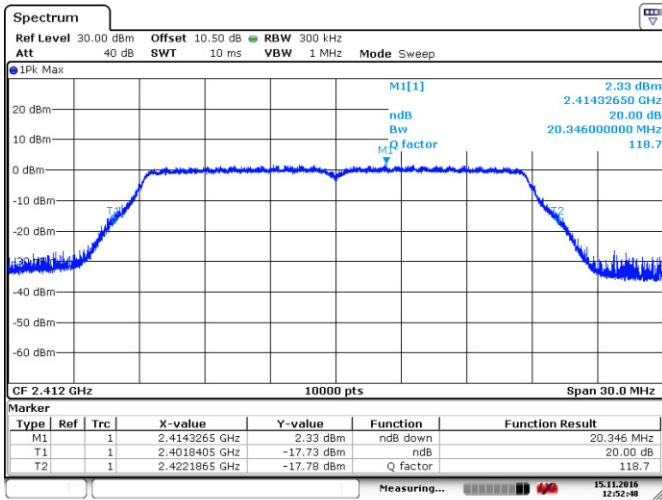
Figure 8.2-6: 20 dB bandwidth on 802.11n, sample
