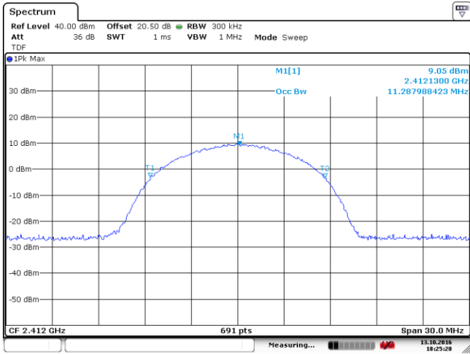
Figure 8.2-7: 99% bandwidth on 802.11b, sample plot
