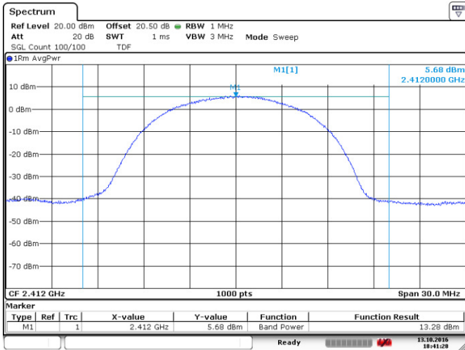
Figure 8.3-1: Conducted output power on 802.11b, sample plot
