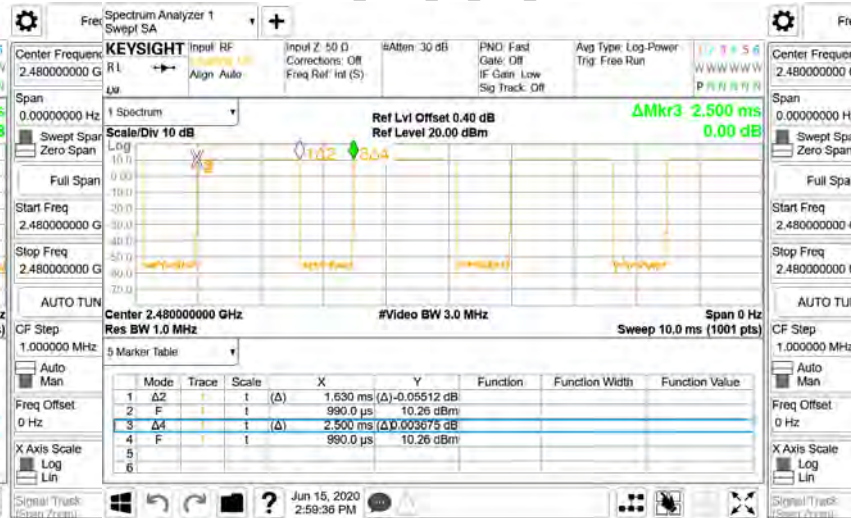
Dwell Time_GFSK_1M_DH3_2480MHz
