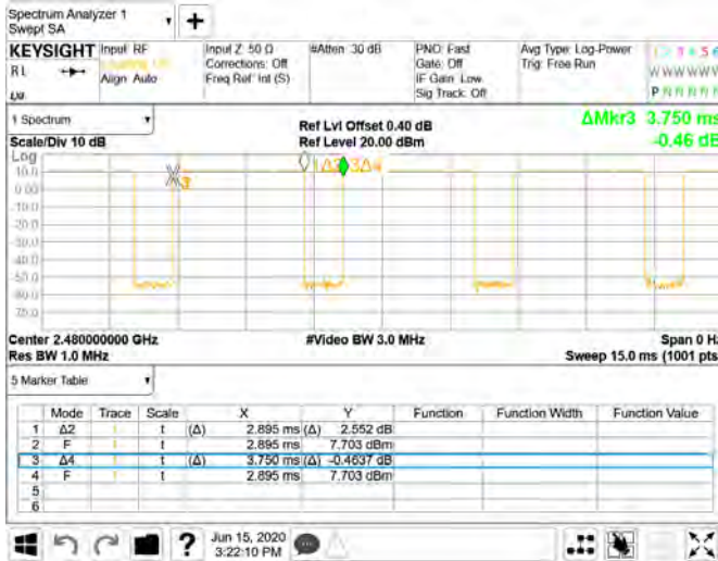
Dwell Time_GFSK_1M_DH5_2480MHz
