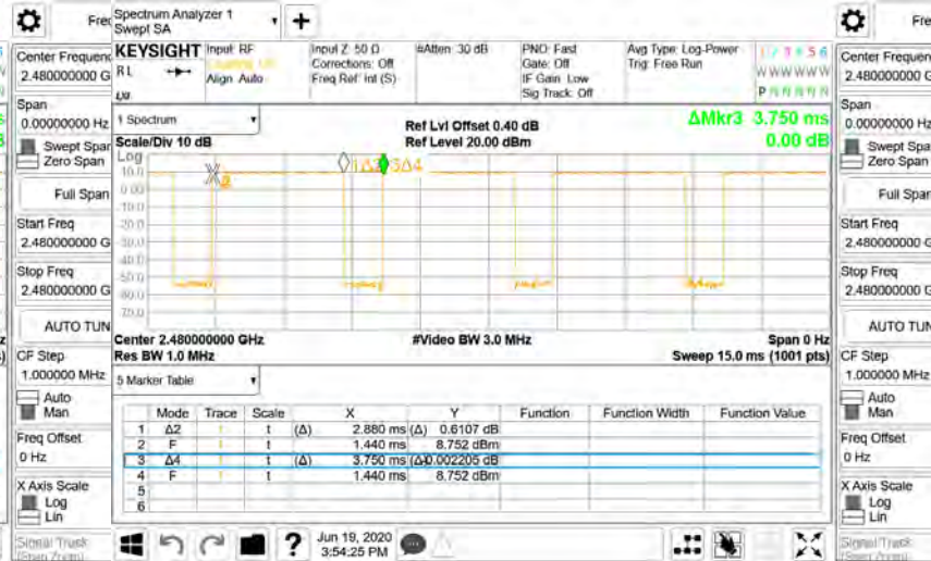
Dwell Time_π/4QPSK_2M_2480MHz
