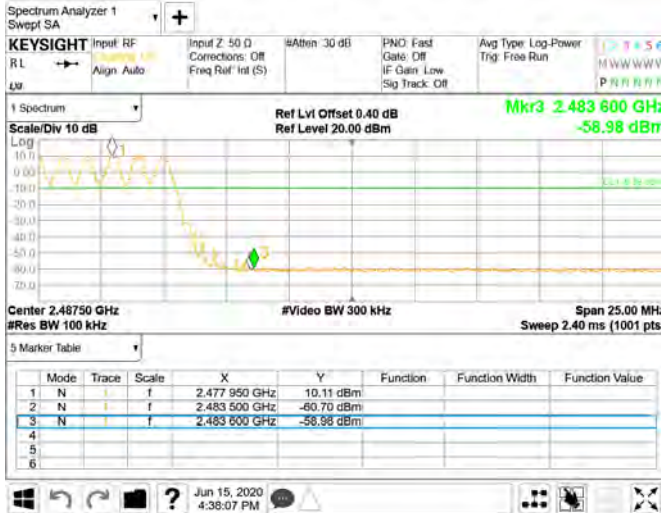
Hopping Band Edge_GFSK_1M_DH5_2480MHz
