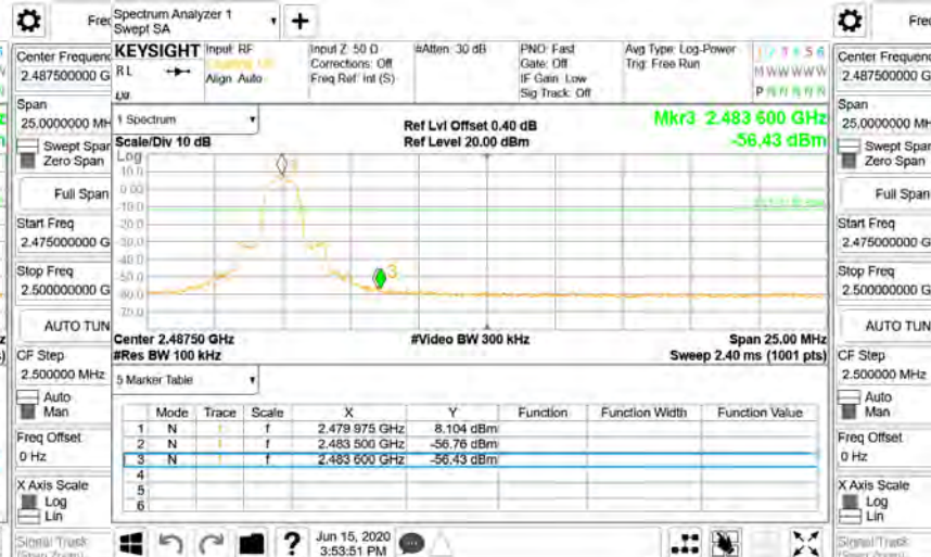
Band Edge_8DPSK_3M_DH5_2480MHz
