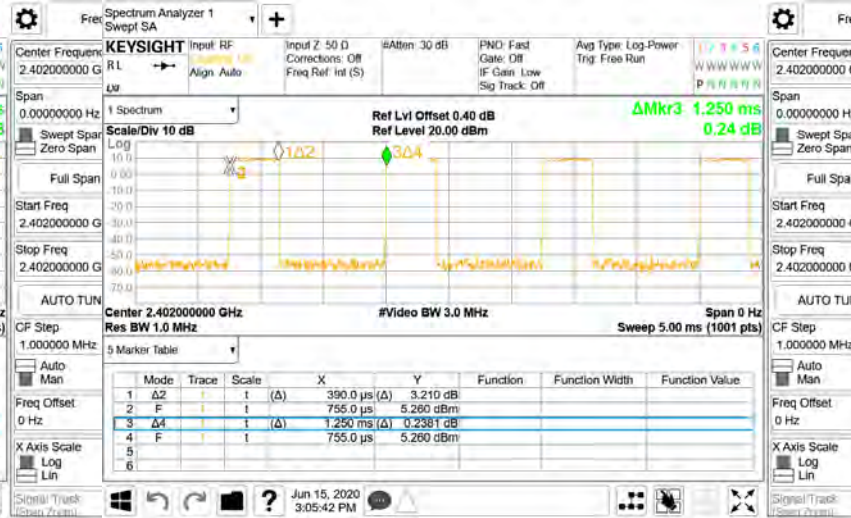
Dwell Time_π/4QPSK_2M_2402MHz
