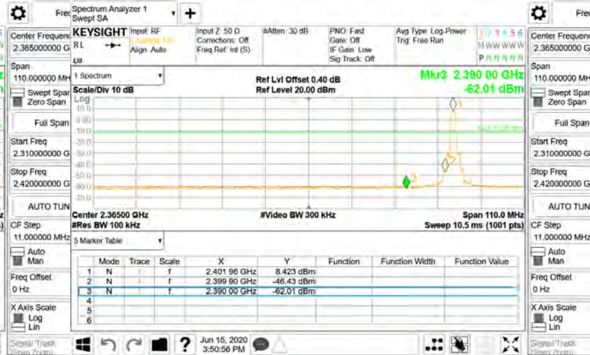
Band Edge_8DPSK_3M_DH5_2402MHz
