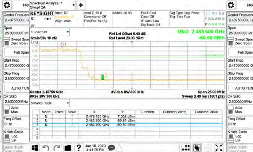
Hopping Band Edge_8DPSK_3M_DH5_2480MHz
