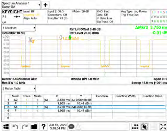
Dwell Time_GFSK_1M_DH5_2402MHz
