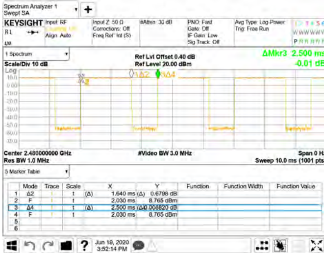
Dwell Time_π/4QPSK_2M_2480MHz
