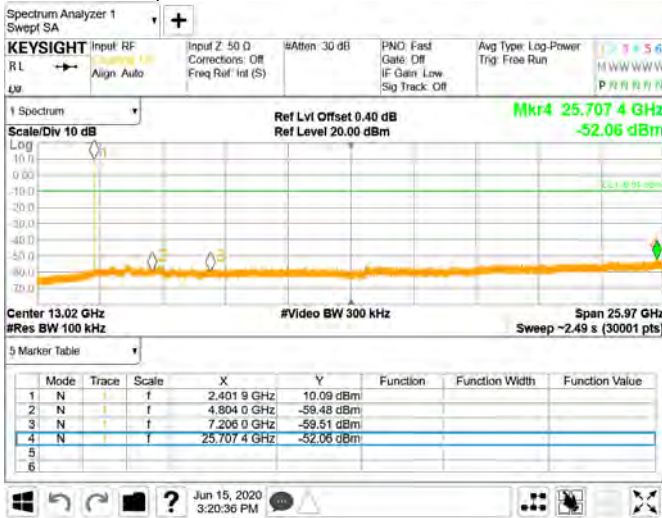
Spurious Emission_GFSK_1M_DH5_2402MHz
