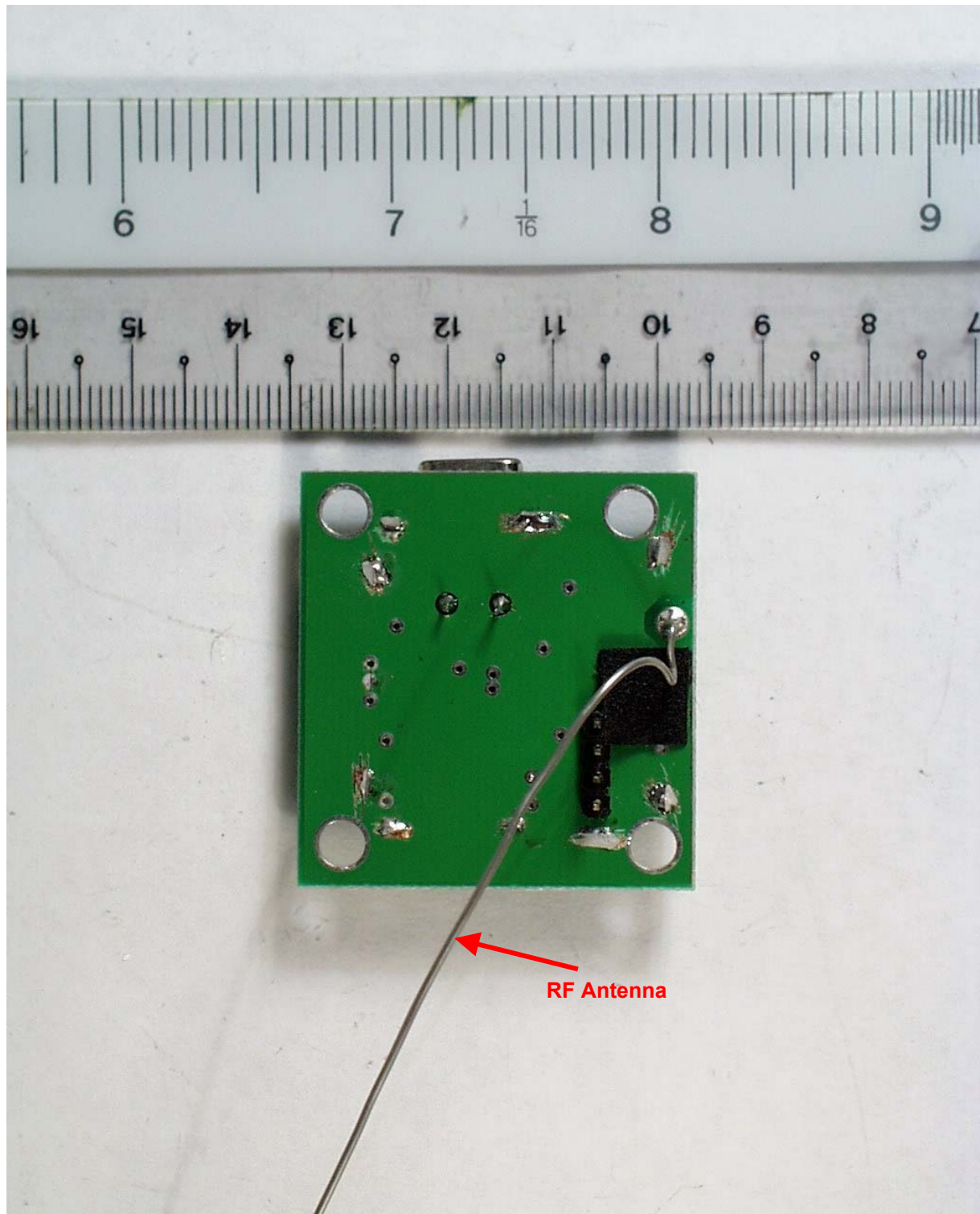
Trace Side (RF Module)– RF Remote Controller
