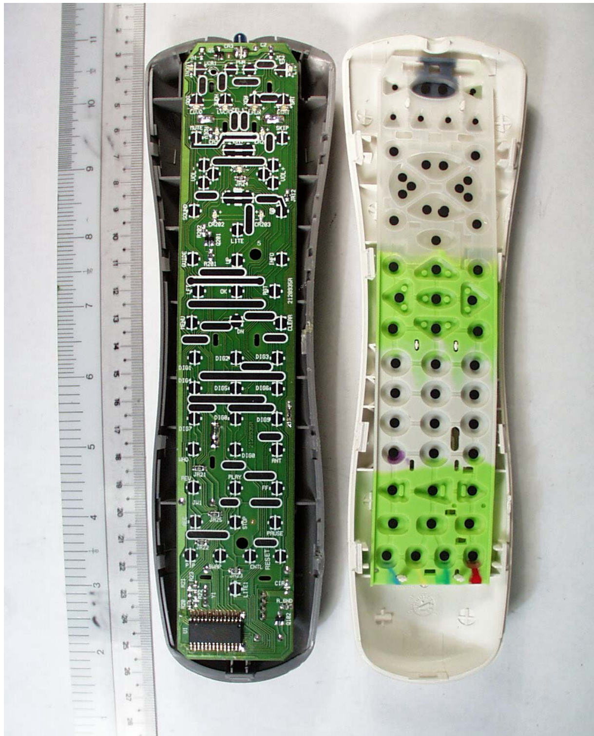
Overall Internal View (Main PCB) – RF Remote Controller
