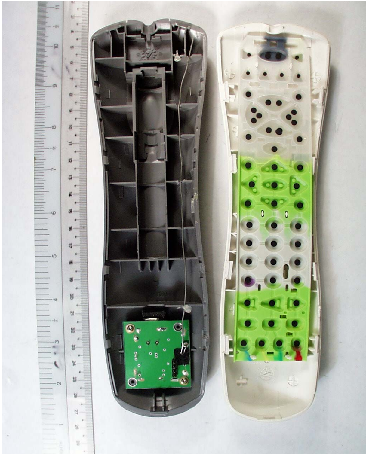
Overall Internal View (RF Module) – RF Remote Controller
