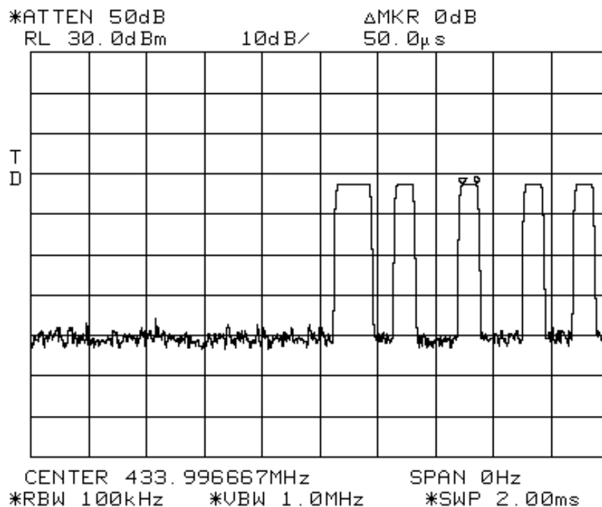
Plot 3 - Pulse Width 1
