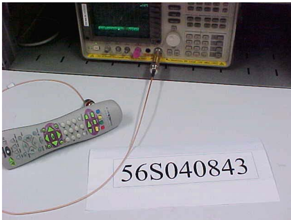
Duty Cycle Factor Measurement Test Setup
