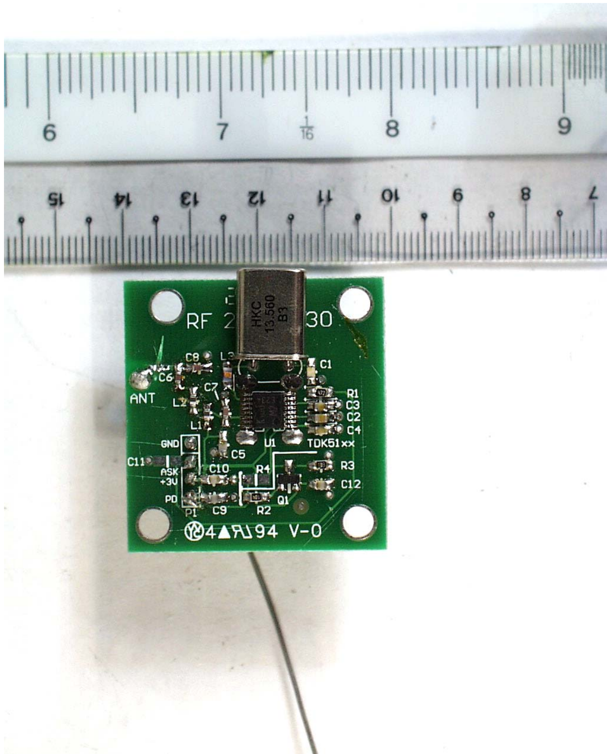
Component Side (RF Module)– RF Remote Controller
