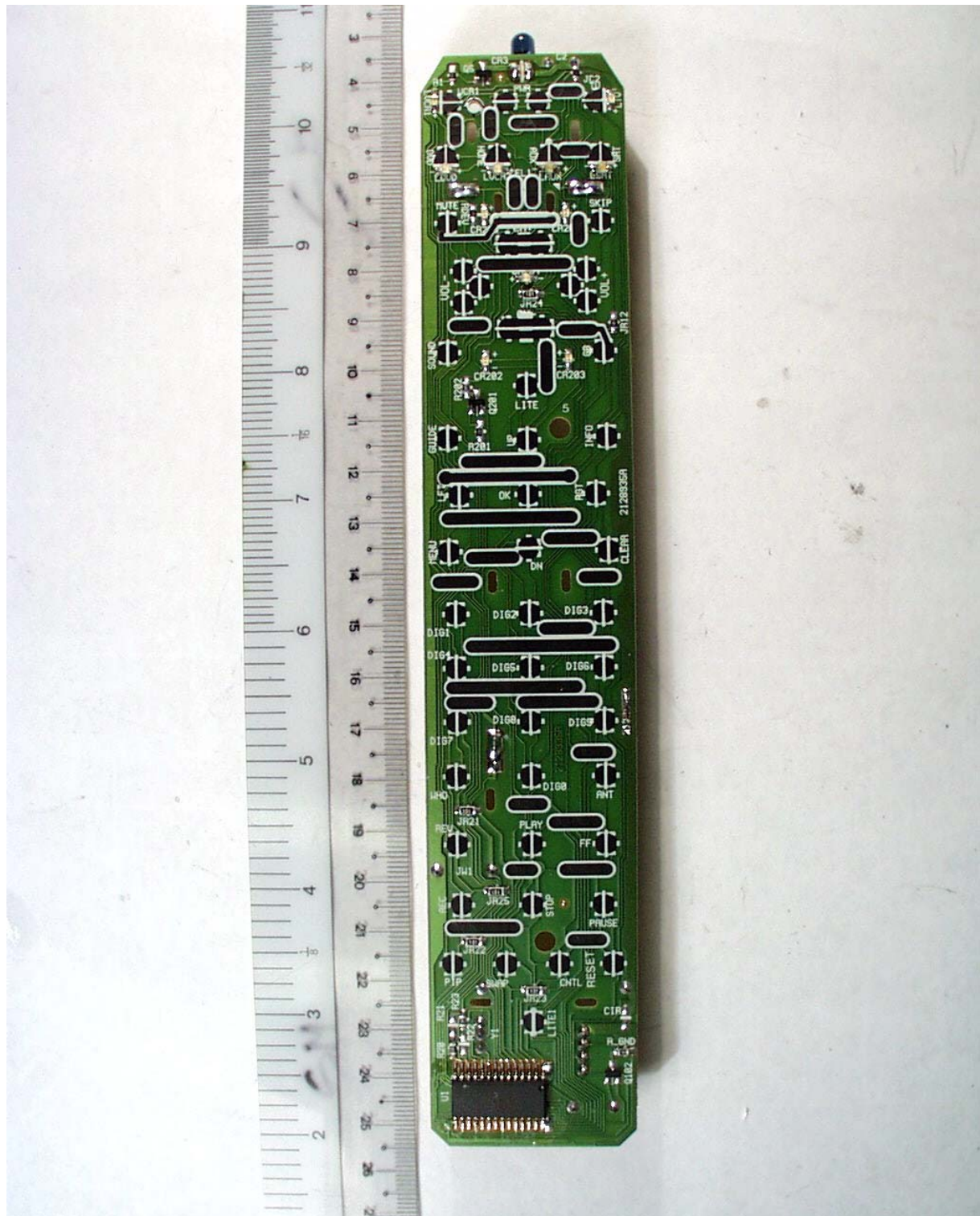
Trace Side (Main PCB)– RF Remote Controller
