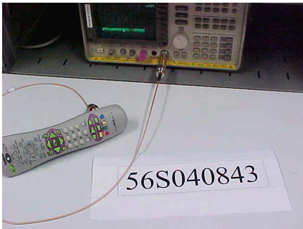
20dB Bandwidth Measurement Test Setup
