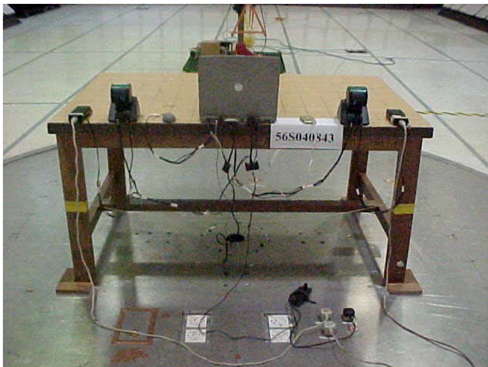
Radiated Emission Setup (Rear View)
