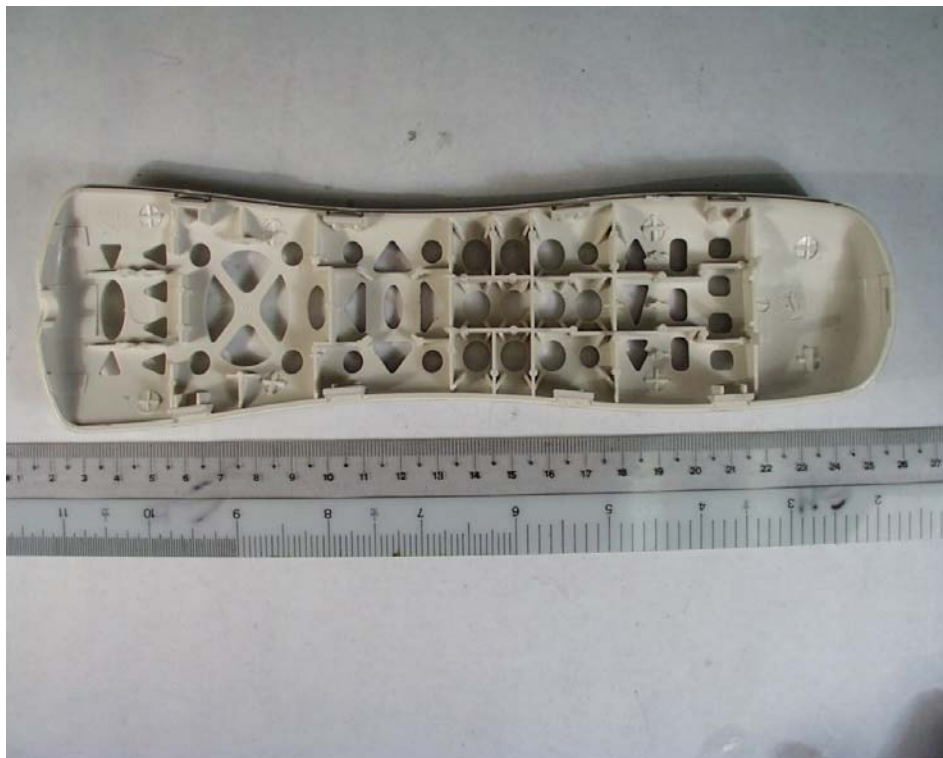
Top Housing Internal View – RF Remote Controller
