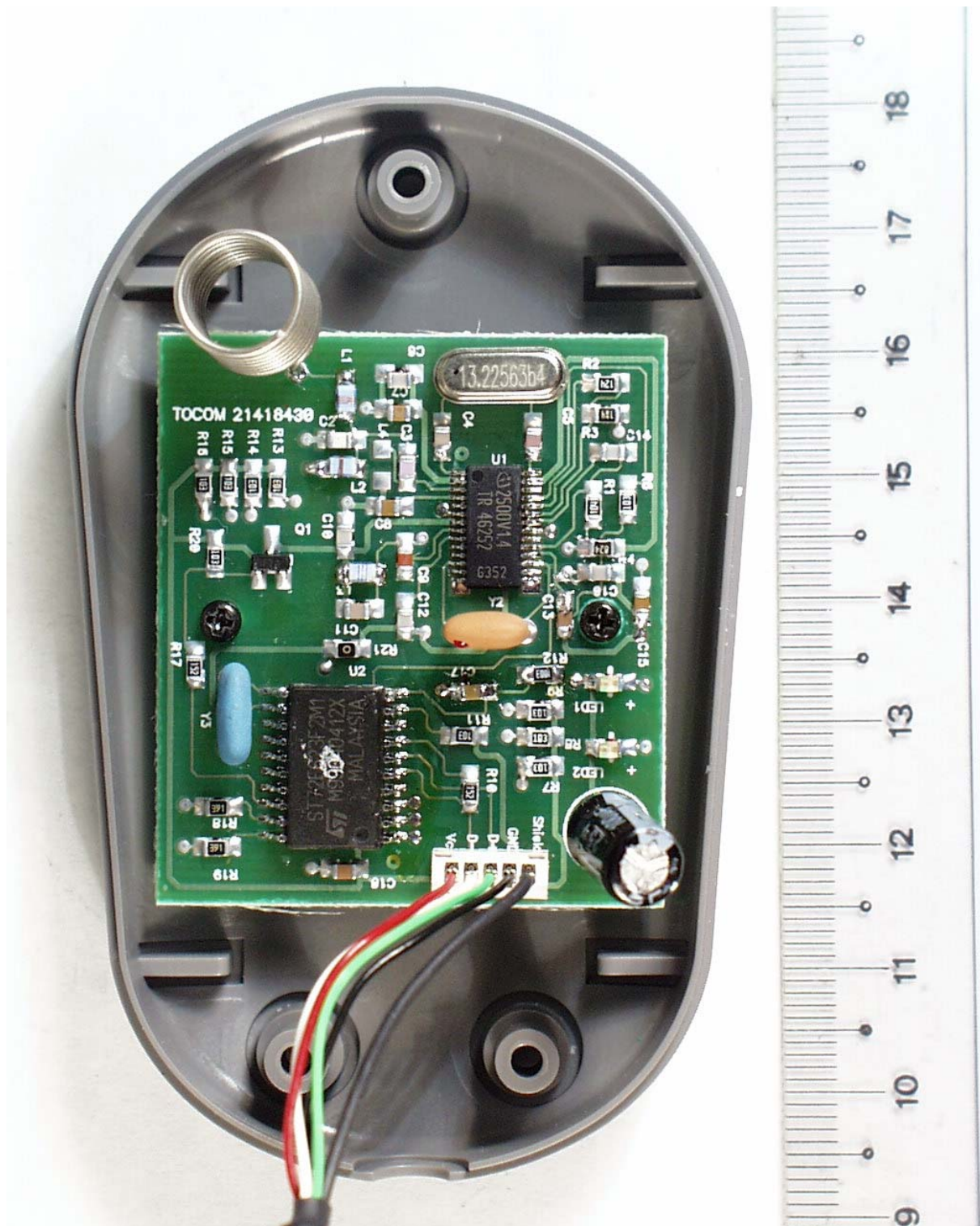
Overall Internal View – RF Dongle
