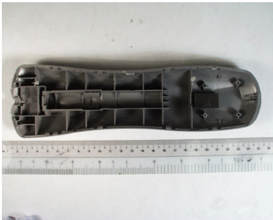
Bottom Housing Internal View– RF Remote Controller
