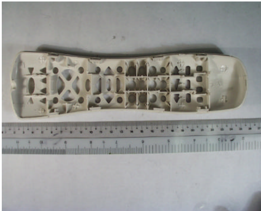
Top Housing Internal View – RF Remote Controller
