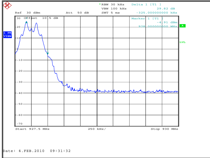
Figure 7.3.1.2-2: Upper Band-edge
