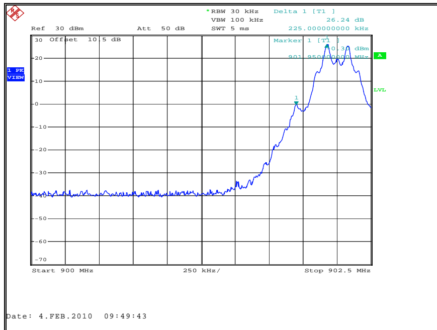
Figure 7.3.1.2-1: Lower Band-edge
