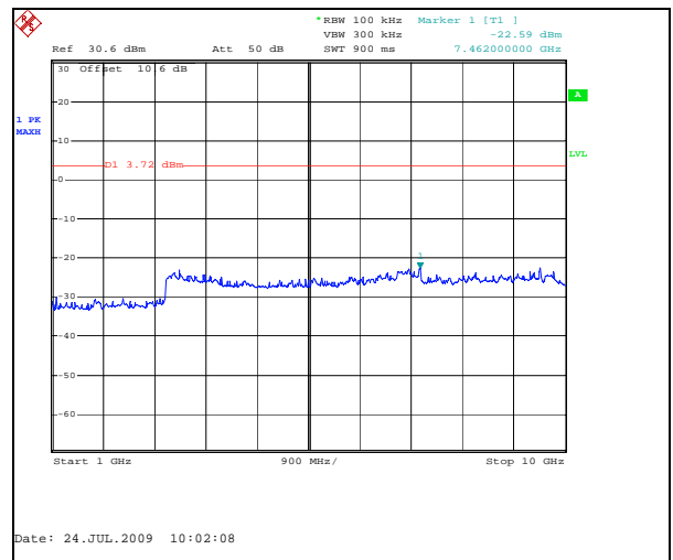
Figure 7.6.2.2-4: 1 GHz – 10 GHz – Mid Channel
