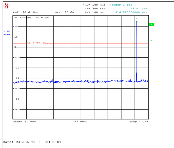
Figure 7.6.2.2-3: 30 MHz – 1 GHz –Mid Channel
