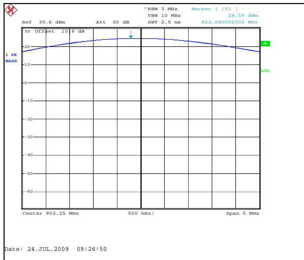
Figure 7.4.2-1: Output power – Low Channel
