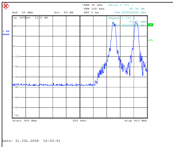
Figure 7.6.1-1: Lower Band-edge – Hopping Enabled
