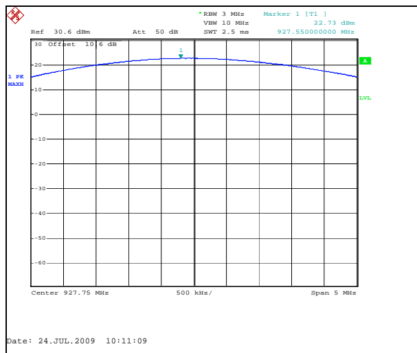
Figure 7.4.2-3: Output power – High Channel
