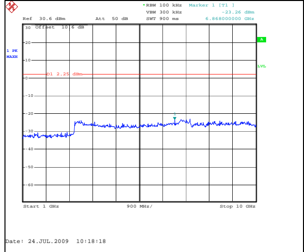
Figure 7.6.2.2-6: 1 GHz – 10 GHz –High Channel
