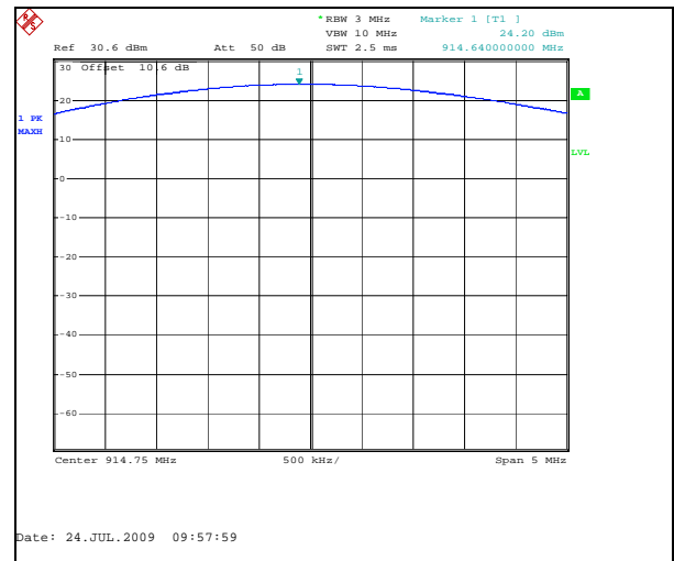
Figure 7.4.2-2: Output power – Mid Channel
