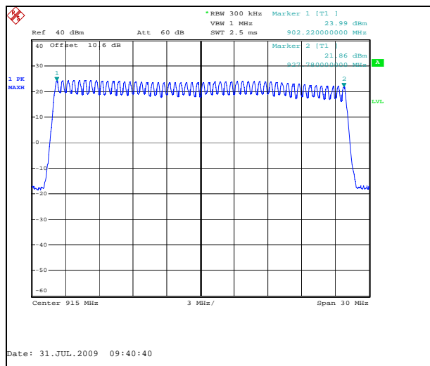
Figure 7.5.2-1: Number of Hopping Channels
