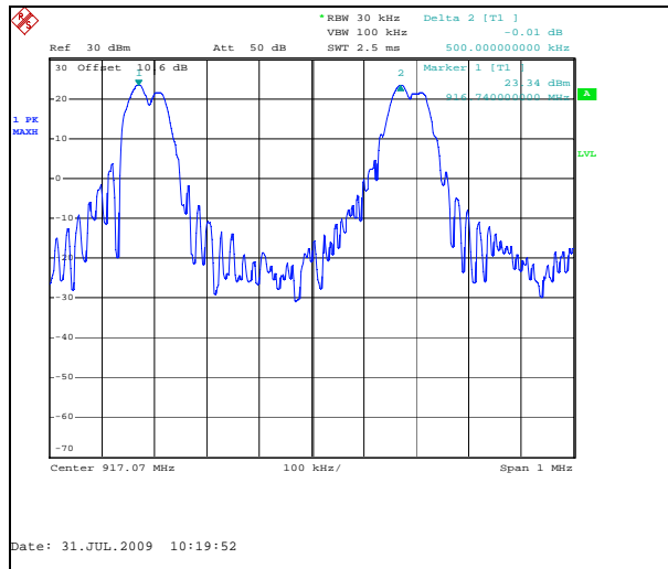
Figure 7.5.1.2-1: Carrier Frequency Separation
