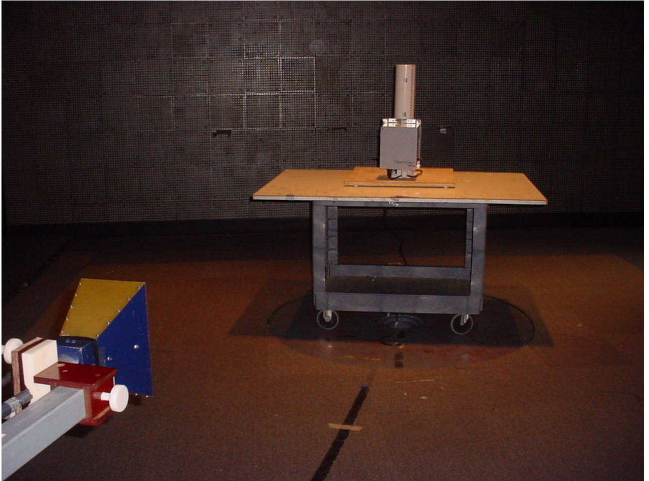
Figure 1: Radiated Emissions – View 1
