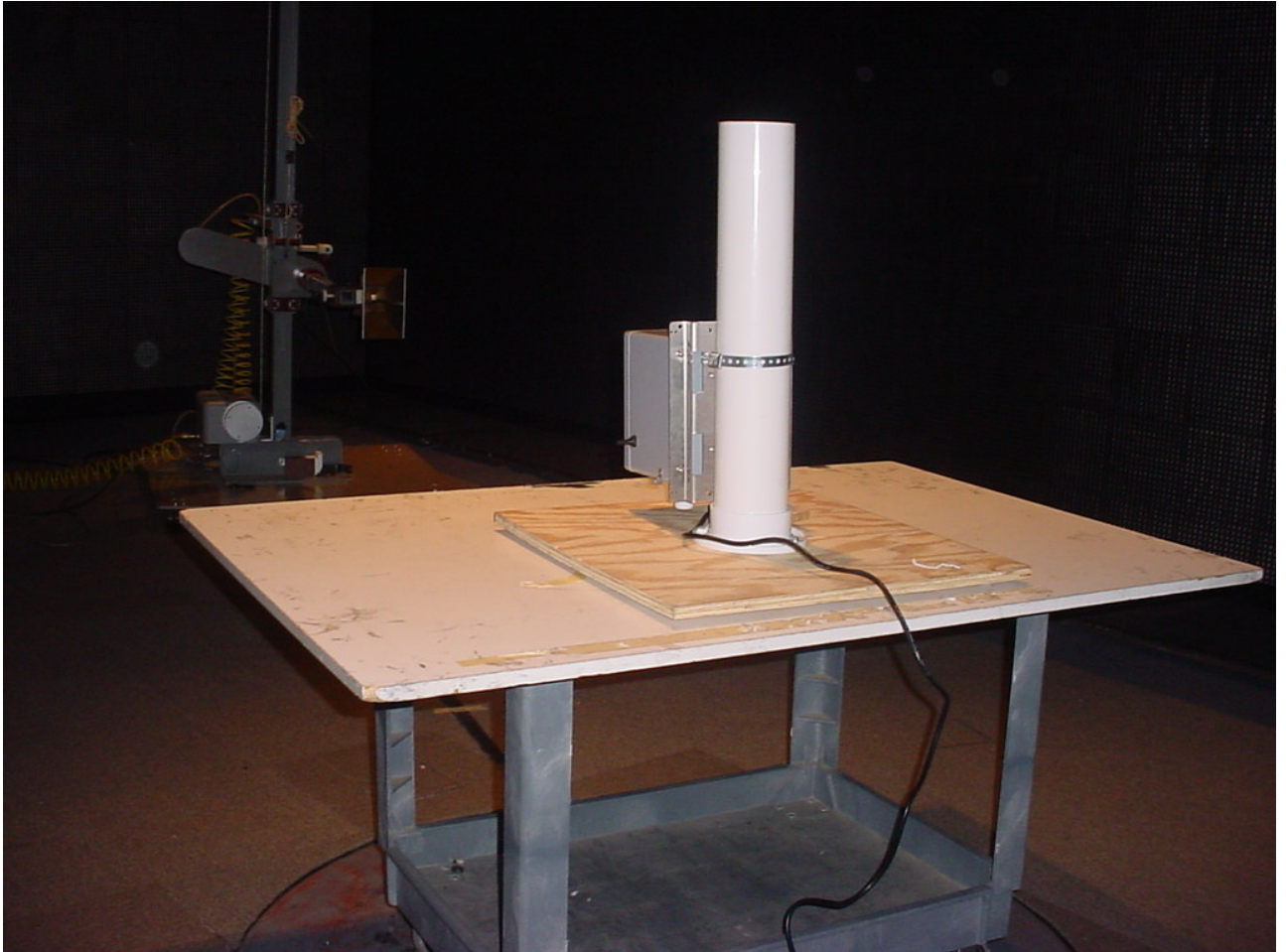
Figure 2: Radiated Emissions – View 2
