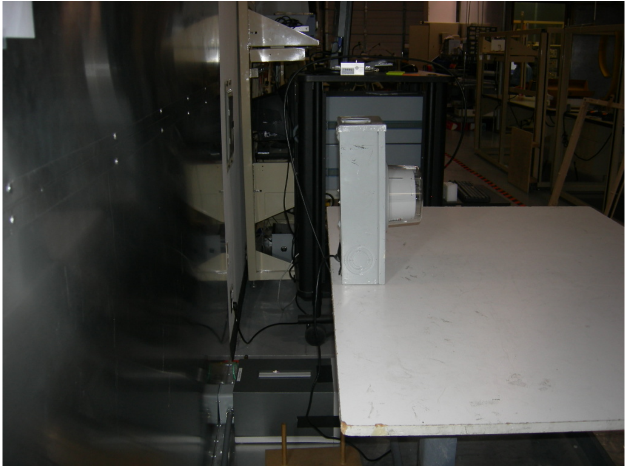
Figure 8: 2S Meter – AC Power Line Conducted Emissions
