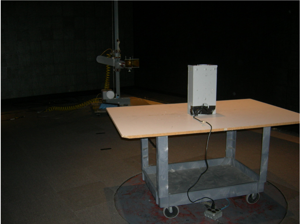
Figure 2: 1S Meter – Radiated Emissions
