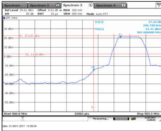
Figure 7.6.1.2-4: Lower Band-edge
