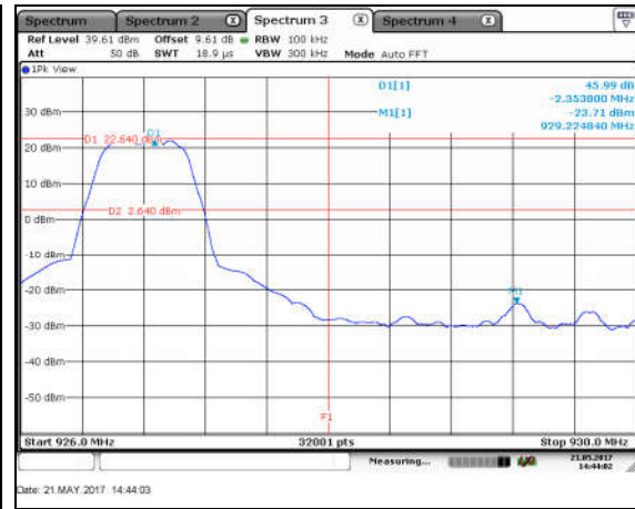
Figure 7.6.1.2-5: Upper Band-edge
