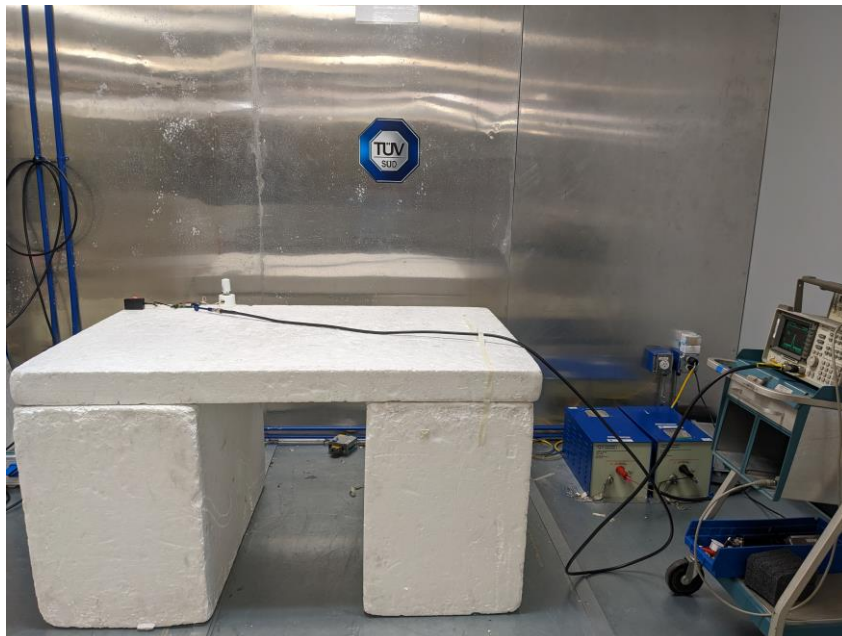
Figure 4 – Test Set up – Power Line Conducted Emissions
