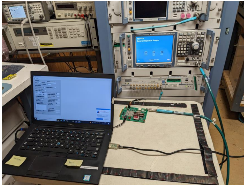
Figure 5 – Test Set up – Antenna Port Measurement
