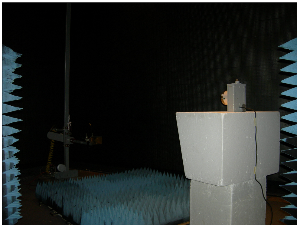
Figure 4: Radiated Emissions – 2S Meter Form
