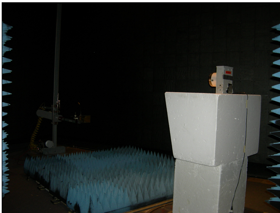
Figure 6: Radiated Emissions – 12S Meter Form
