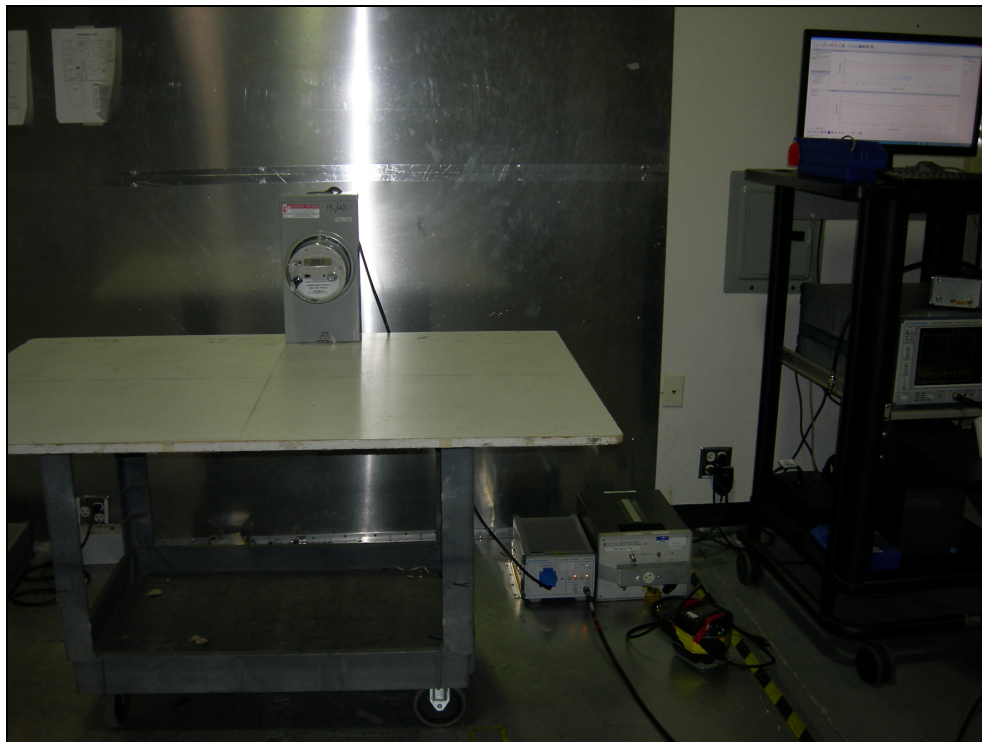
Figure 7: Conducted Emissions – 1S Meter Form
