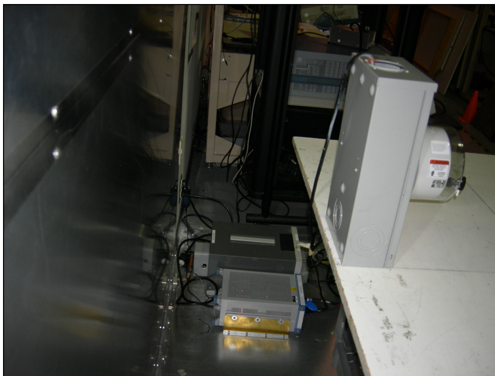
Figure 8: Conducted Emissions – 1S Meter Form
