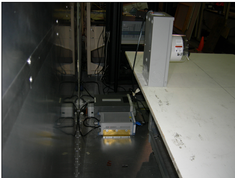
Figure 10: Conducted Emissions – 2S Meter Form
