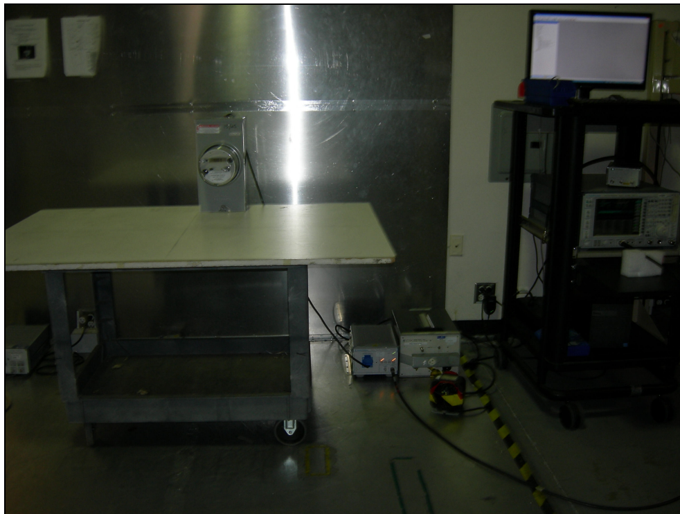
Figure 9: Conducted Emissions – 2S Meter Form
