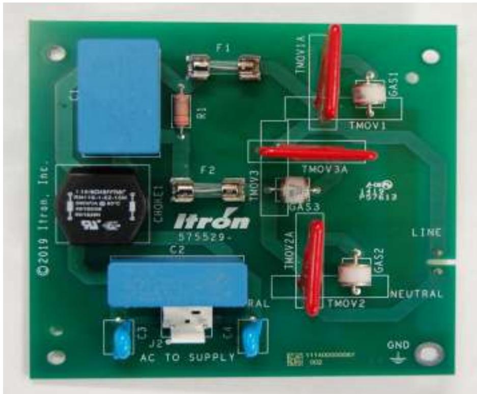
Protection/filter board, top
