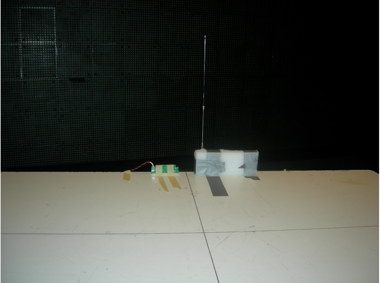
Figure 3: Radiated Emissions – Intentional
