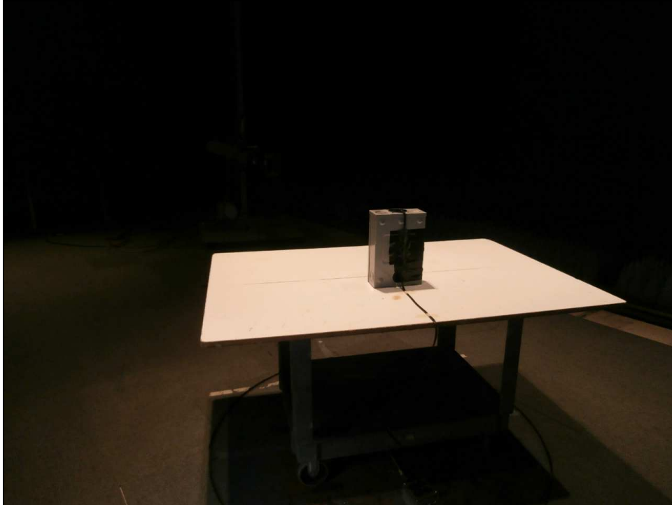
Figure 6: Radiated Emissions – Installed in 12S Meter
