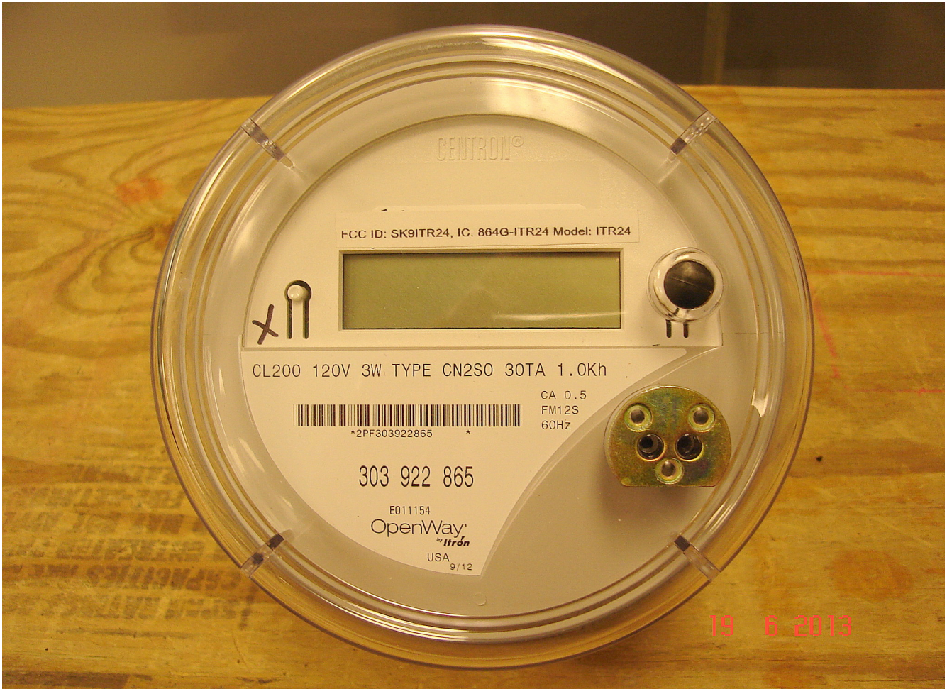
Figure 2 Itron ITR24 module installed in electricity meter
