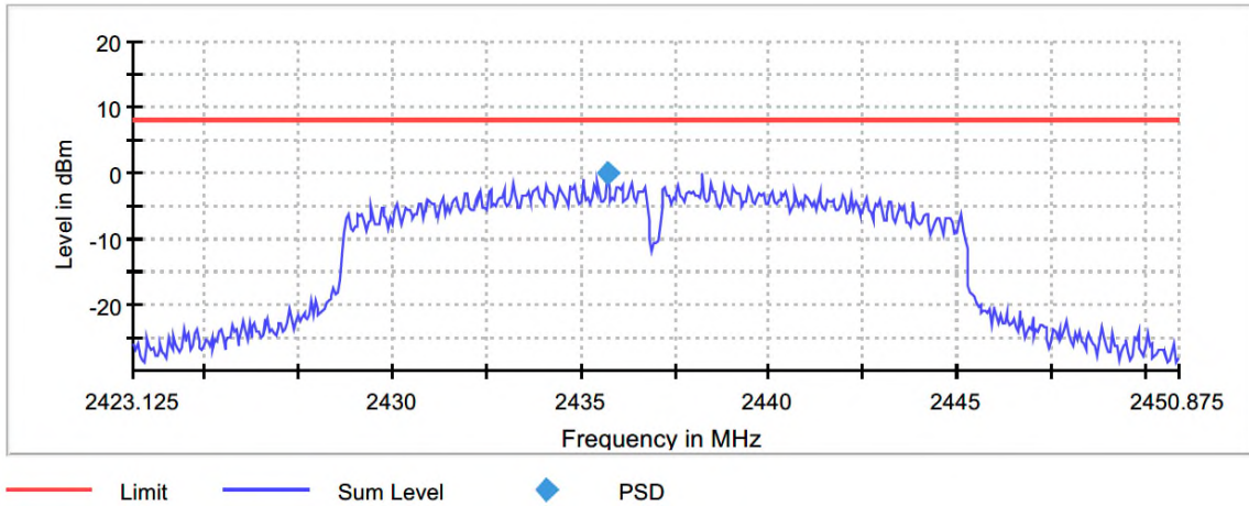
Figure 7.6.2-1: Sample PSD Plot
