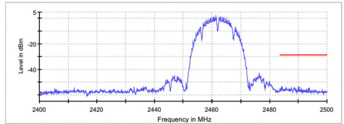
Figure 7.5.1.2-5: 802.11b – Upper Band-edge
