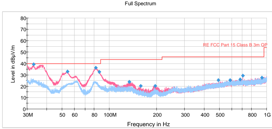
Note: Emissions above the noise floor are from the digital sections of the DUT and not associated with the radio. Figure A-3: 30MHz-1GHz
