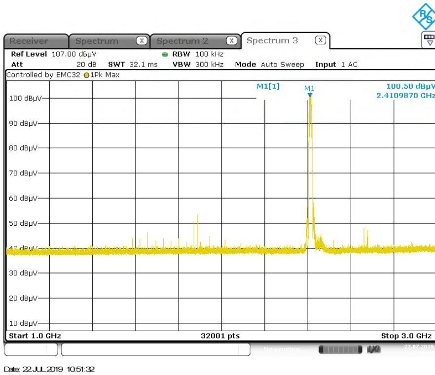
Note: Emissions above the noise floor are from the digital sections of the DUT and not associated with the radio. Figure A-4: 1GHz-3GHz
