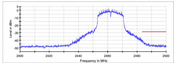
Figure 7.5.1.2-9: 802.11n20 – Upper Band-edge
