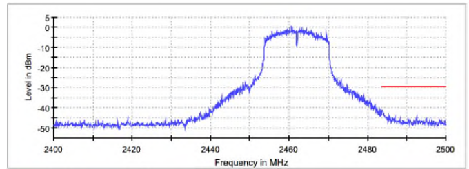
Figure 7.5.1.2-7: 802.11g – Upper Band-edge
