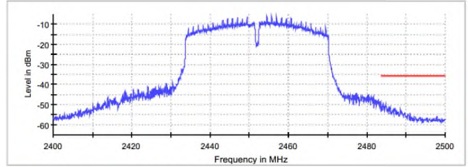
Figure 7.5.1.2-11: 802.11n40 – Upper Band-edge
