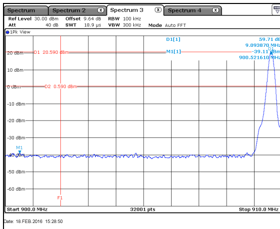
Figure 7.5.1.2-1: Lower Band-edge
