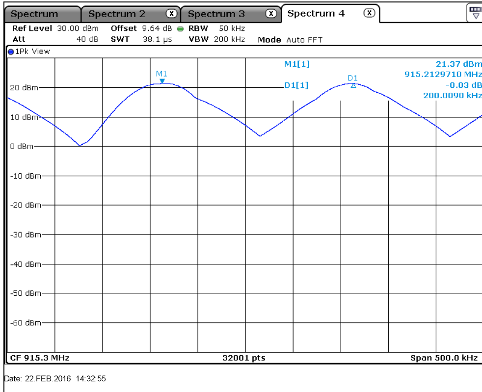
Figure 7.4.1.2-1: Channel Separation
