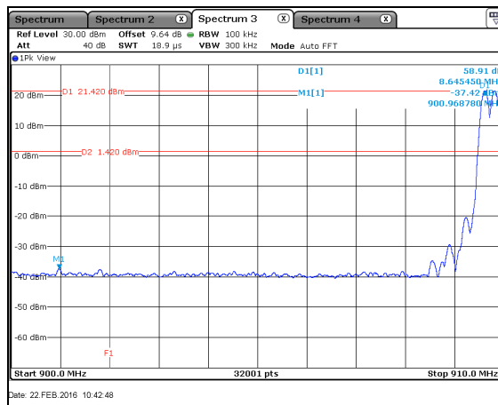
Figure 7.5.1.2-3: Lower Band-edge
