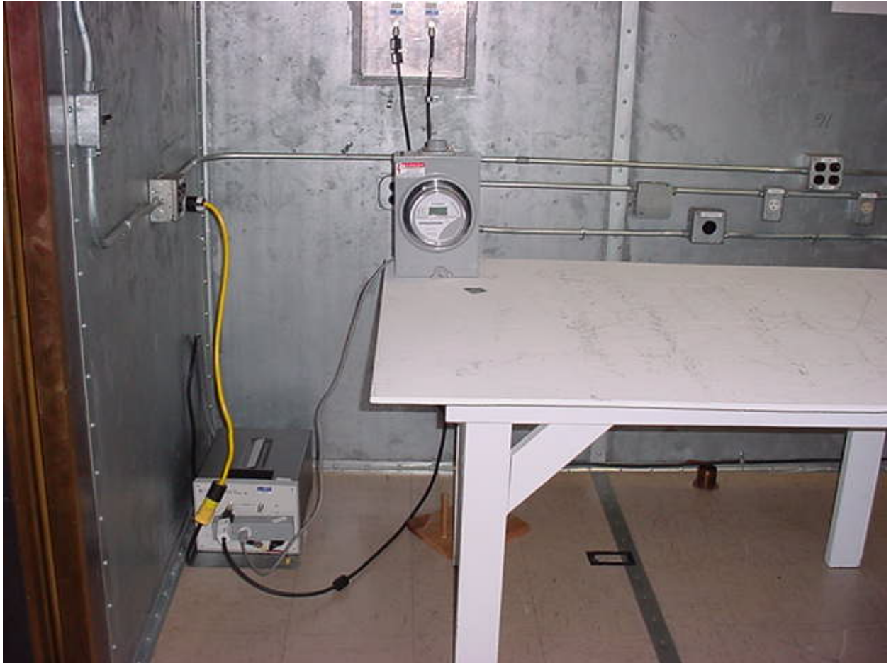
Figure 3: Conducted Emissions – Front View
