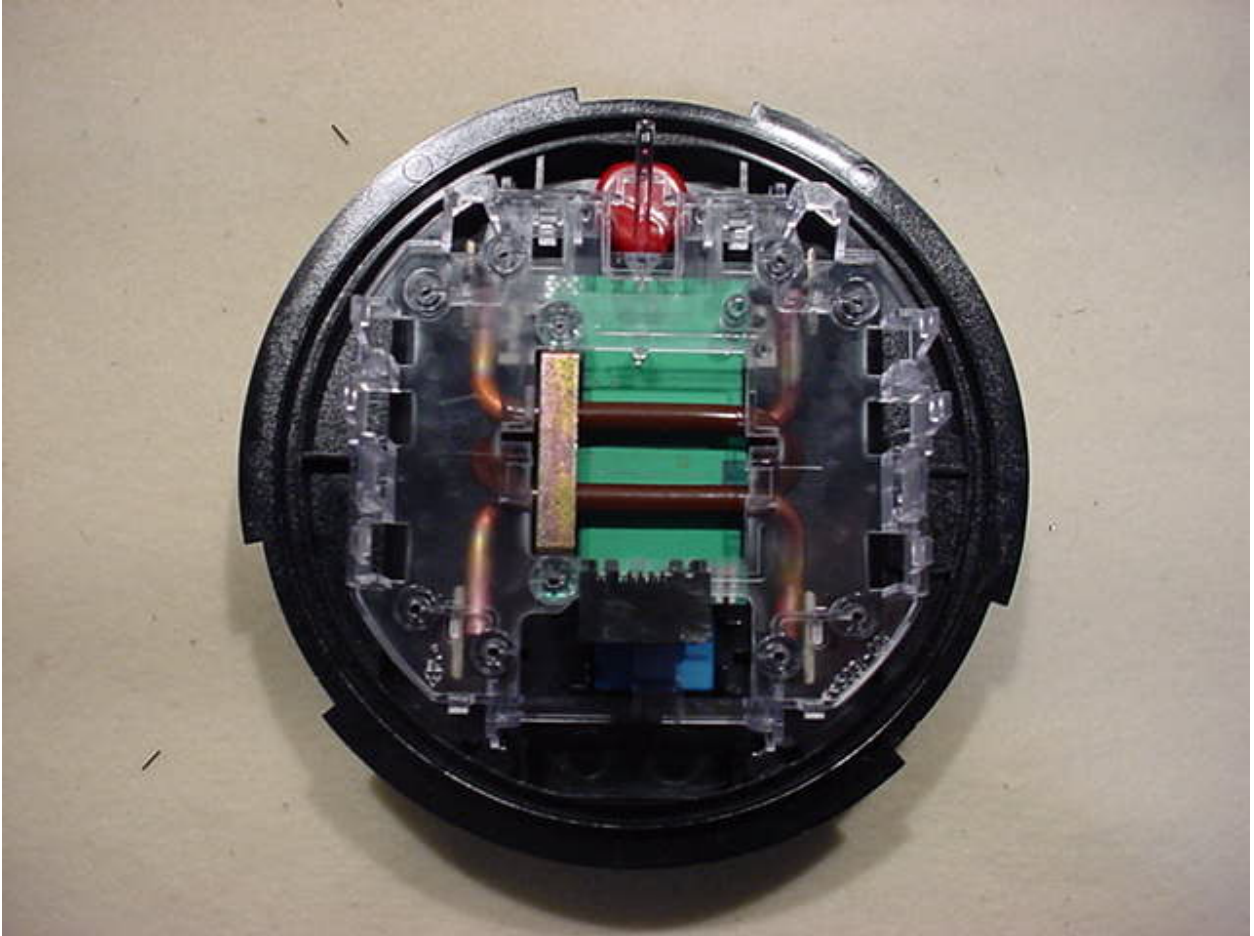
Figure 6: Housing Top View
